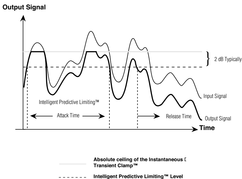
Figure 4: Protective Action of the PeakStopPlus™ Limiter
