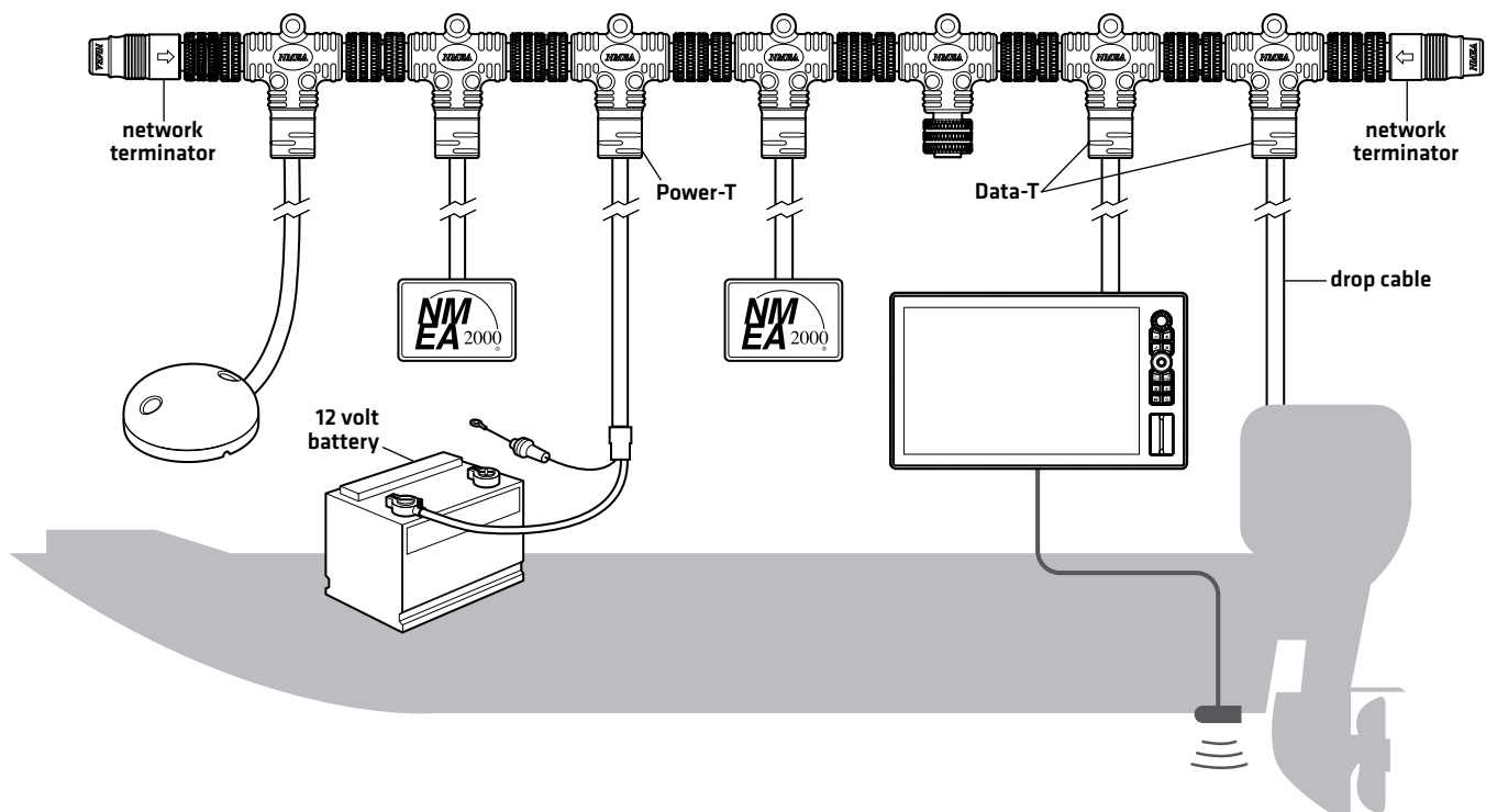
Sample NMEA 2000 Backbone
