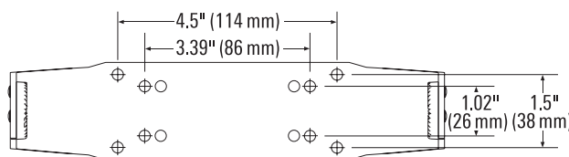
Bracket Hole Pattern Measurements
