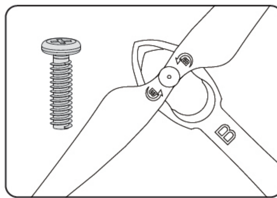
Propeller B
