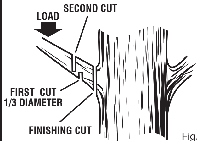
UNDERBUCKING
