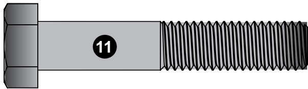
1/2-13 X 2-3/4" HEX BOLT 1B-6223-10 (QTY. 4)
