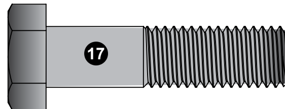
5/8-11x2-1/2" HEX BOLT 1B-7185-00 (QTY. 5)
