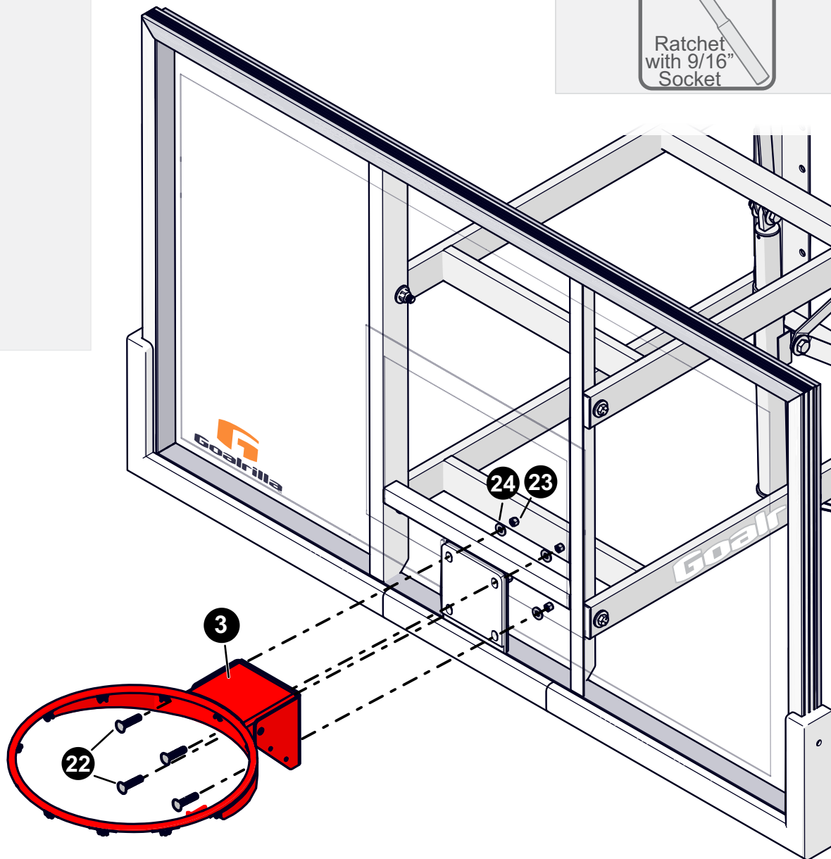
3/8-16 LOCKNUT 2B-6238-10 (QTY. 4)
