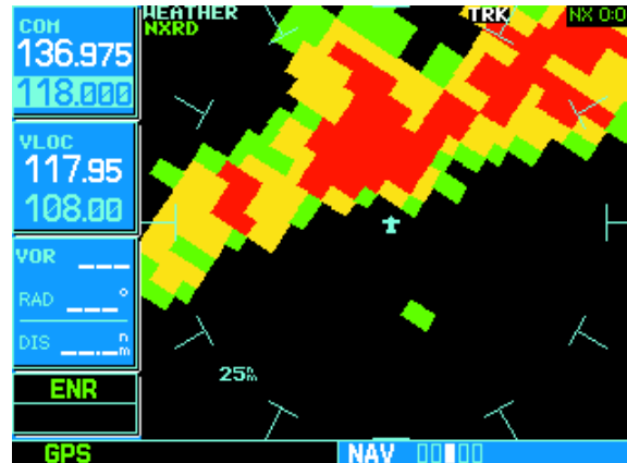
Figure 5-2 Weather Page
