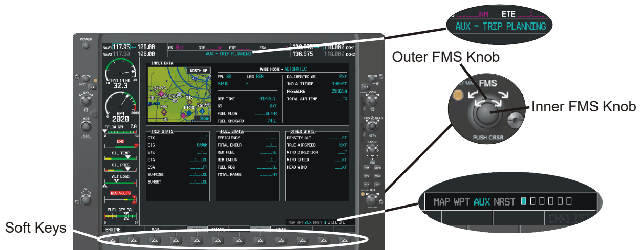
Figure 3-1 AUX Group
