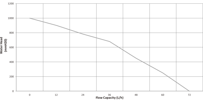
Pressure - Flow
