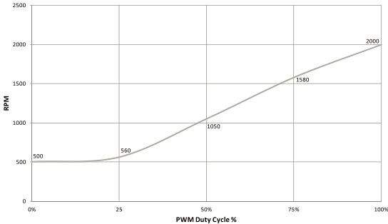
RPM - PWM Duty Cycle
