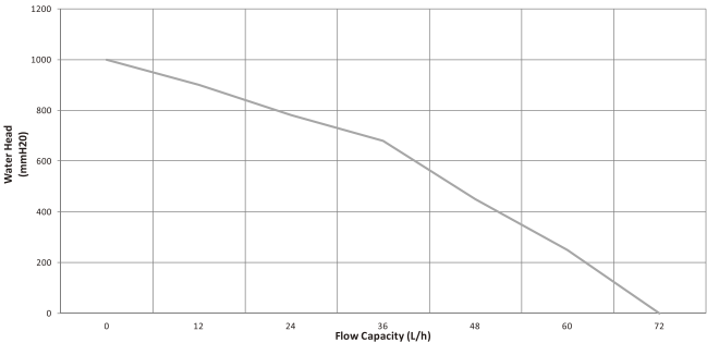
Pressure - Flow
