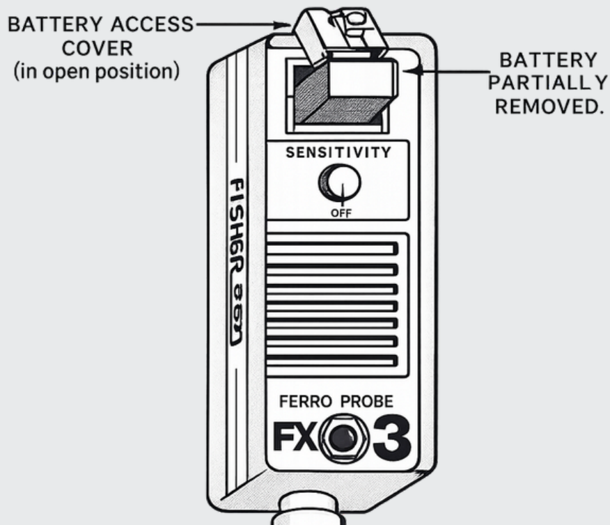
Figure 8. Battery Placement
