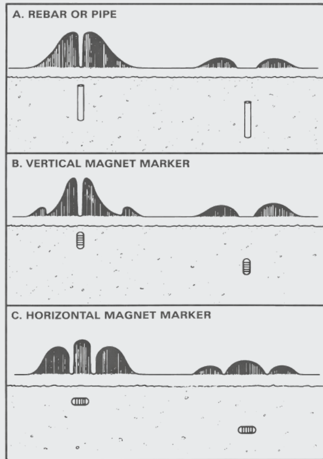
Figure 4. Locating Property Markers – Typical FX-3 responses at medium sensitivity and moderate sweep speed for shallow and deep targets.
