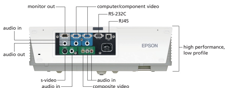
Back View
