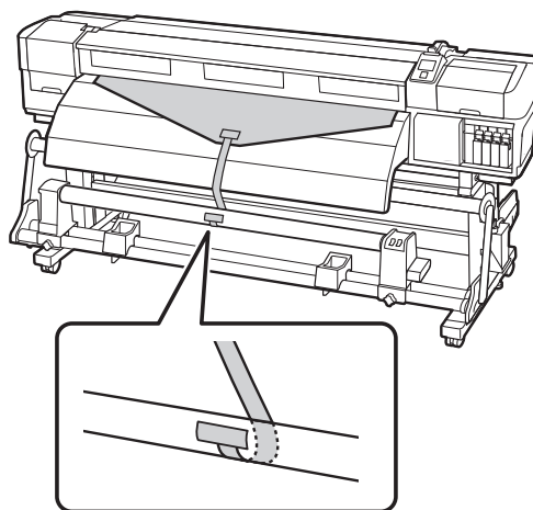
Printed side in
