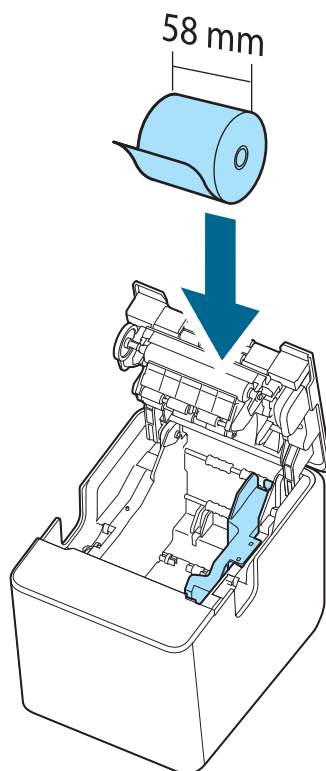
Attach 58-mm width roll paper guide to the right (Default)
