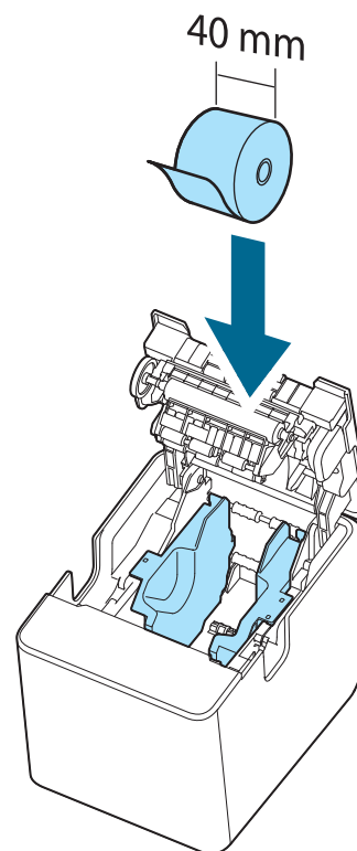
Attach 58-mm width roll paper guide to the right Attach 40-mm width roll paper guide to the left
