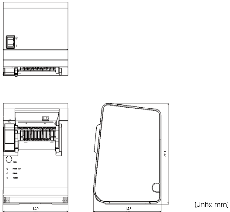
External Appearance (TM-L90 Peeler Model)
