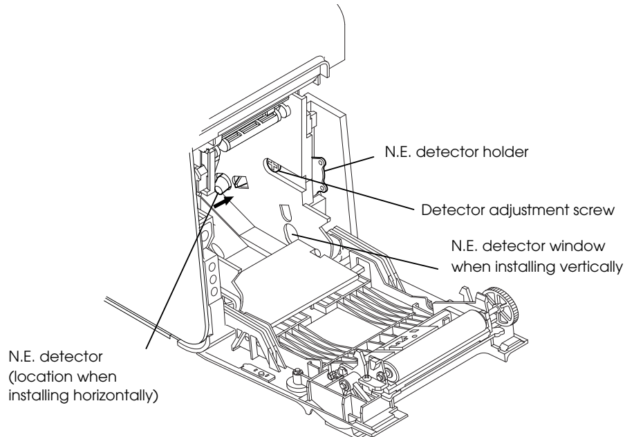
Part names and the locations of N.E. detector components
