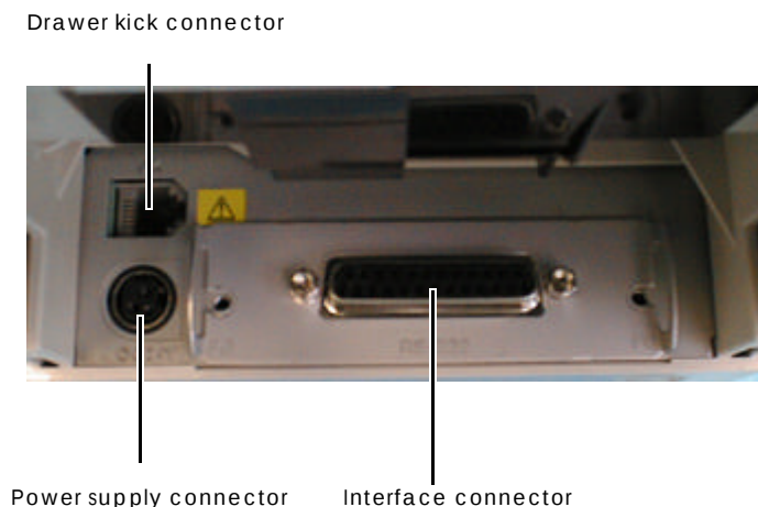
Connector Panel
