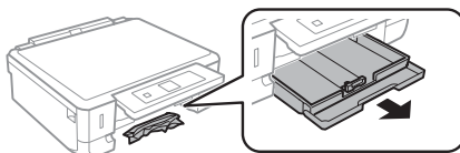
Paper cassette
