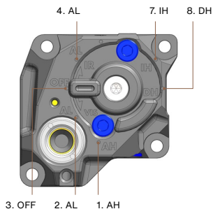
FIGURE 3.7 Modes of Operation (Rear View)
