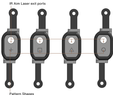
FIGURE 3.15 Pattern Generators
