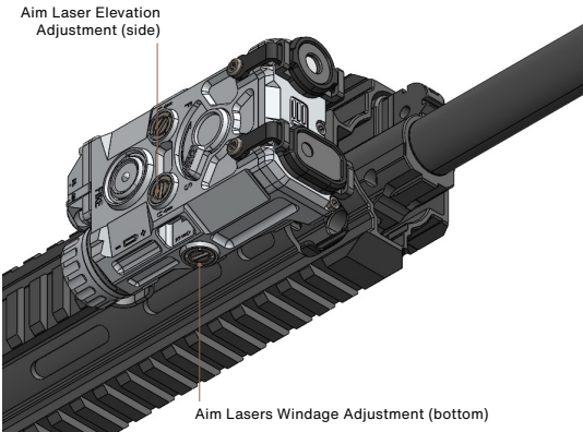
FIGURE 3.22 Aim Laser Adjusters (right side mounted)
