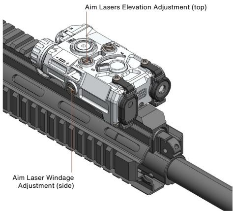
FIGURE 3.20 Aim Laser Adjusters (top mounted)
