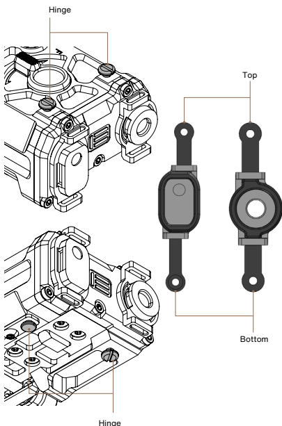
FIGURE 4.2 OGL C Assembly
