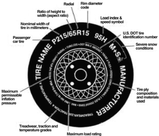
Figure 3: Typical Passenger Tire Markings
