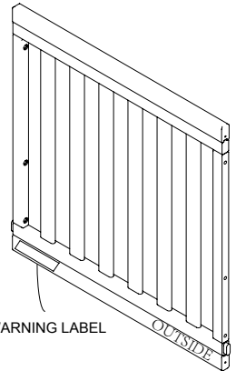
C. Right Crib End x 1 Part #24676
