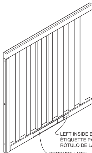
F. Front Rail x 1 Panneau avant x 1 Barandilla frontal x 1 25841
