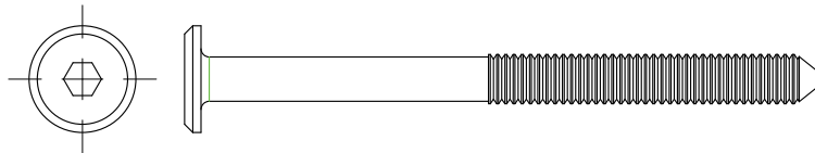
DD. 75mm Bolt x2 Boulon 75mm Perno 75mm
