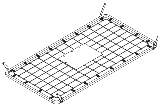
G. Mattress Support x 1 Support du matelas x 1 Soporte del Colchón x 1 24242
