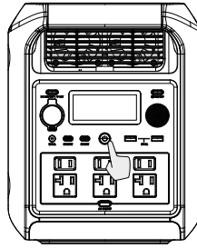
Short Press to Turn On/Long Press to Turn Off
