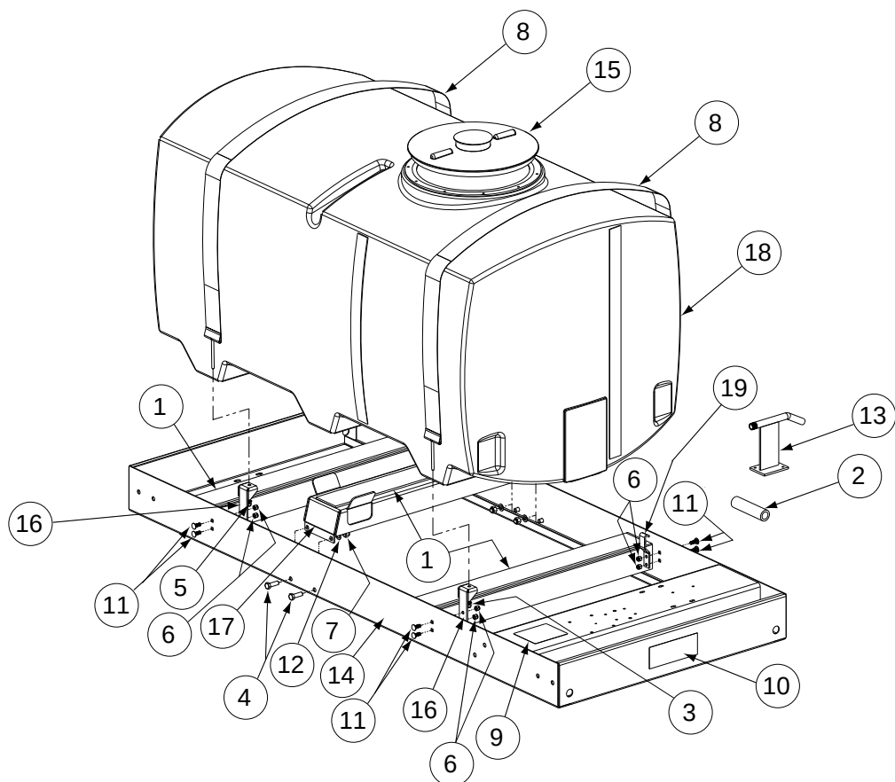
300 Gallon Gasoline-Powered Polyethylene Tank Sprayers No. 02004706
