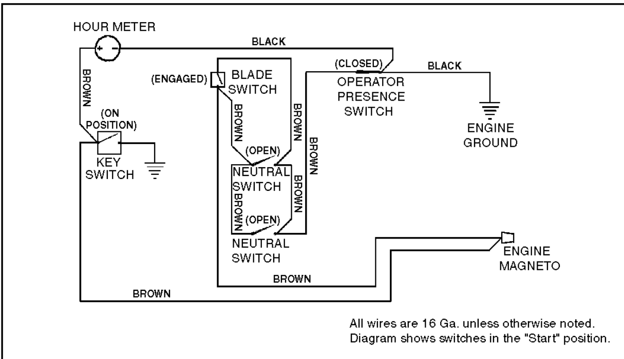
15HPElectrical Diagram - Figure 26
