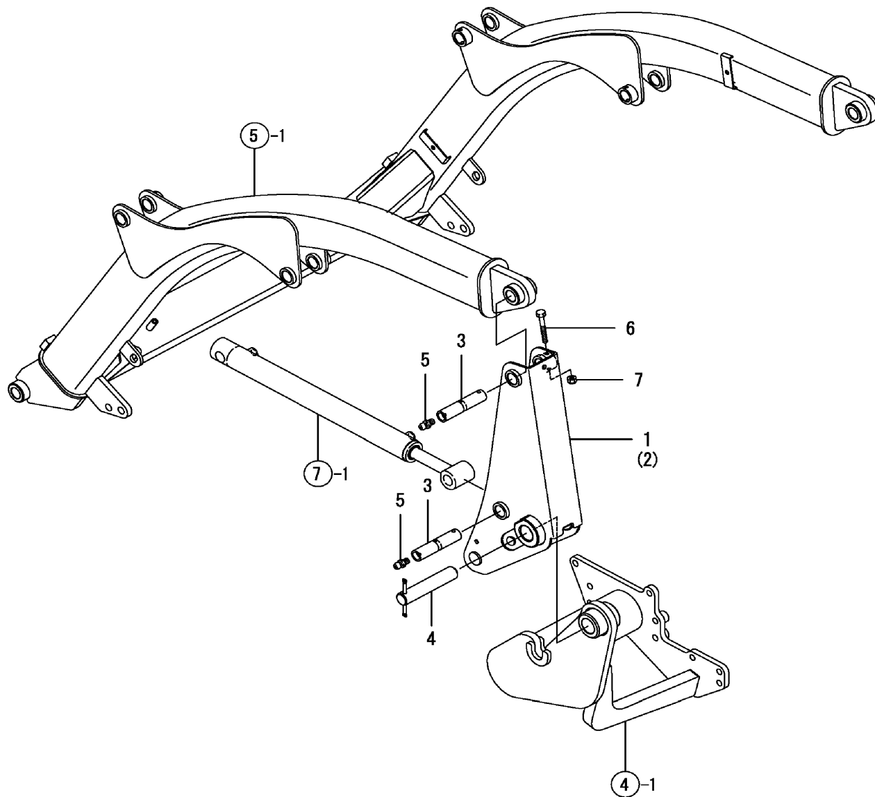
FIG. 3. SUPPORT FRAME
