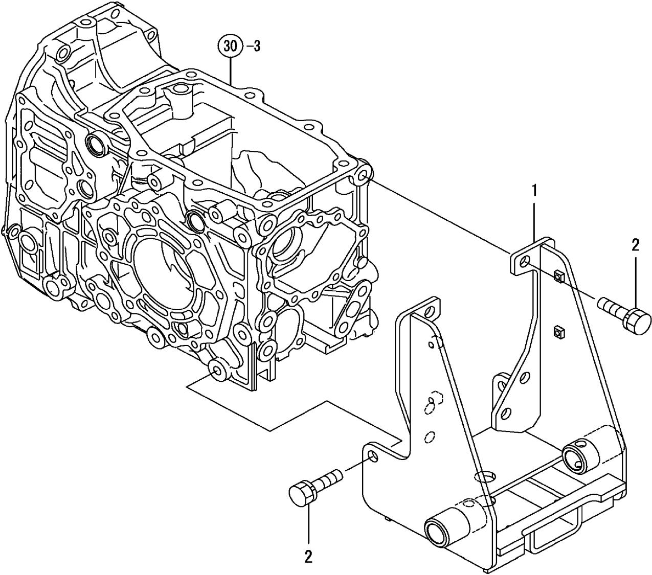
FIG. 96. REAR HITCH
