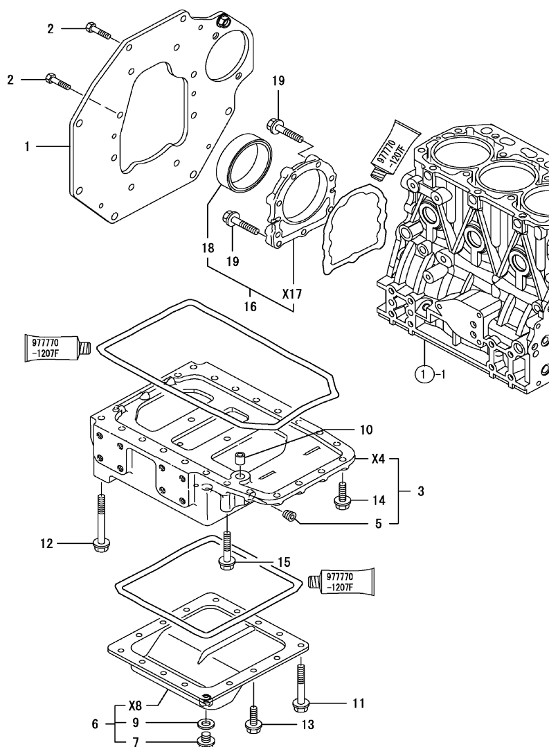
FIG. 3. MOUNTING FLANGE &amp; OIL SUMP
