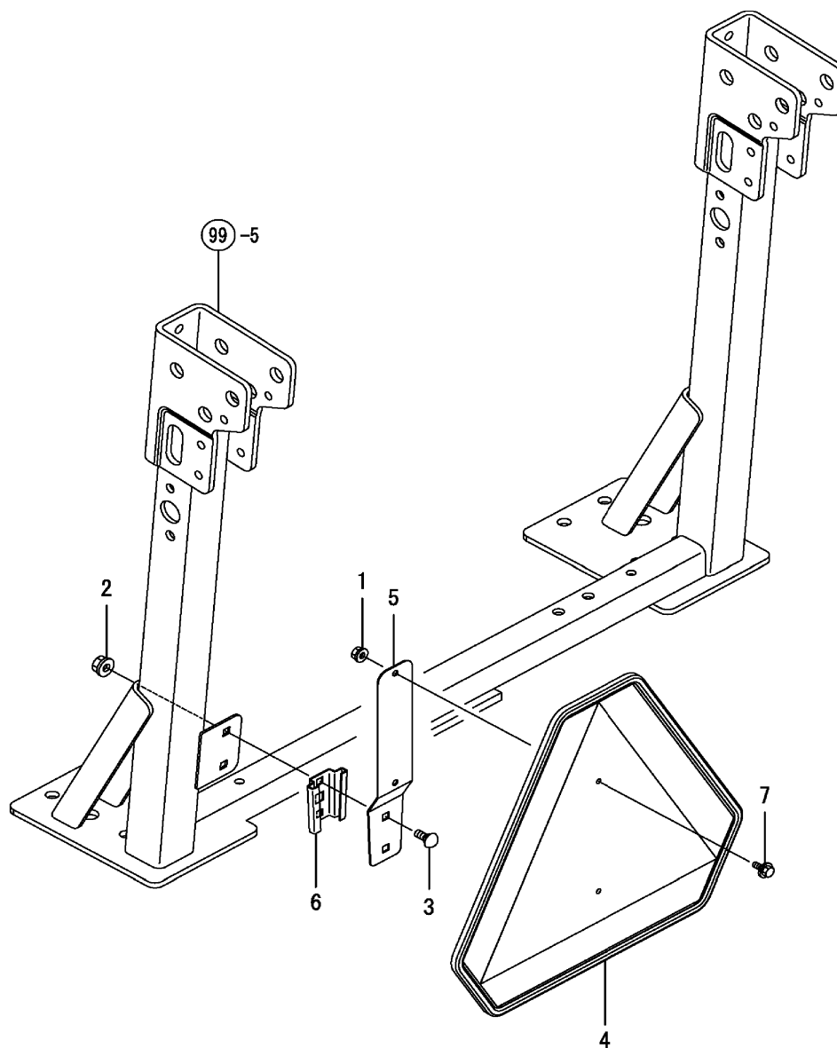
FIG. 100. SMV
