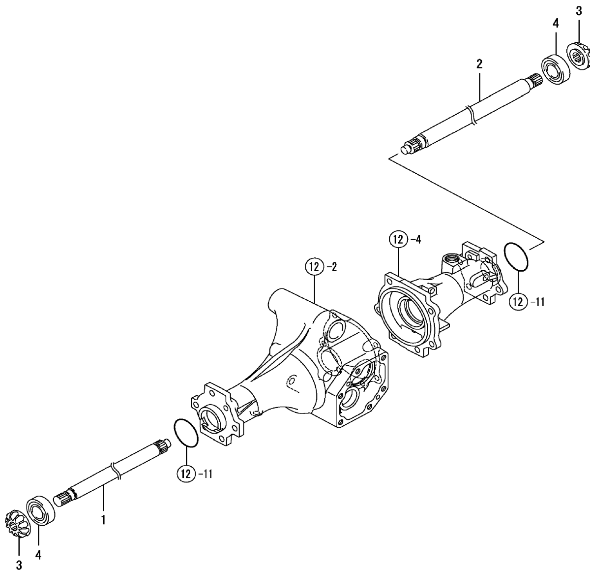
FIG. 11. FRONT SHAFT 1
