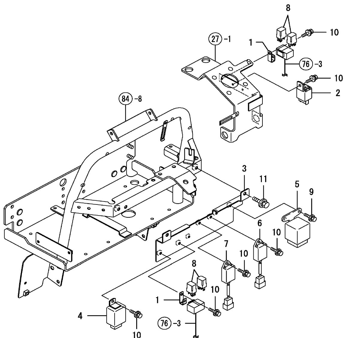
FIG. 82. RELAY
