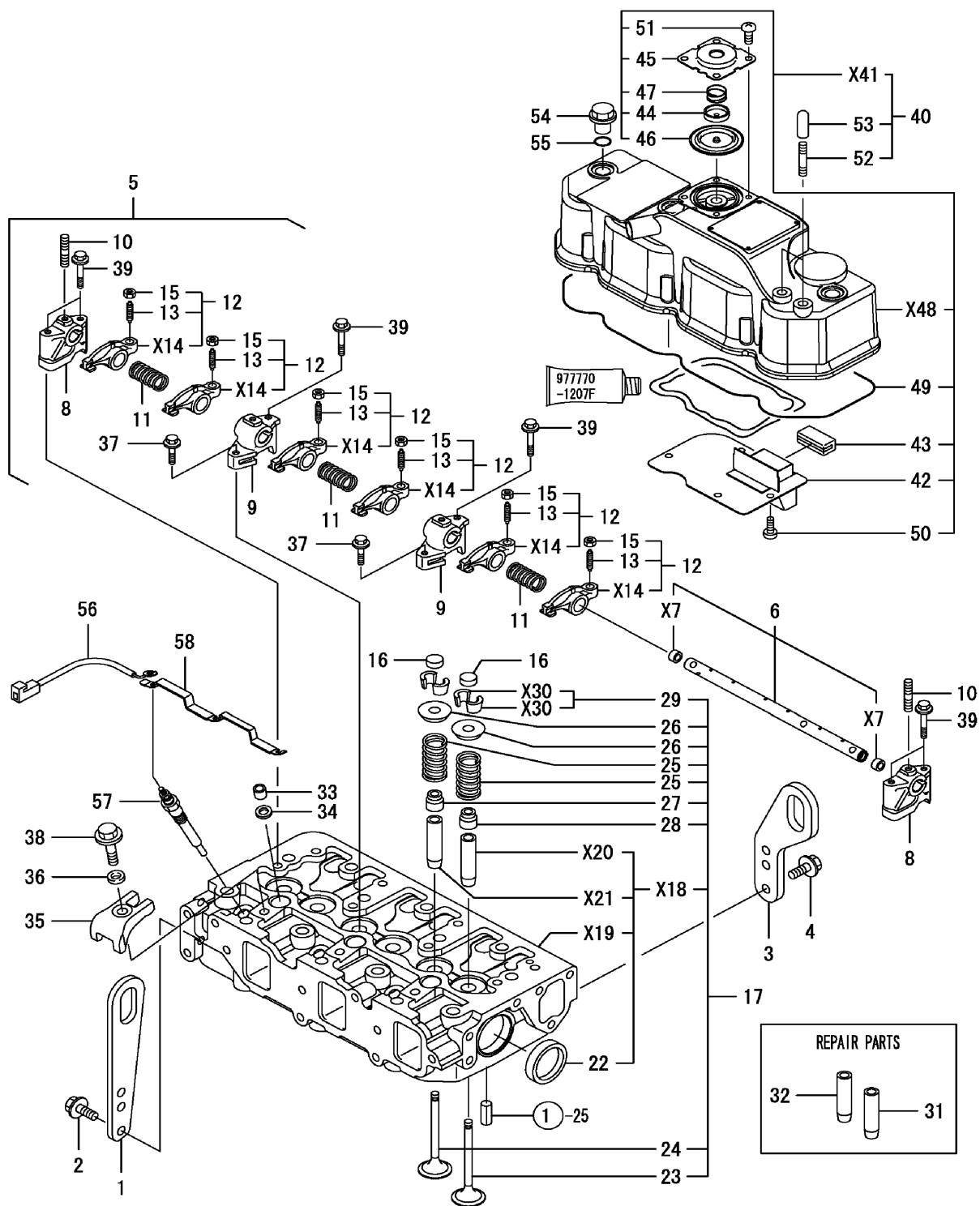
FIG. 4. CYLINDER HEAD &amp; BONNET
