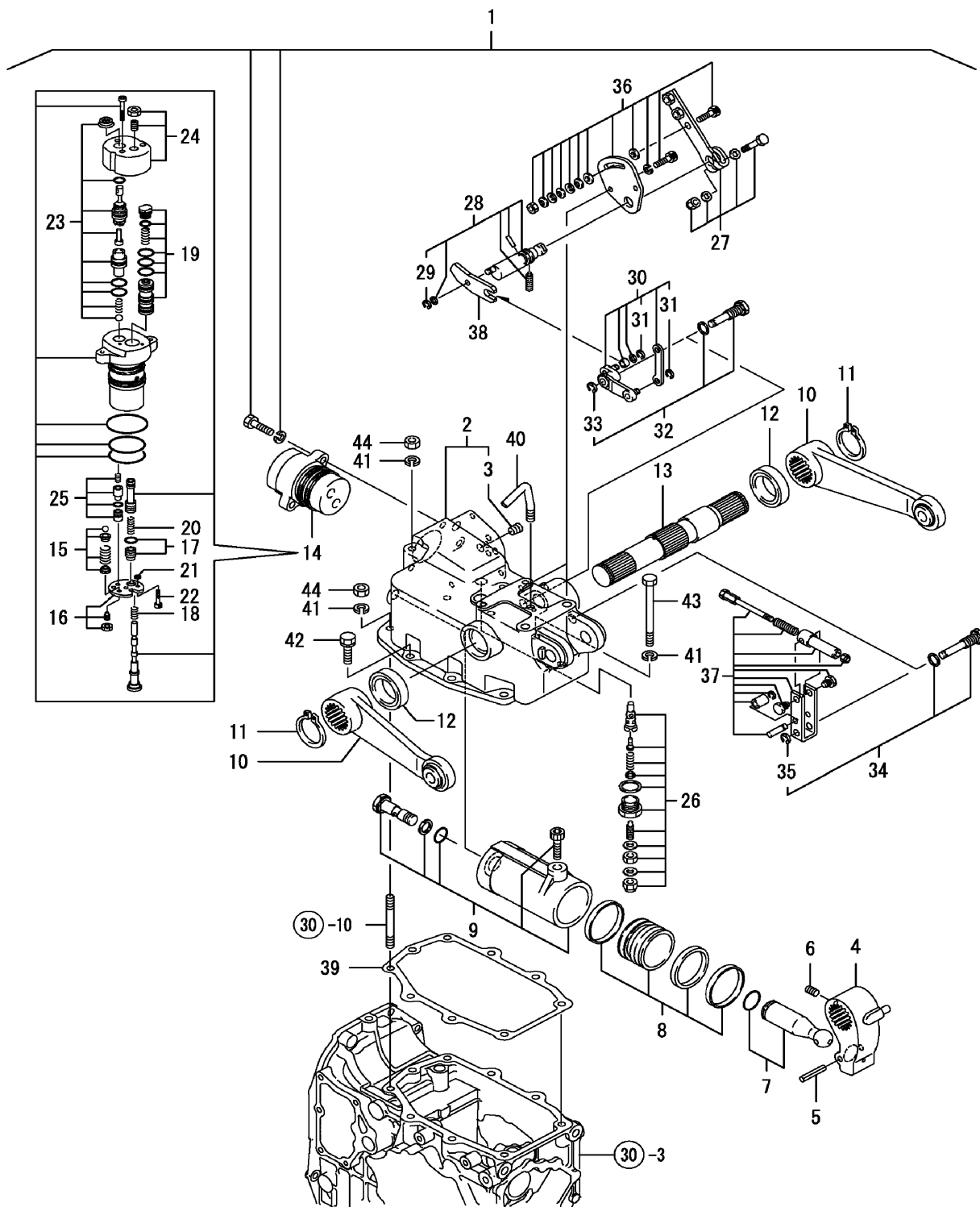
FIG. 70. HYDRAULIC LIFT
