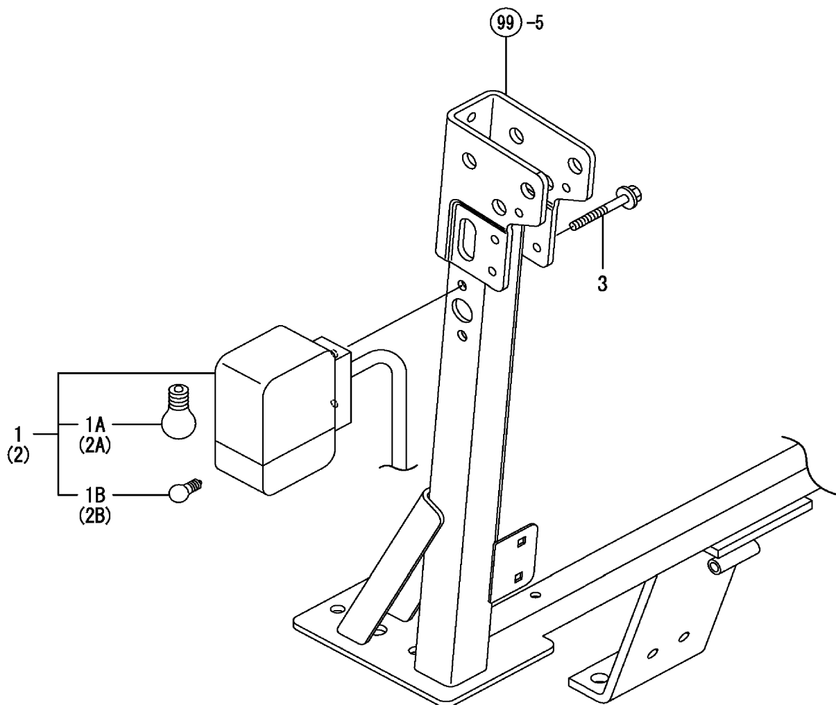
FIG. 80. LAMPS
