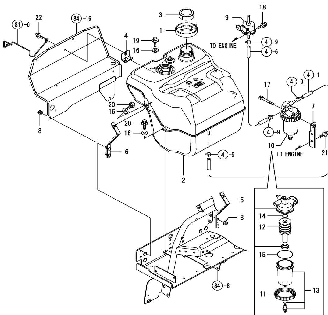
FIG. 3. TANK, FUEL
