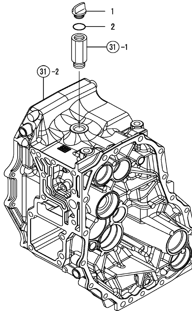
FIG. 32. OIL CAP
