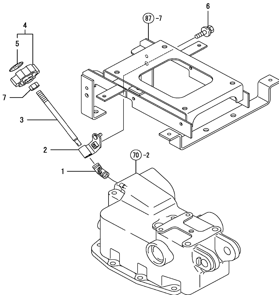
FIG. 72. STOP VALVE
