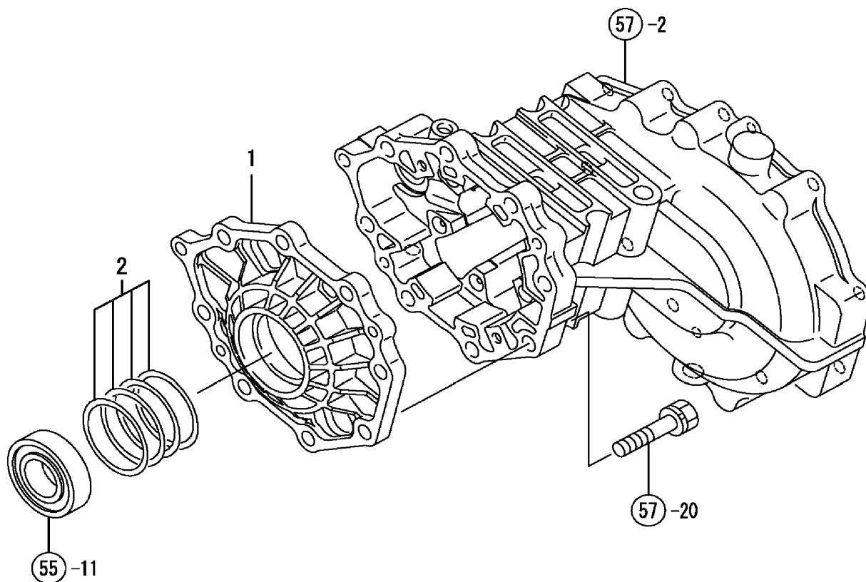
FIG. 56. DIFFERENTIAL CARRIER
