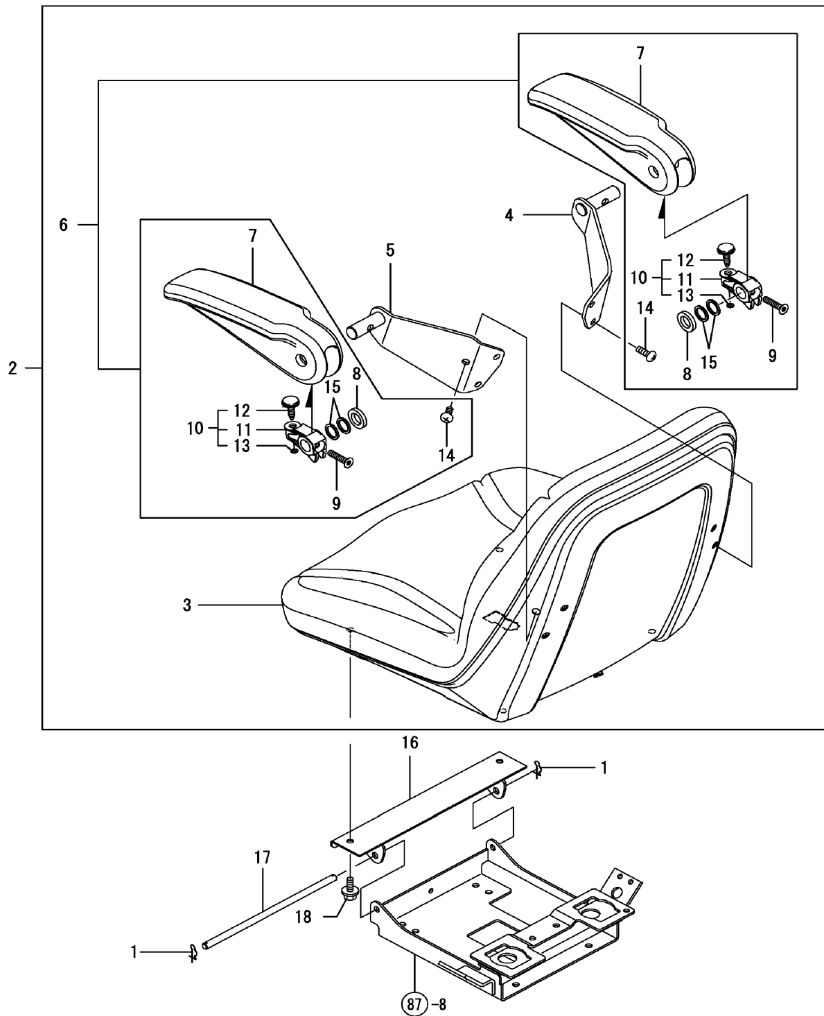
FIG. 88. DRIVER SEAT
