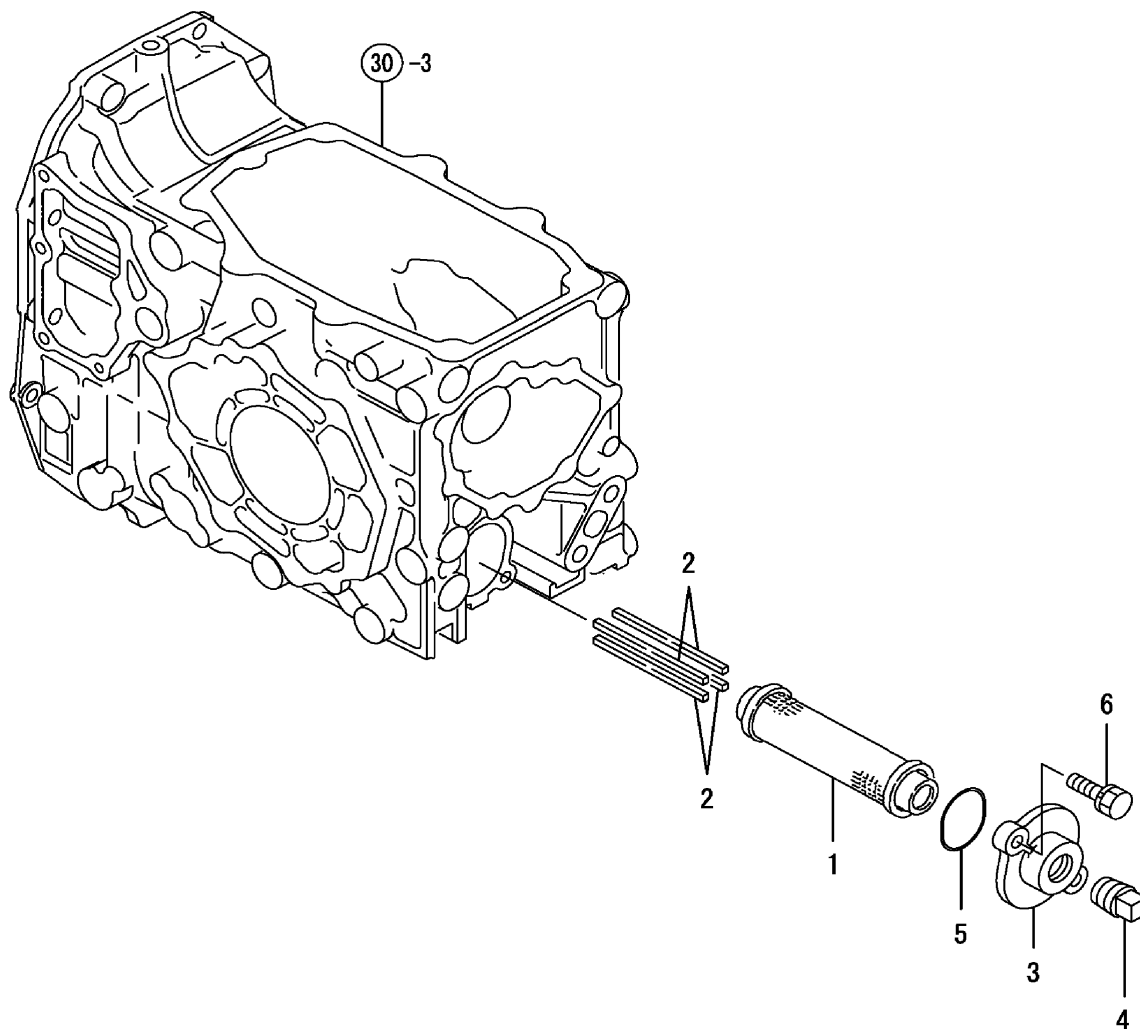
FIG. 33. OIL STRAINER
