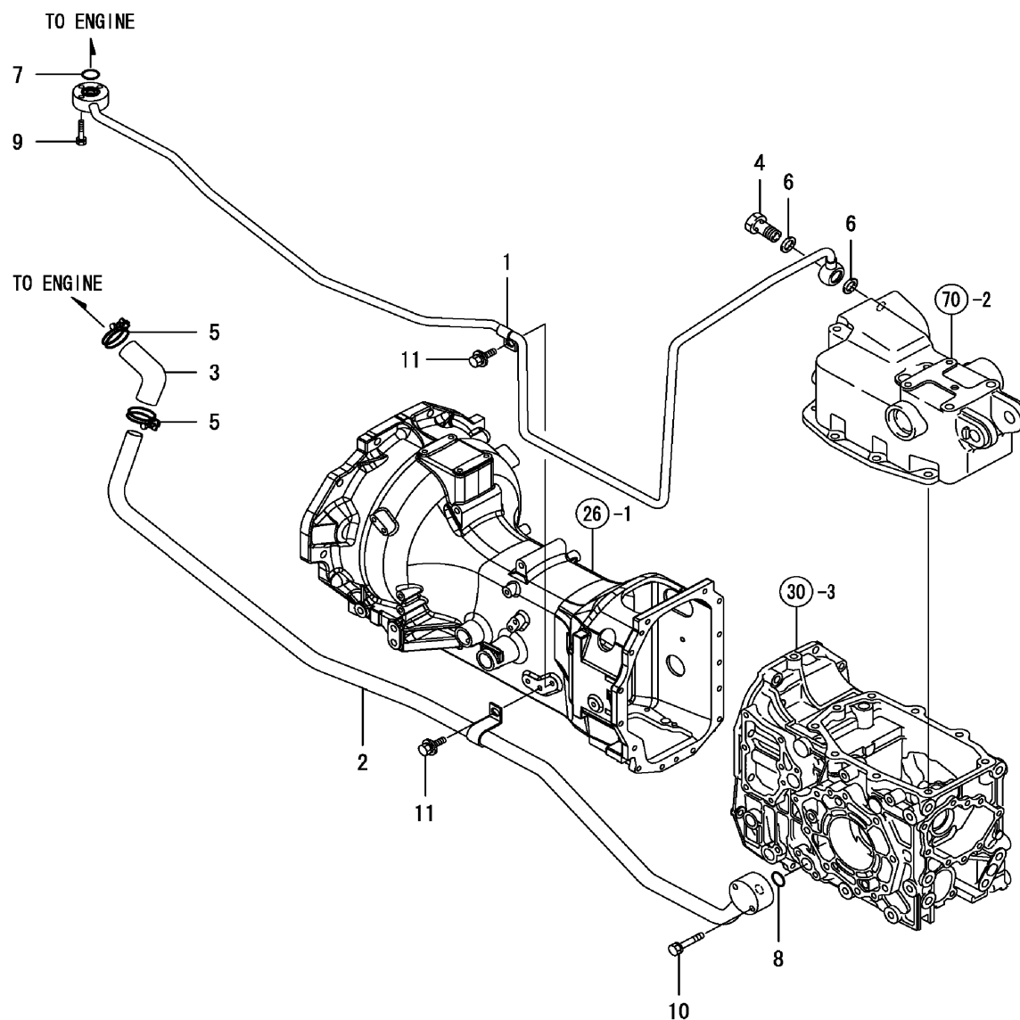
FIG. 75. HYDRAULIC LINE
