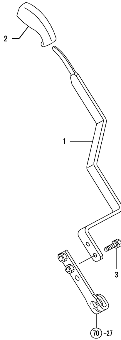
FIG. 71. HYDRAULIC CONTROL
