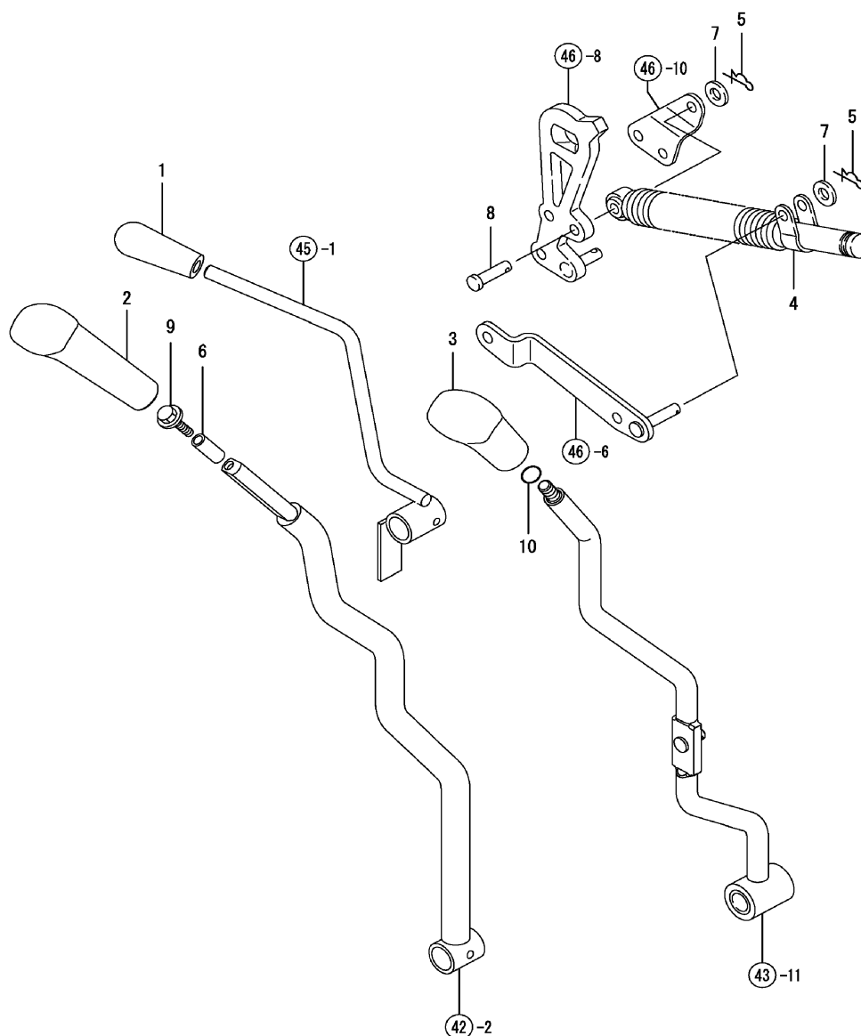
FIG. 47. HST CONTROL 2
