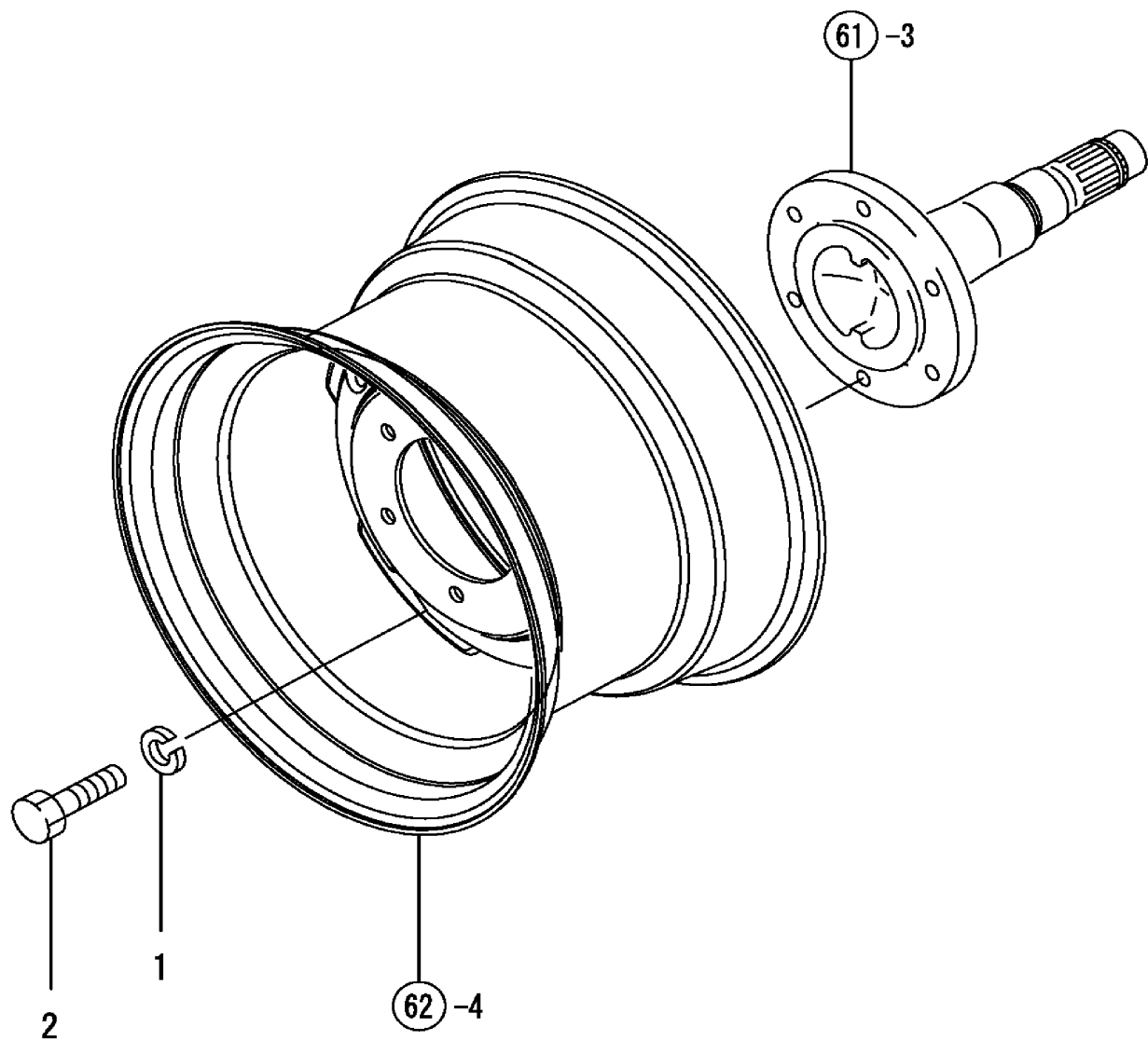
FIG. 64. REAR HUB BOLT
