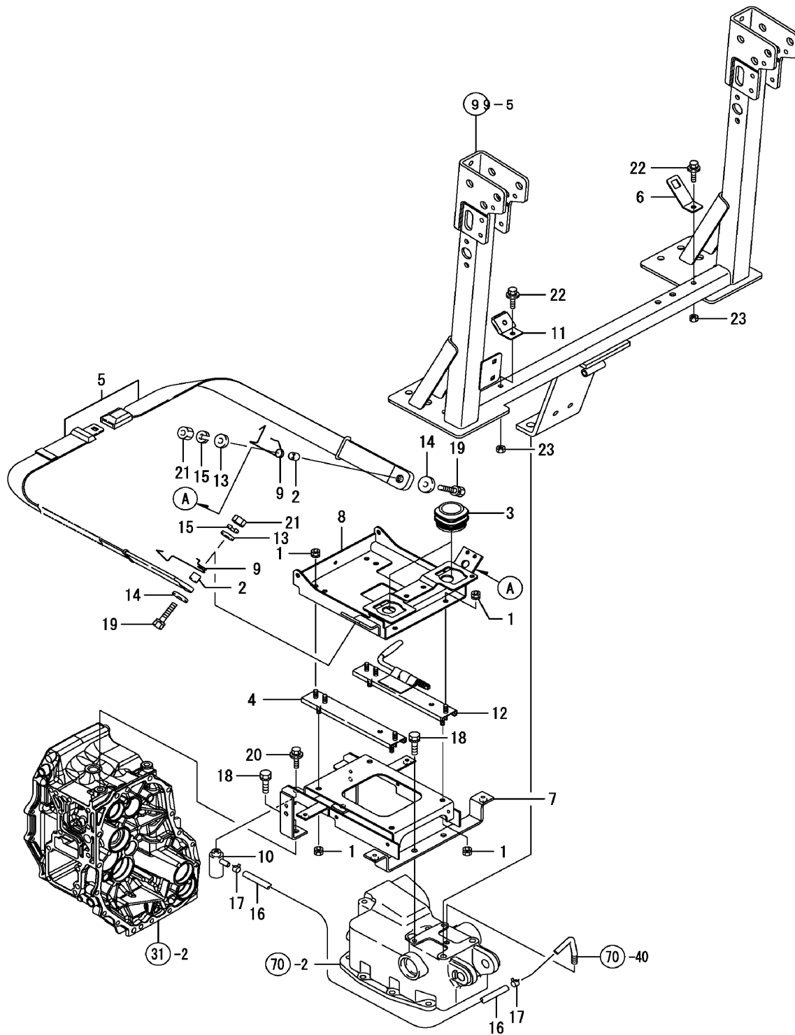
FIG. 87. SEAT BRACKET
