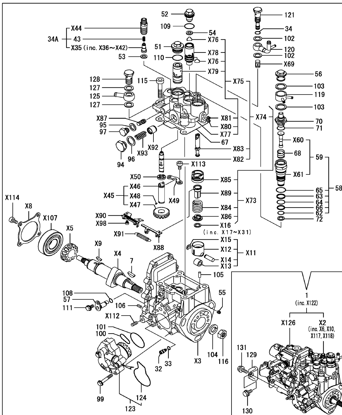
FIG. 12. FUEL INJECTION PUMP
