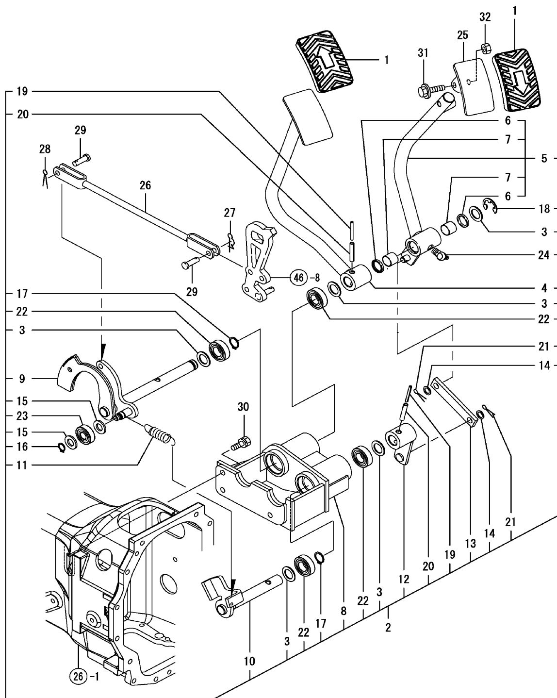
FIG.65. HYDRAULIC PEDAL
