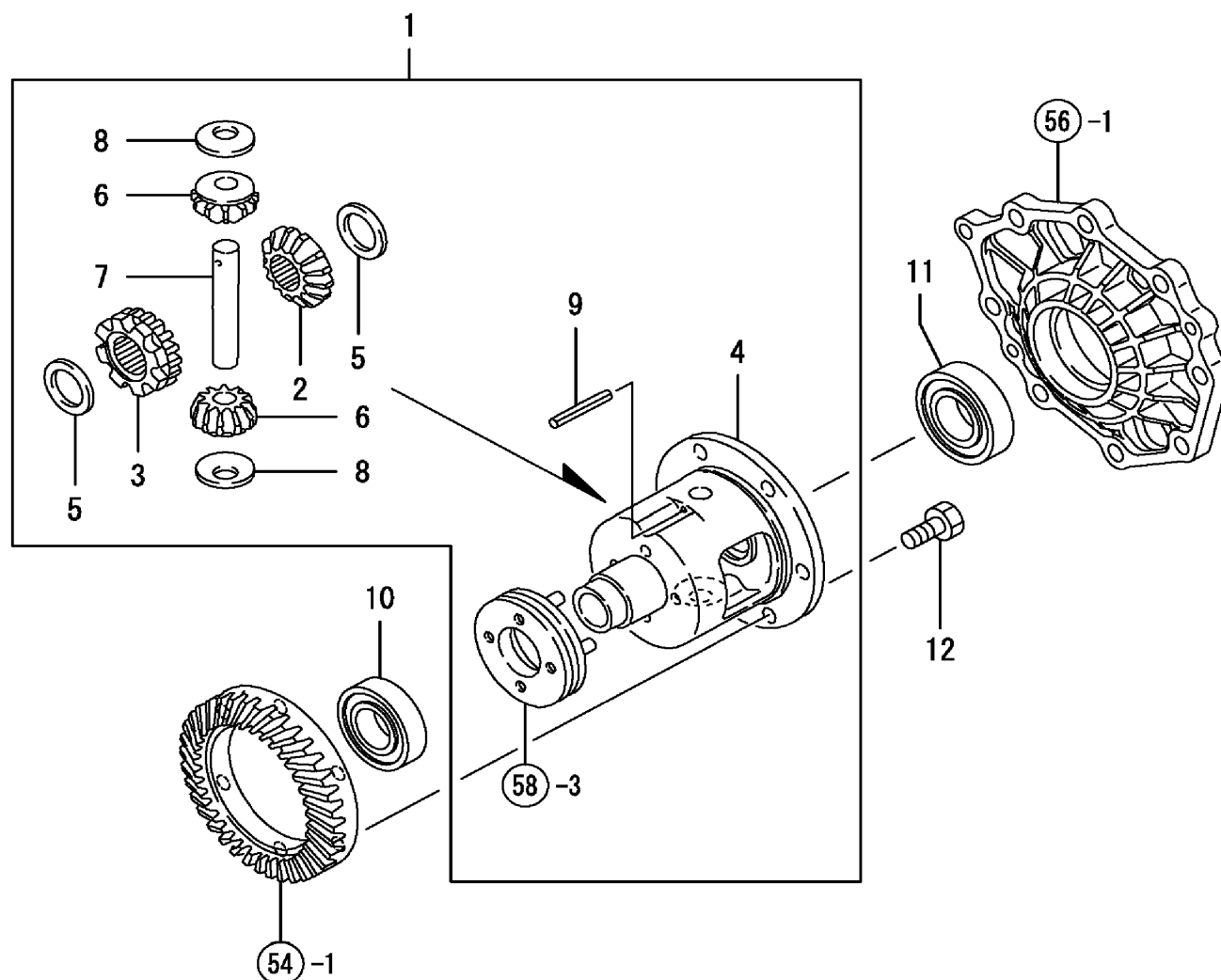
FIG. 55. DIFFERENTIAL GEAR
