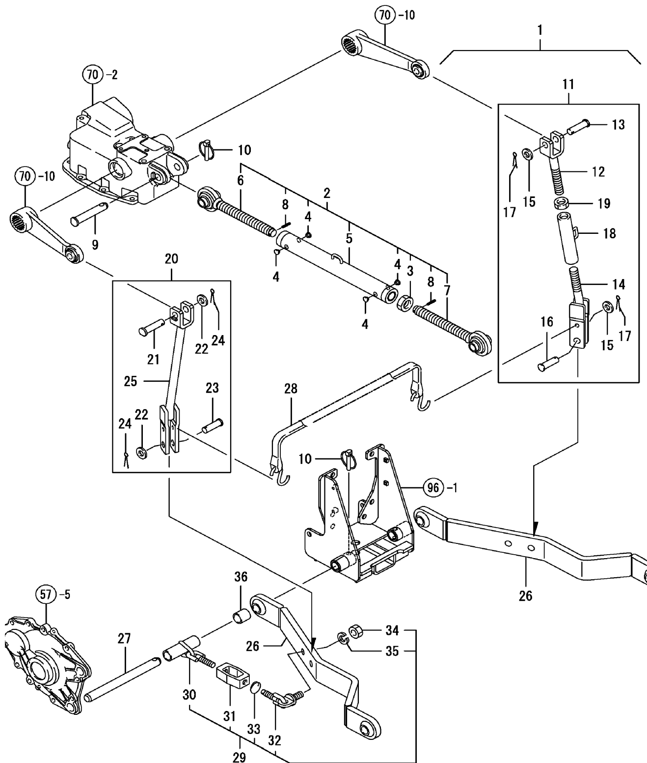
FIG. 95. 3-POINT HITCH
