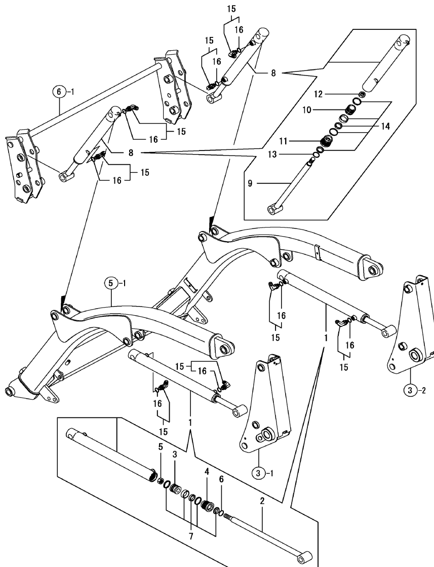
FIG. 7. CYLINDER
