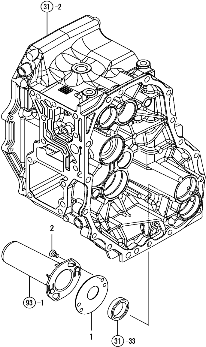
FIG. 94. OIL SEAL COVER
