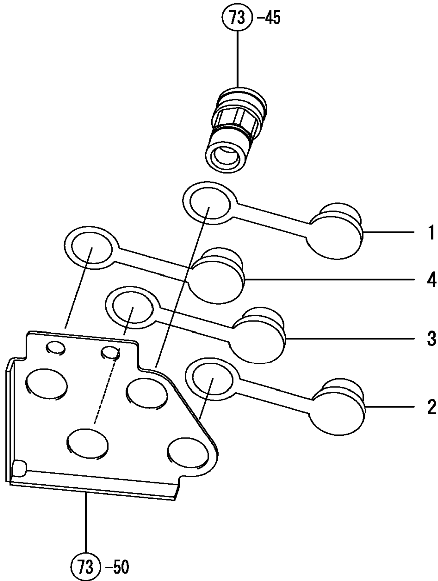
FIG. 74. VALVE ACCESSORIES
