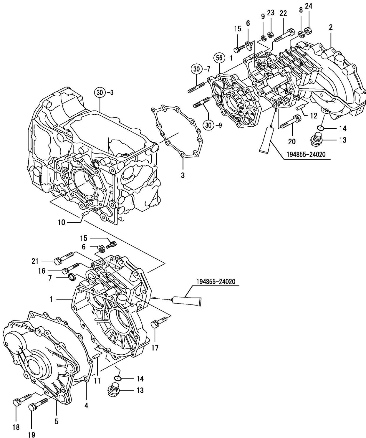
FIG. 57. REAR HOUSING
