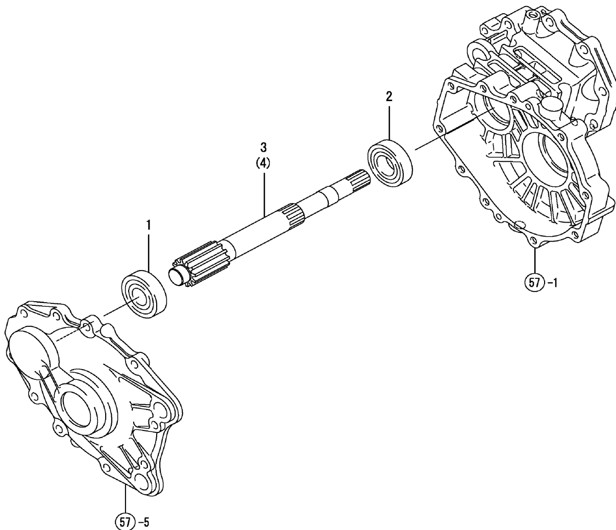
FIG. 59. FINAL PINION
