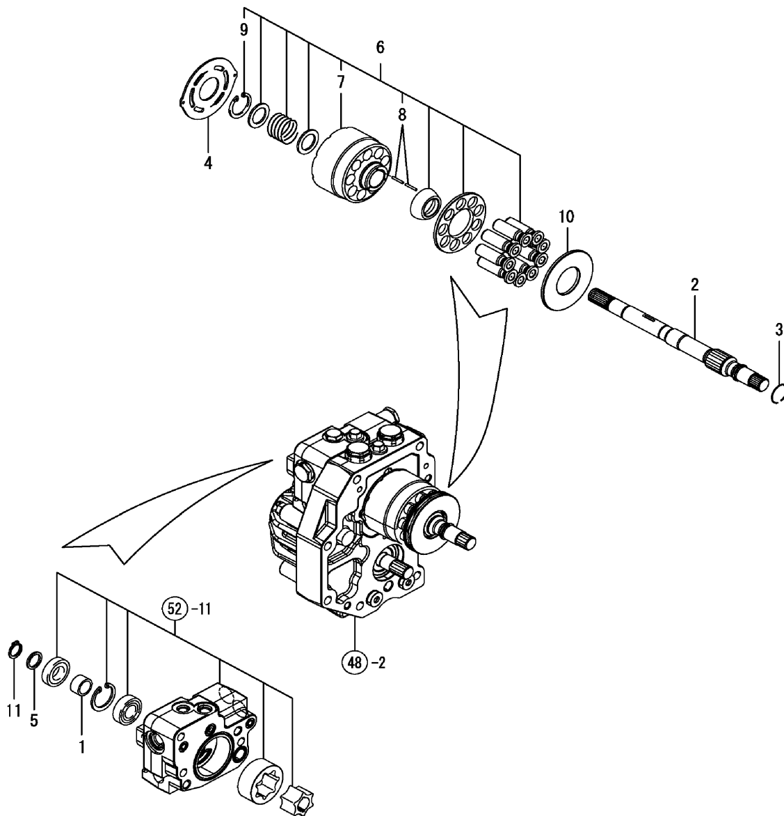
FIG. 50. PUMP
