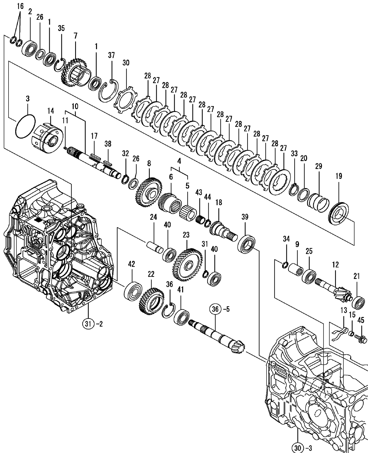
FIG. 38. PTO CLUTCH SHAFT
