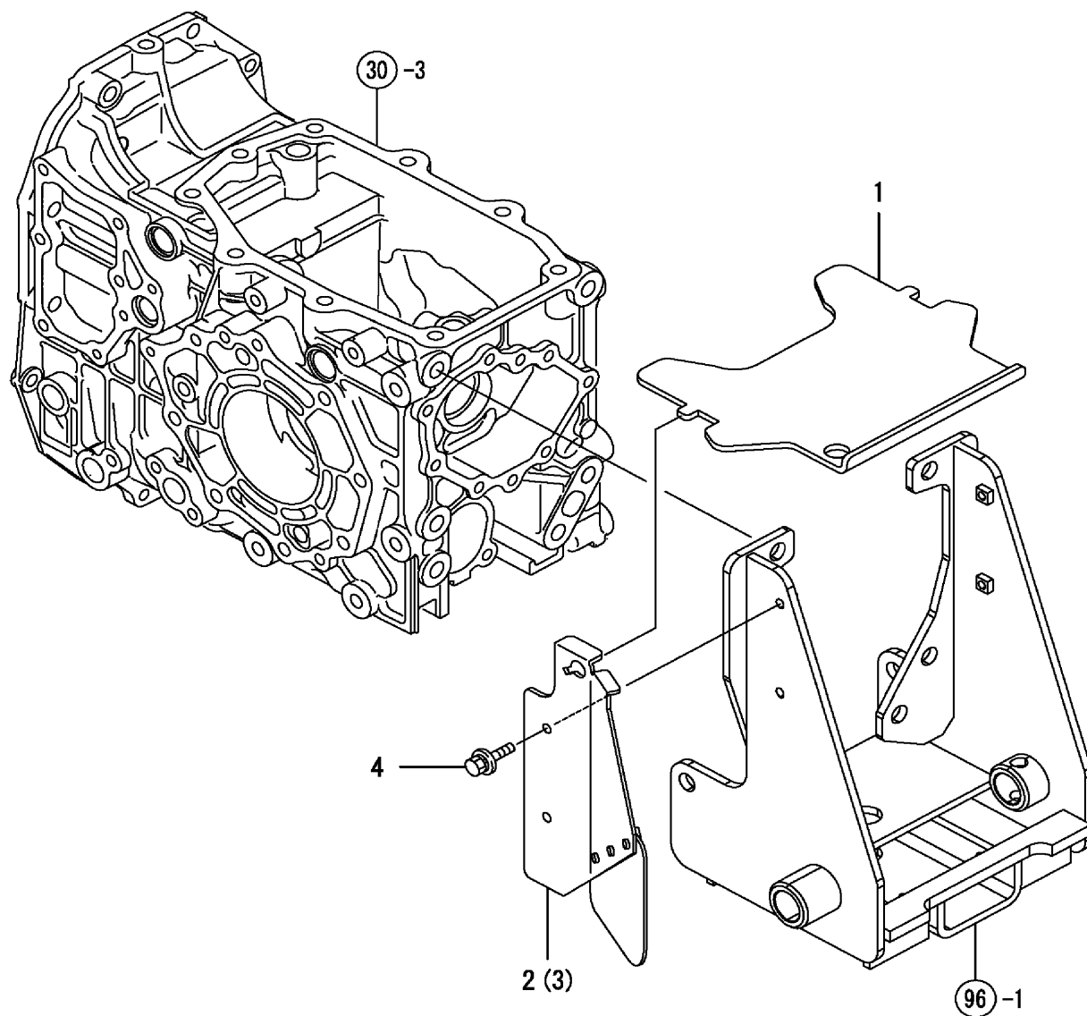
FIG. 92. PTO GUARD
