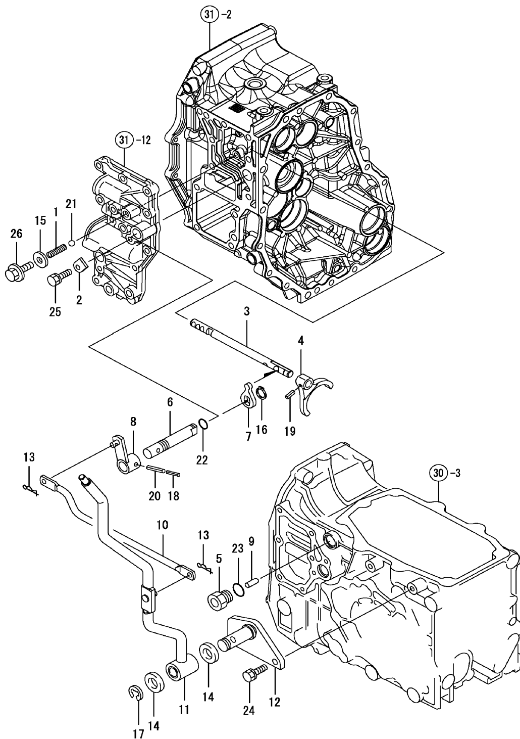
FIG. 43. PTO CHANGE
