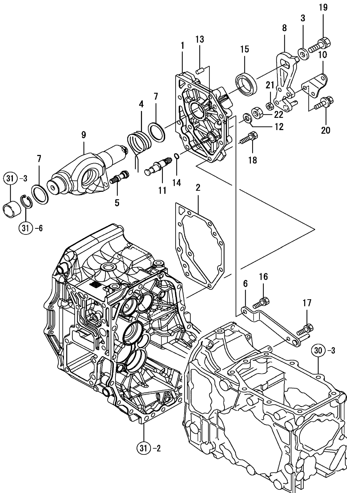
FIG. 46. HST CONTROL 1
