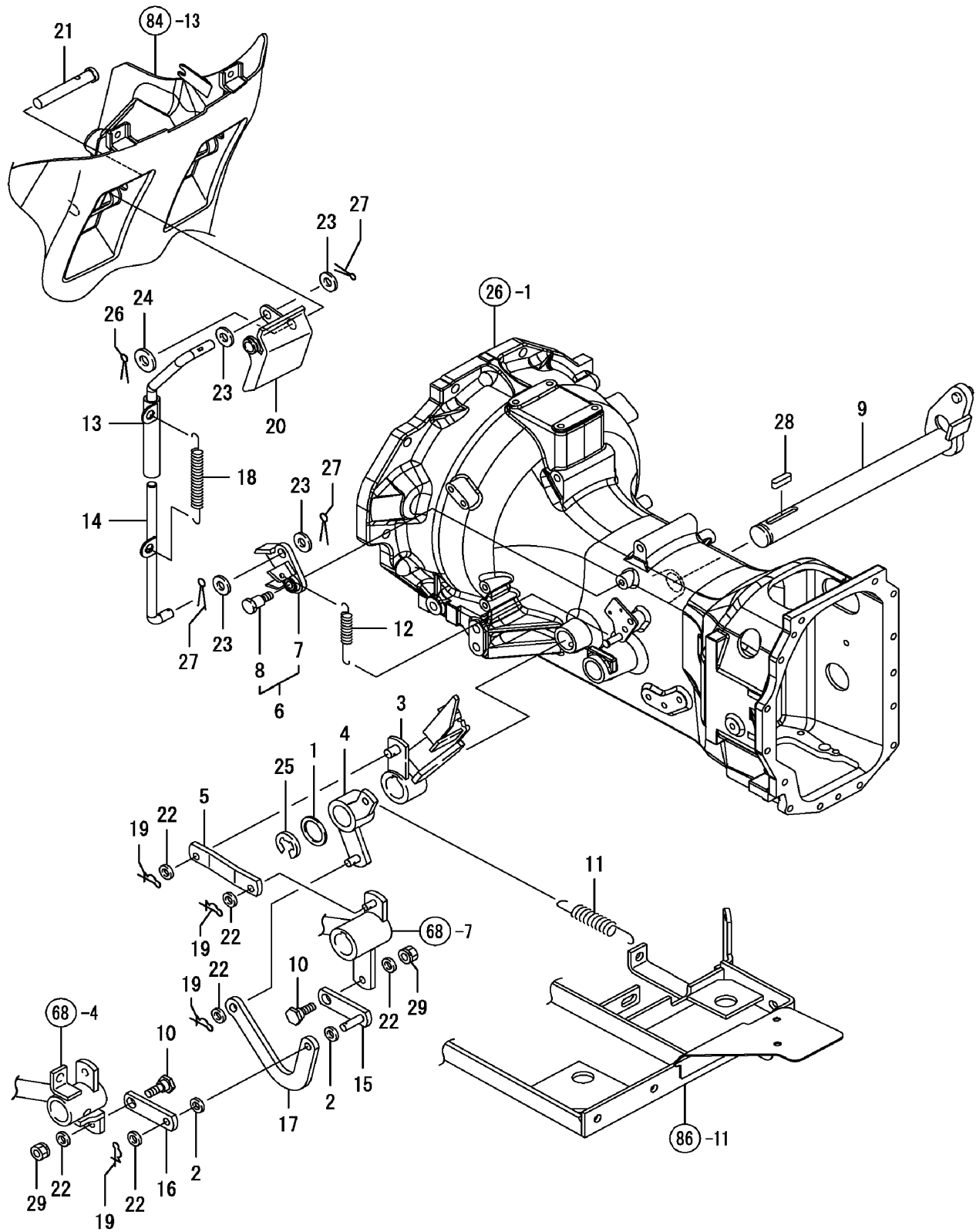
FIG. 69. PARKING BRAKE
