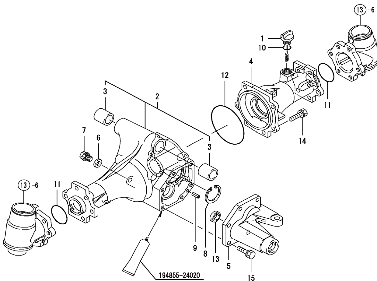
FIG. 12. FRONT AXLE HOUSING
