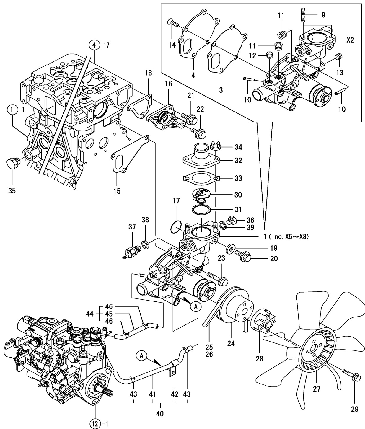
FIG. 11. COOLING WATER SYSTEM
