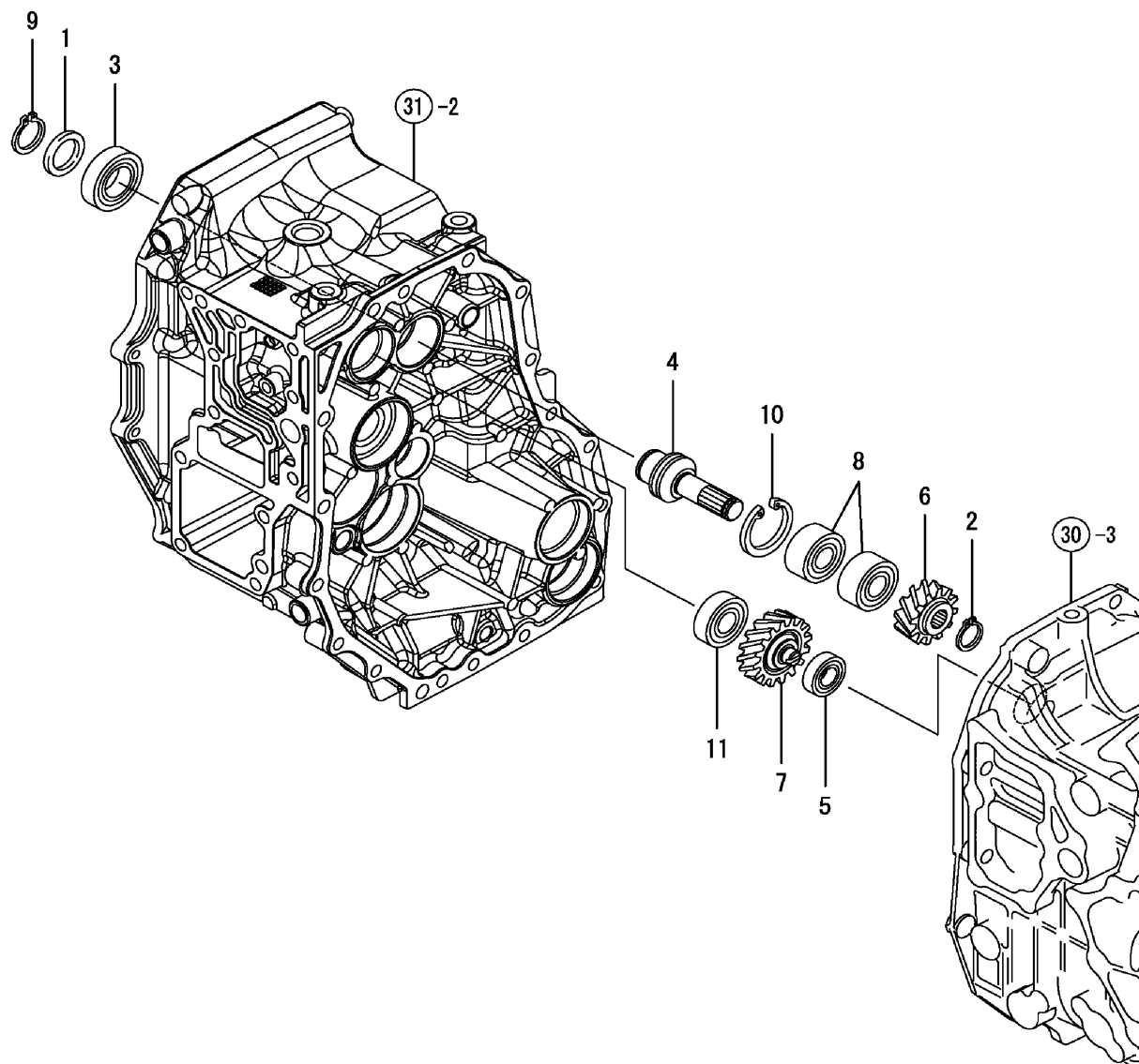
FIG. 37. PTO DRIVE SHAFT
