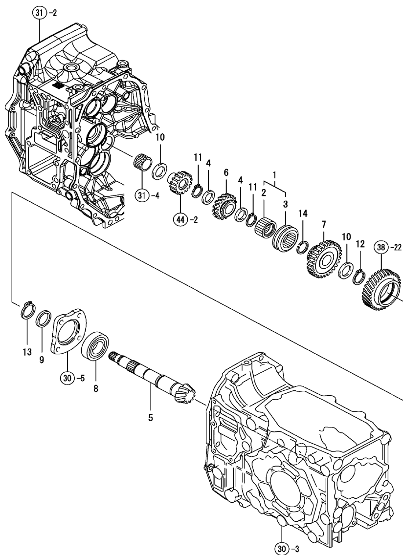
FIG. 36. COUNTER SHAFT
