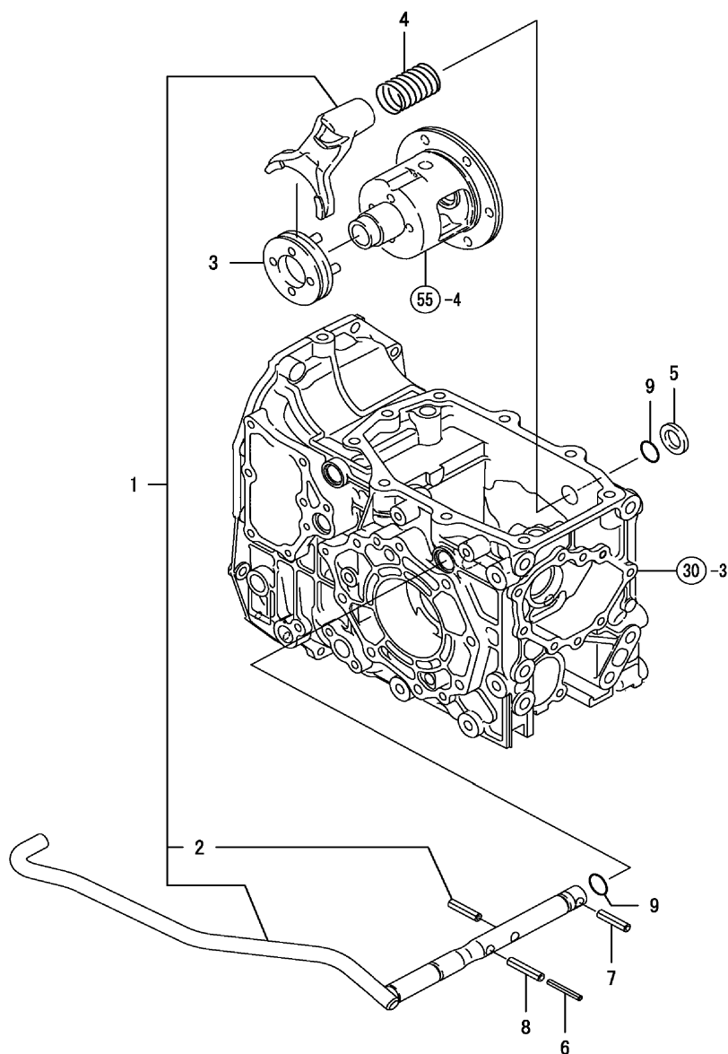
FIG. 58. DIFFERENTIAL LOCK
