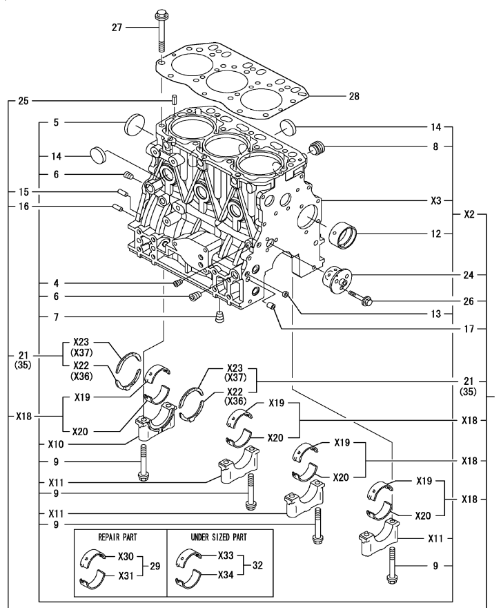
FIG. 1 CYLINDER BLOCK
