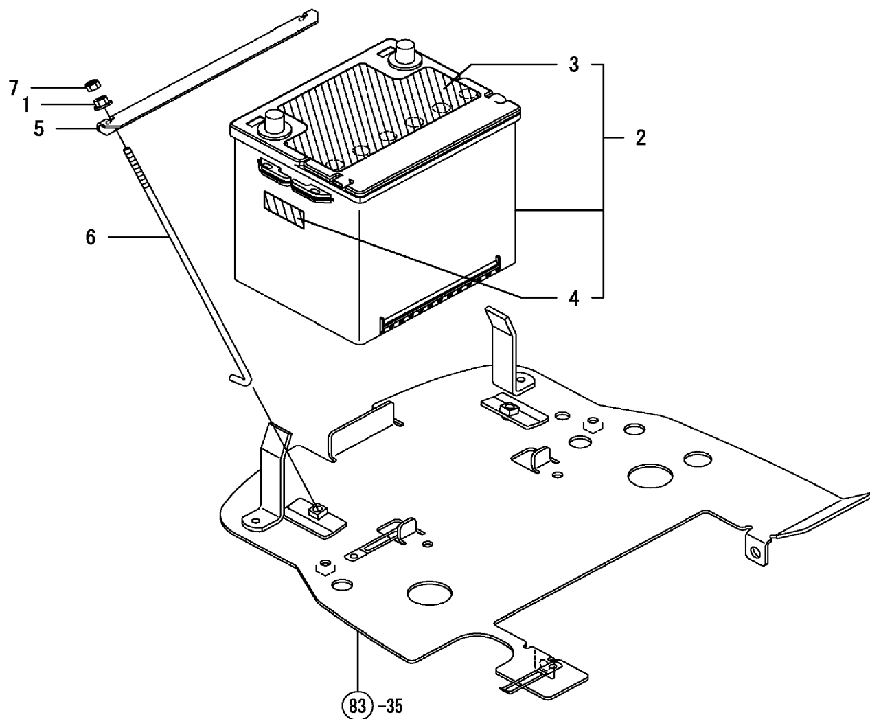
FIG. 77. BATTERY
