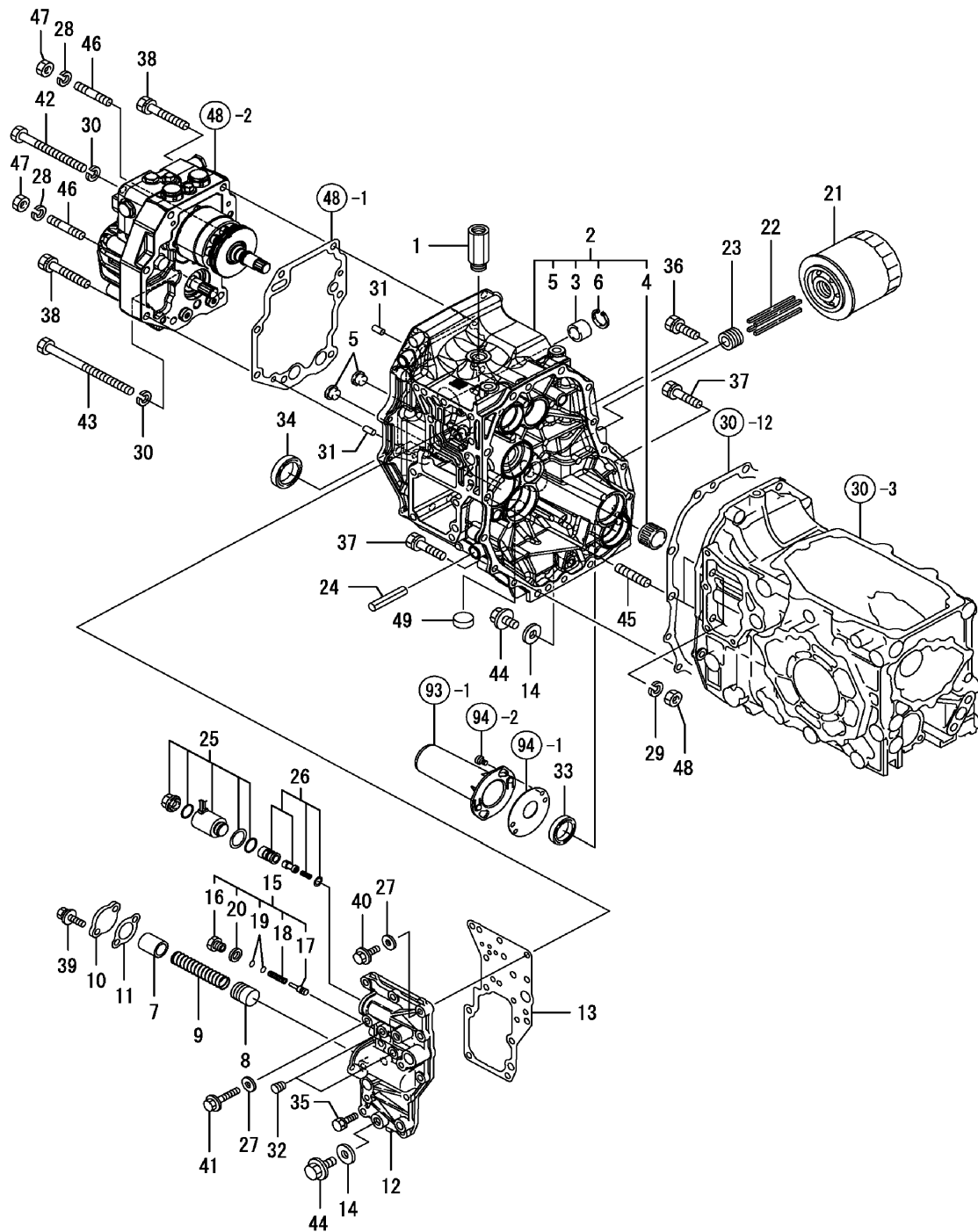
FIG. 31 CENTER PLATE
