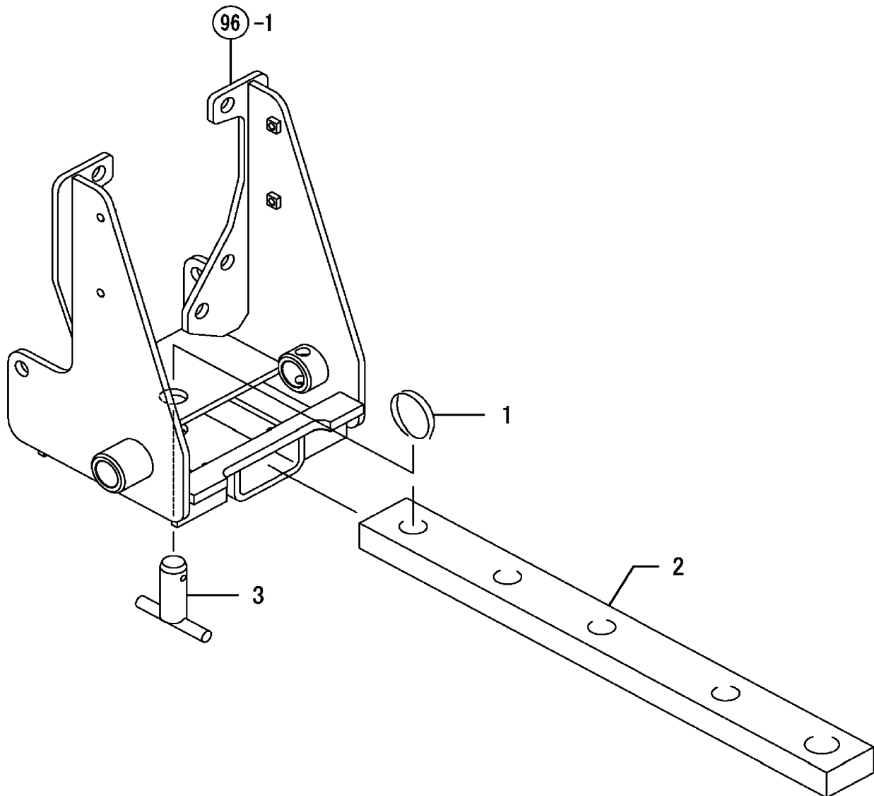
FIG. 97. DRAWBAR HITCH
