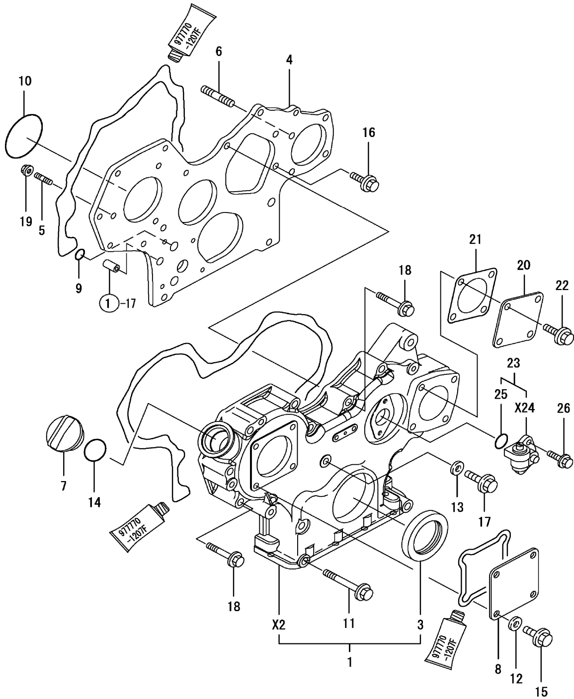
FIG. 2. GEAR HOUSING
