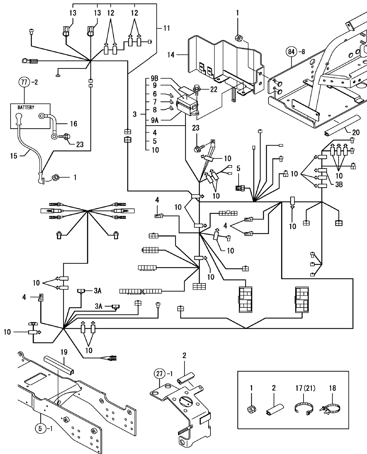
FIG. 76. WIRE HARNESS
