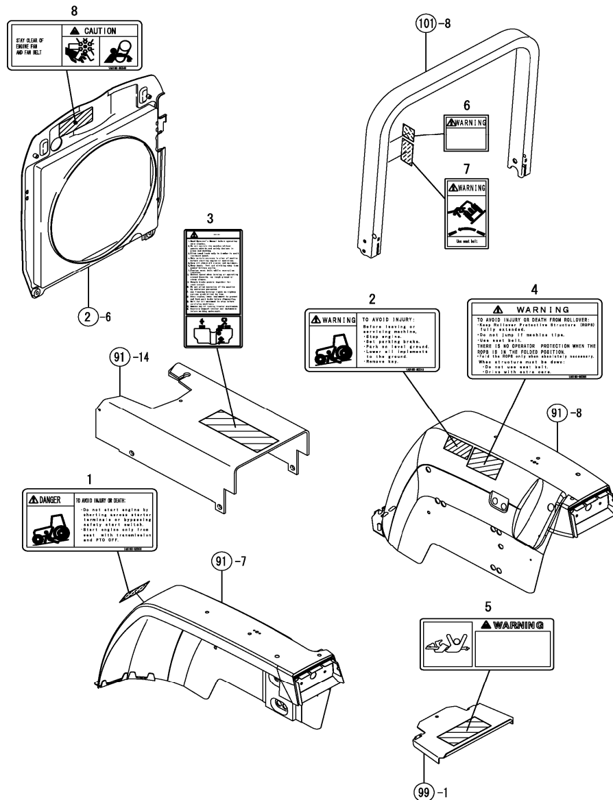
FIG. 96. LABELS, SAFETY
