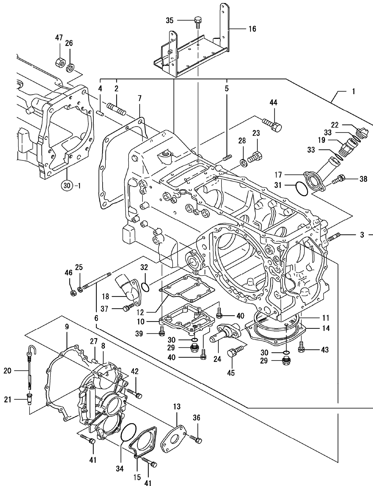
FIG. 35. TRANSMISSION CASE
