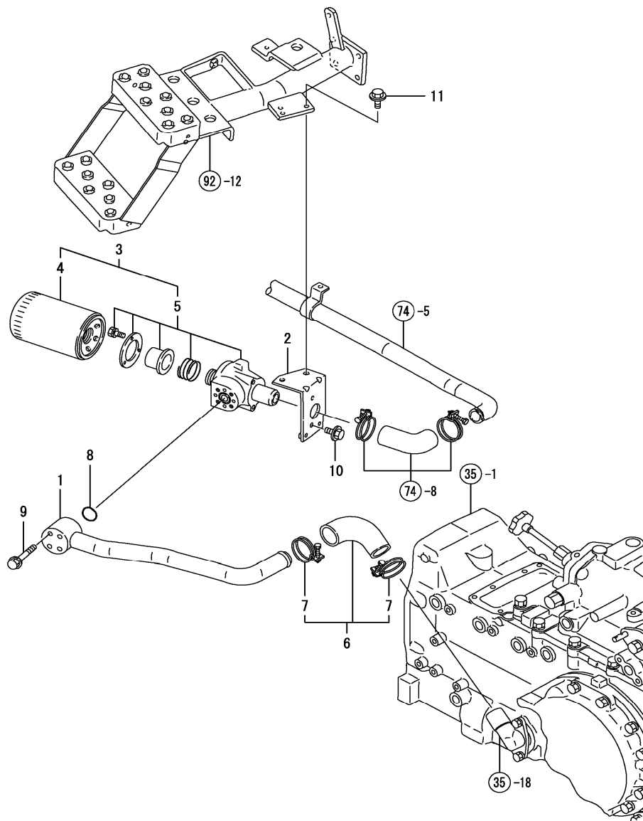
FIG. 75. HYDRAULIC FILTER
