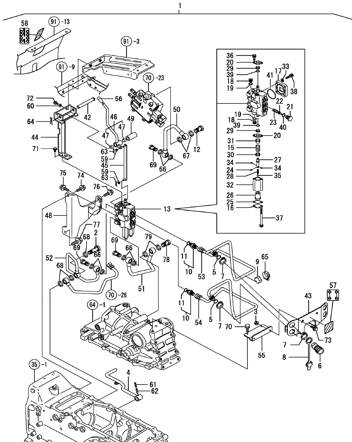
FIG. 103. REAR REMOTE VALVE 1P
