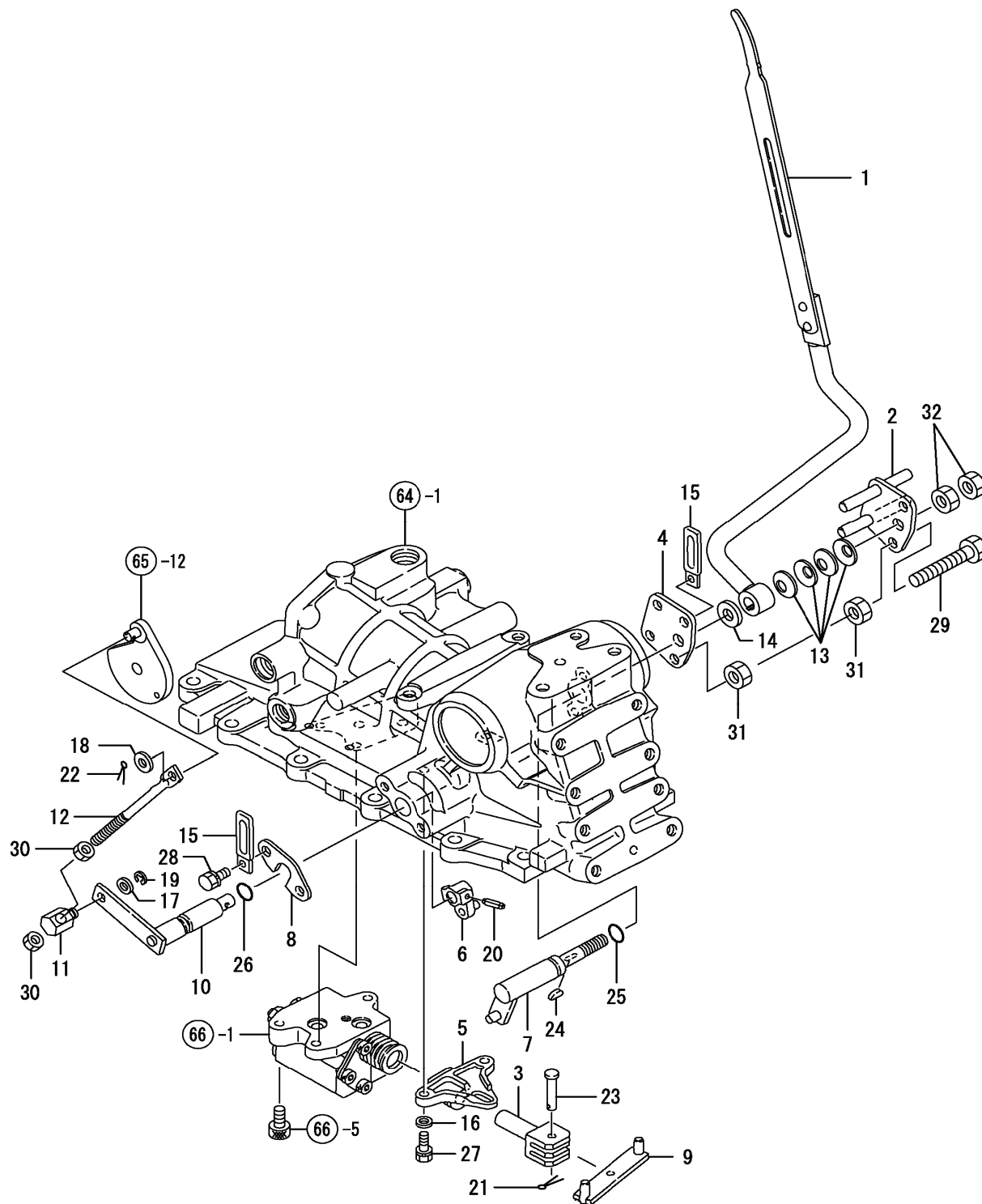
FIG. 72. HYDRAULIC CONTROL
