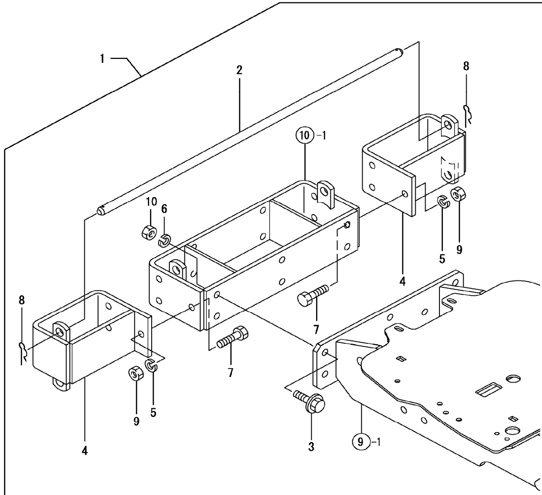
FIG. 104. EXTRA HITCH
