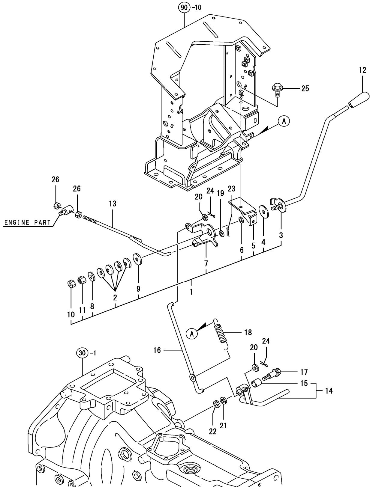
FIG. 3. ACCELERATOR LEVER
