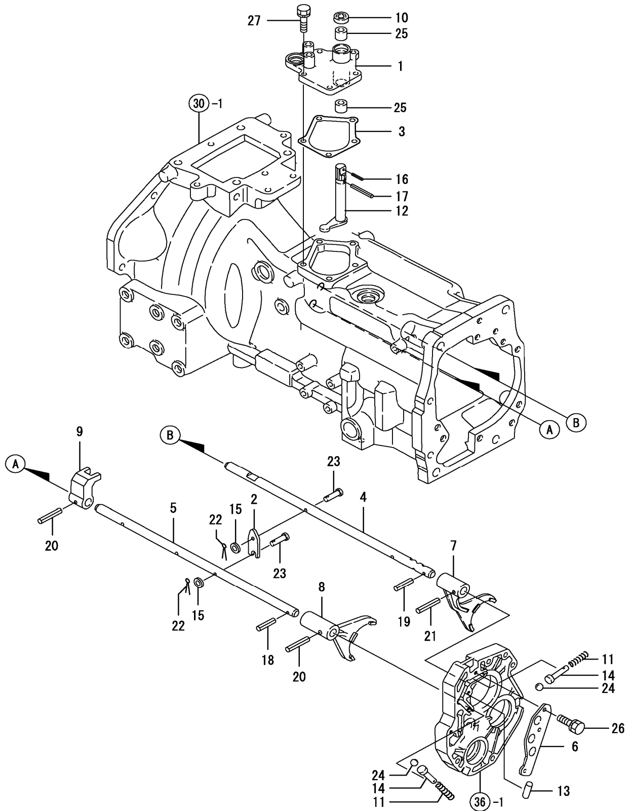
FIG. 47. MAIN CHANGE
