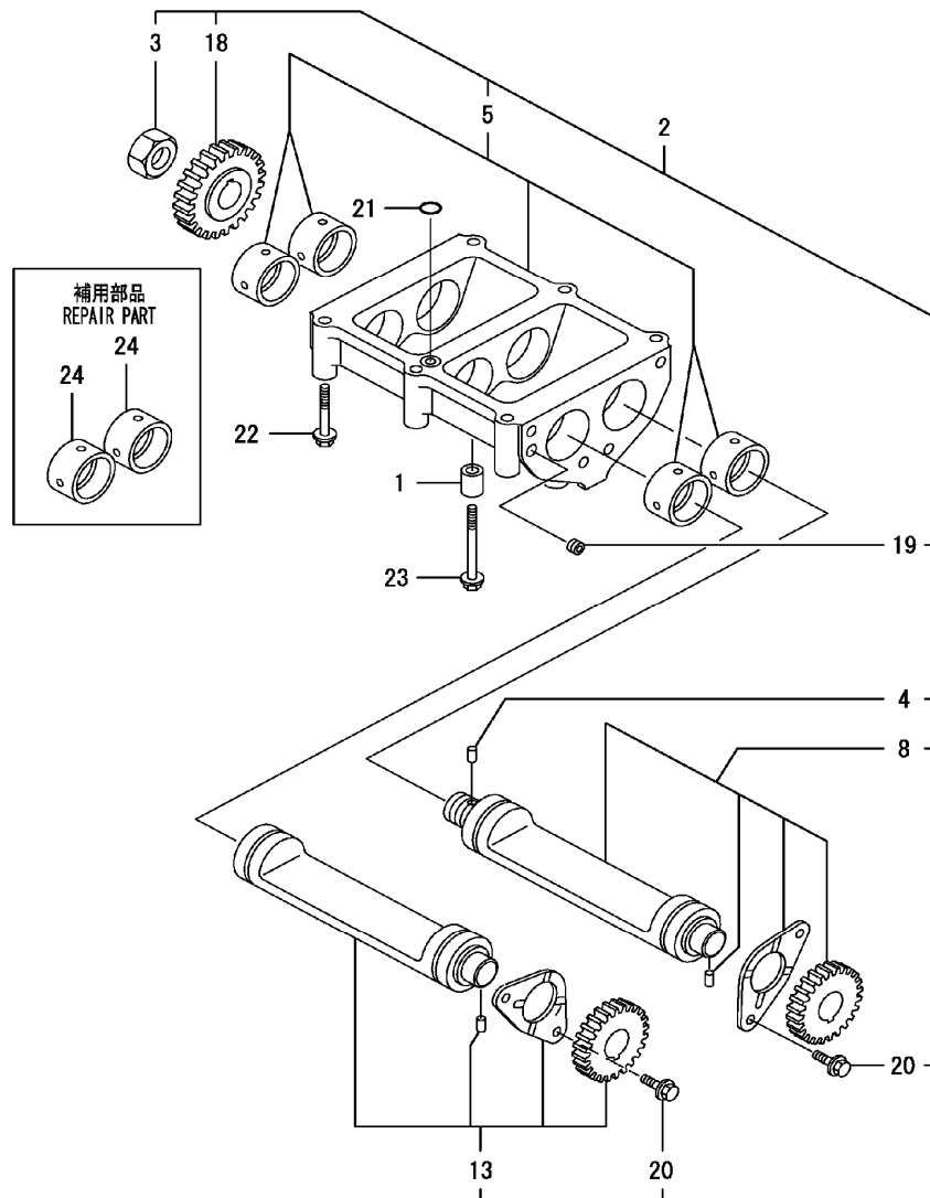
FIG. 10. BALANCER
