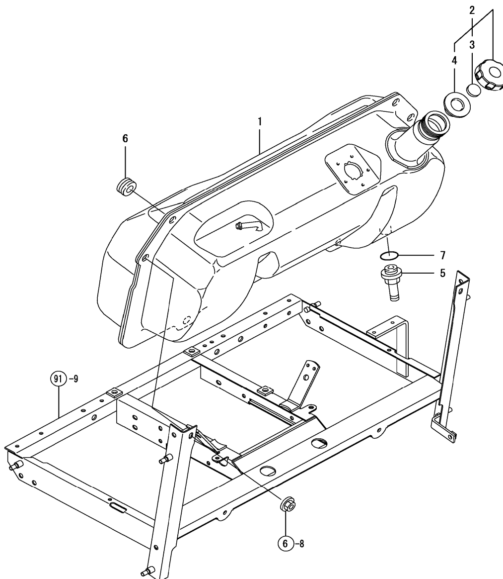
FIG. 5. TANK, FUEL OIL
