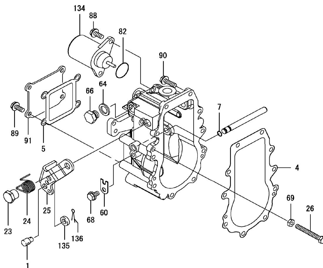
FIG. 14 GOVERNOR
