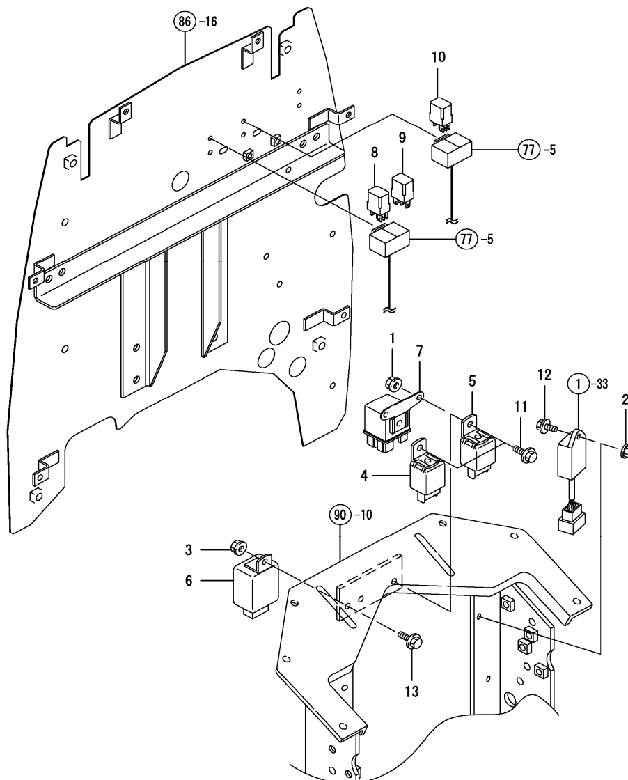
FIG. 84. RELAY
