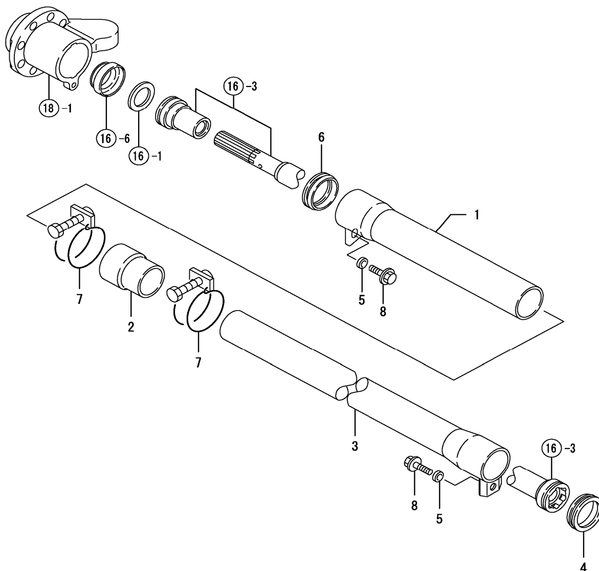
FIG. 22. SHAFT COVER
