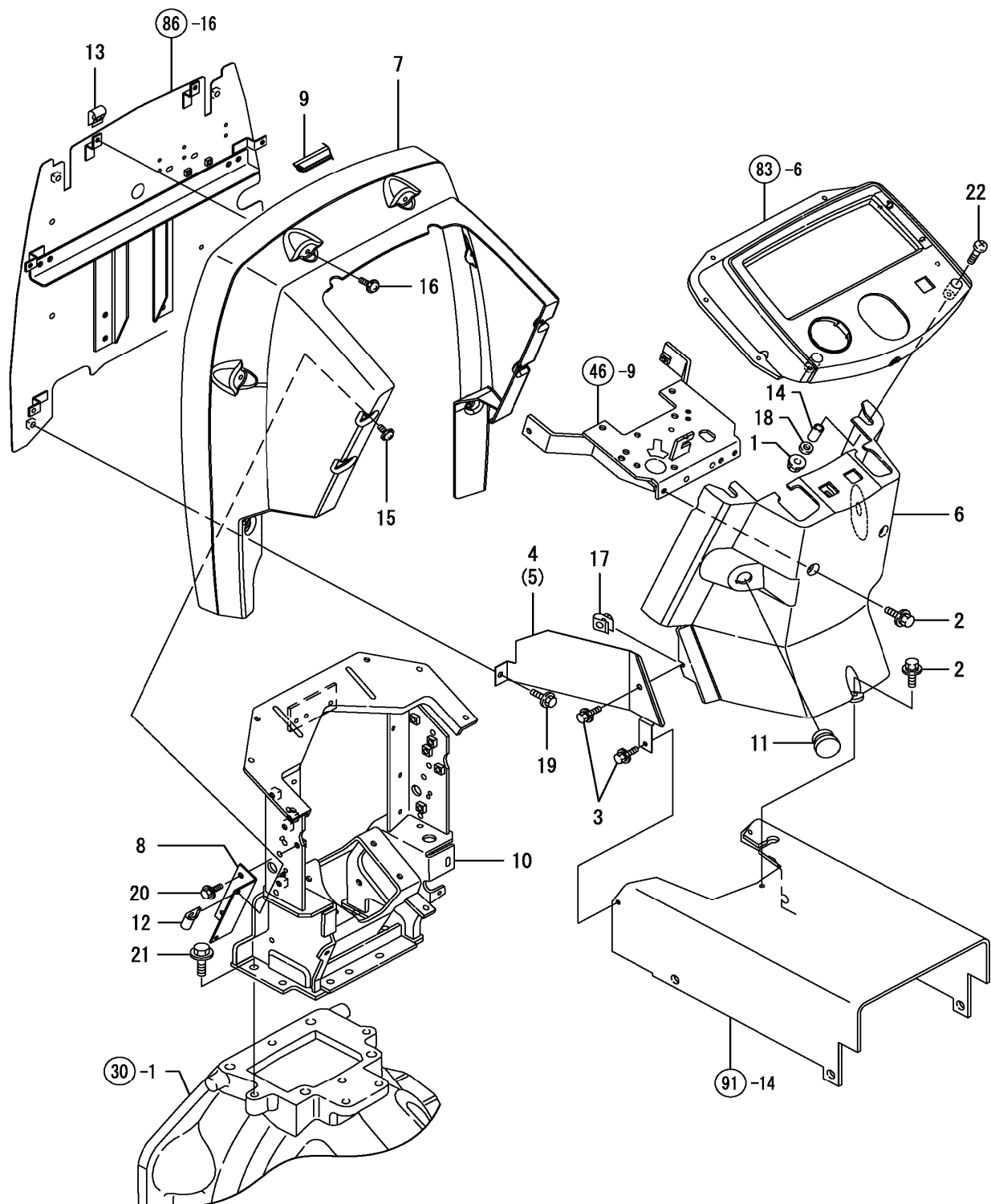
FIG. 90. DASHBOARD
