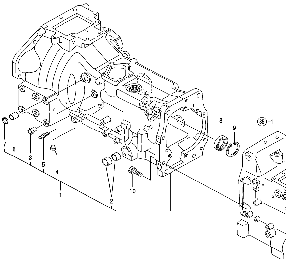
FIG. 30. CLUTCH HOUSING
