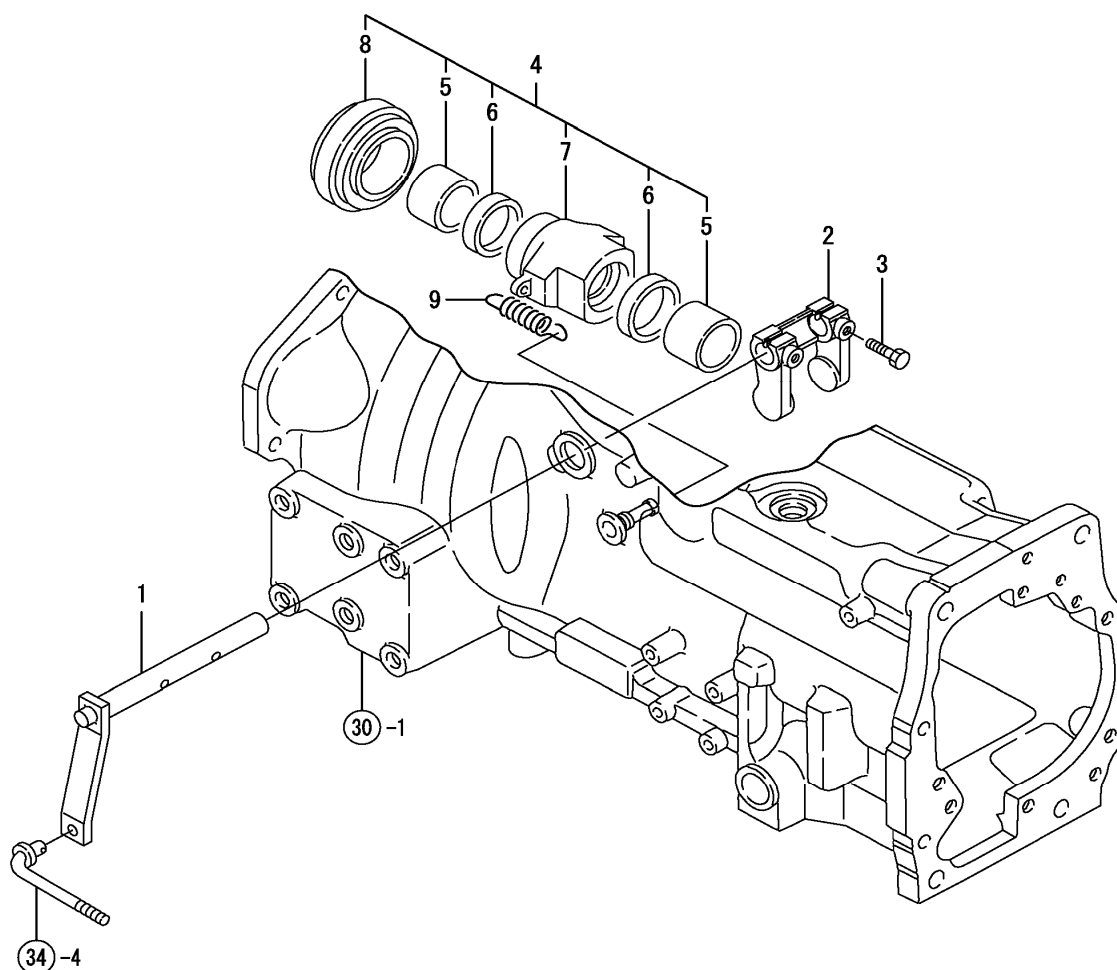
FIG. 33. CLUTCH RELEASE
