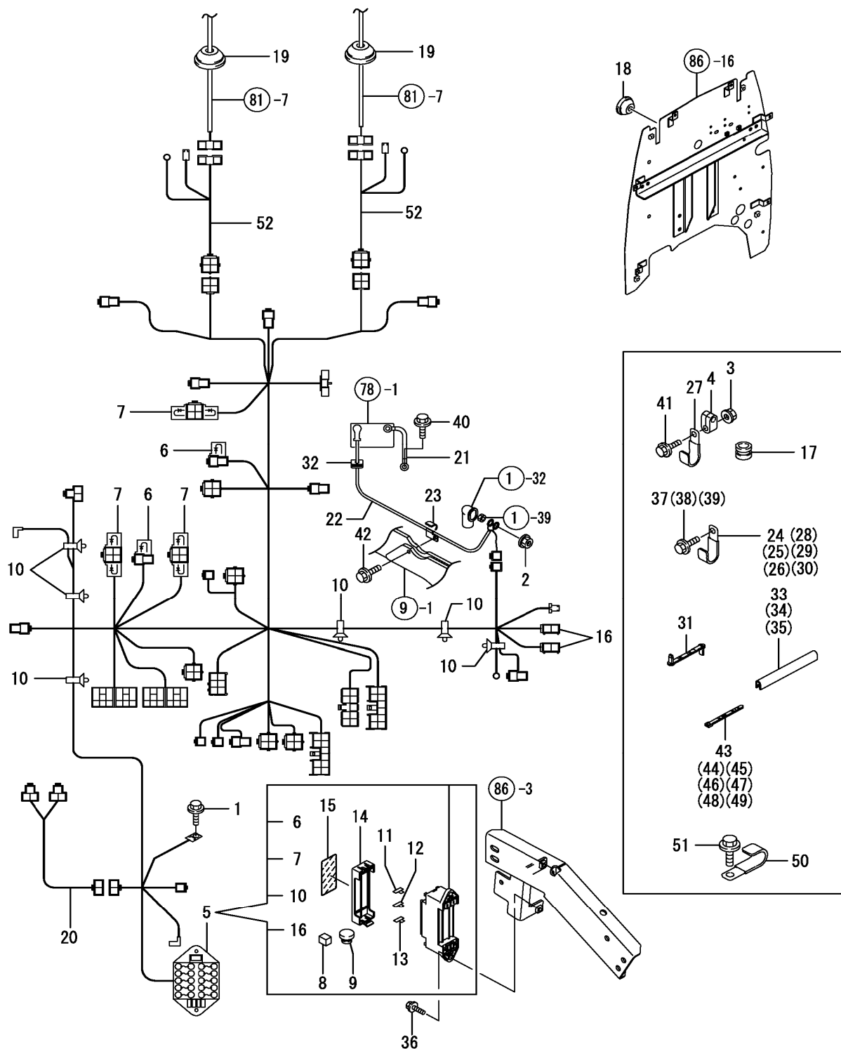
FIG. 77. WIRE HARNESS
