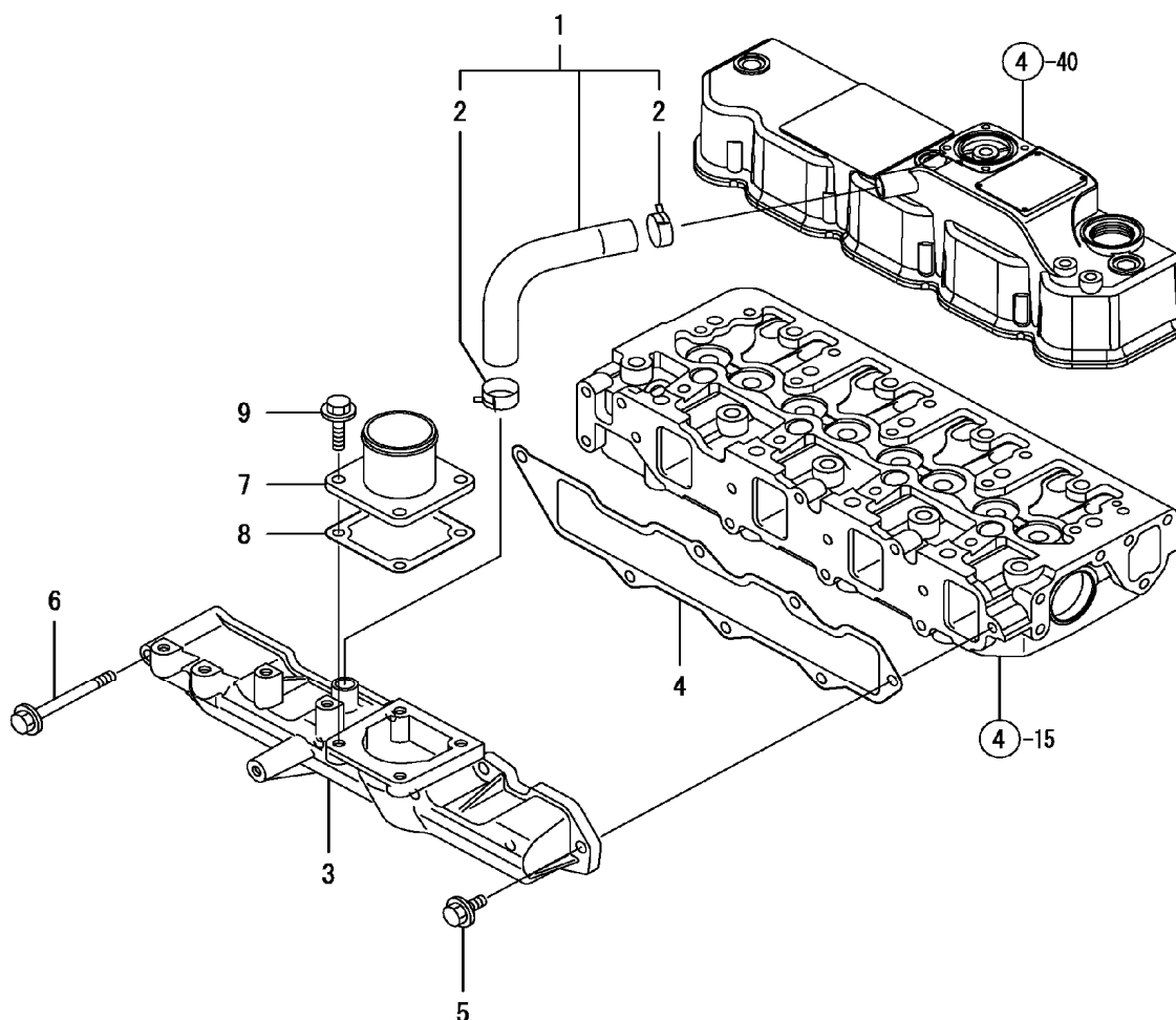
FIG. 8. SUCTION MANIFOLD
