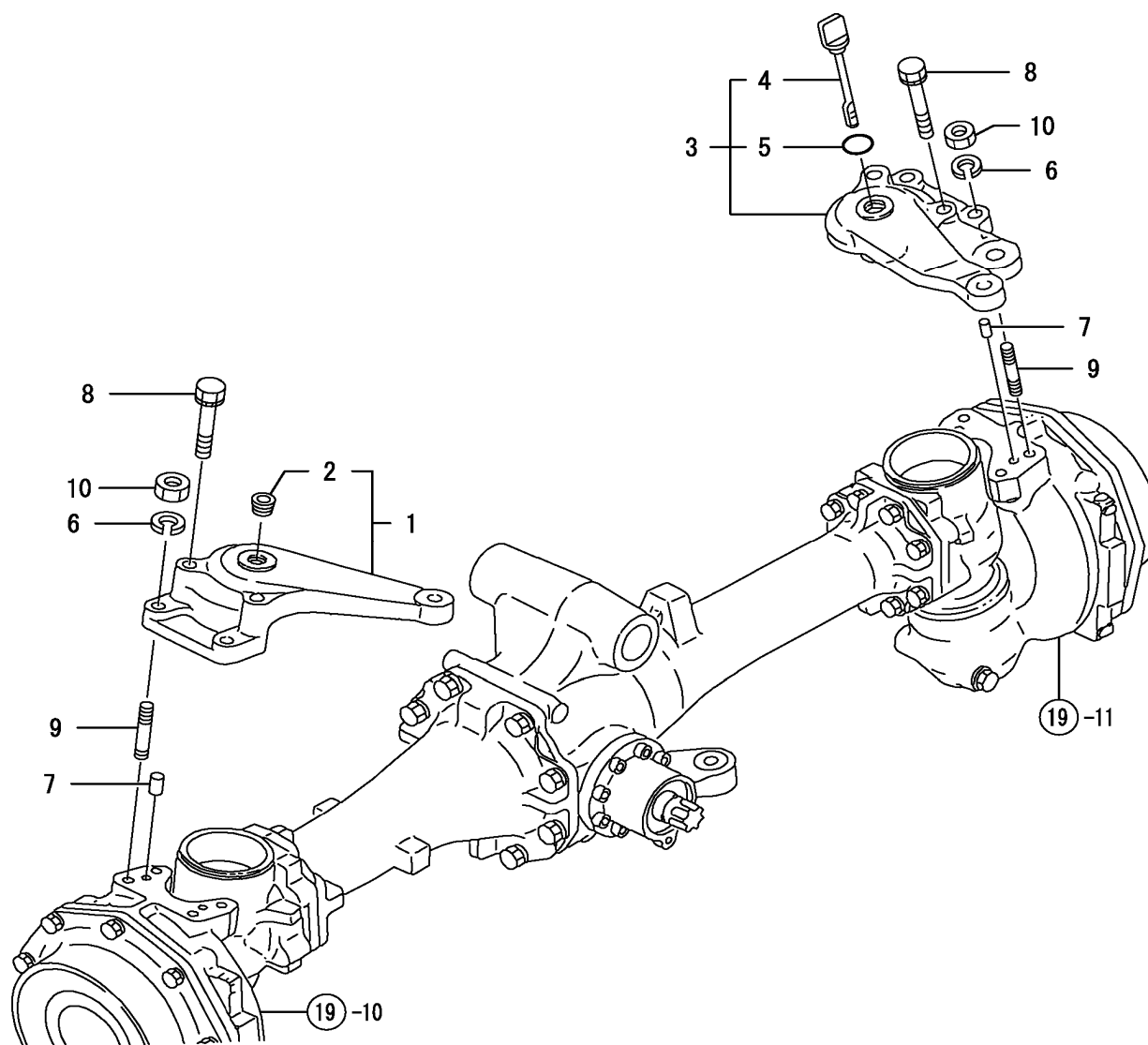
FIG. 12. KNUCKLE ARM
