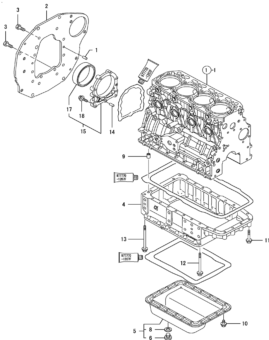
FIG. 3. MOUNTING FLANGE &amp; OIL SUMP
