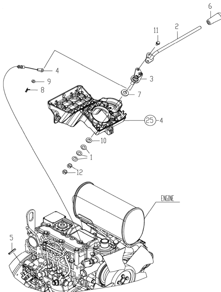
FIG. 3. ACCELERATOR LEVER
