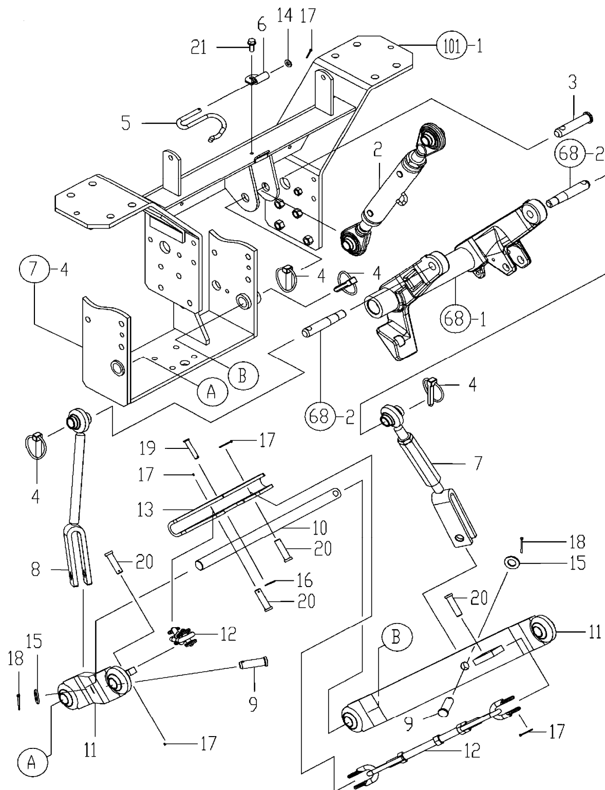
FIG. 98. THREE POINT LINK
