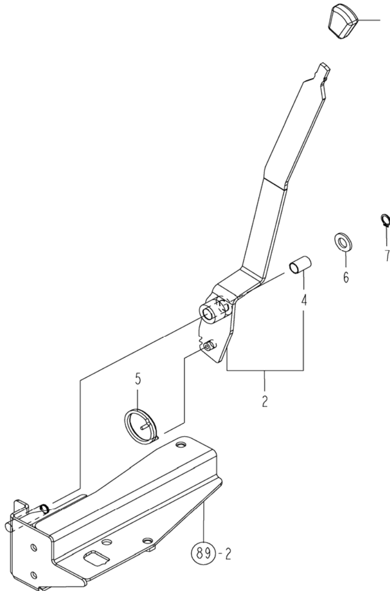
FIG. 66. PARKING BRAKE
