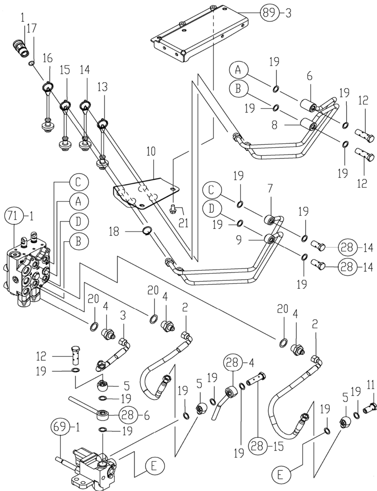
FIG. 76. PIPING, SCV
