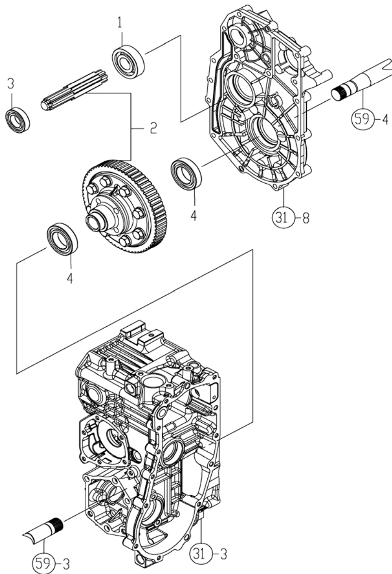
FIG. 55. REAR DIFFERENTIAL GEAR
