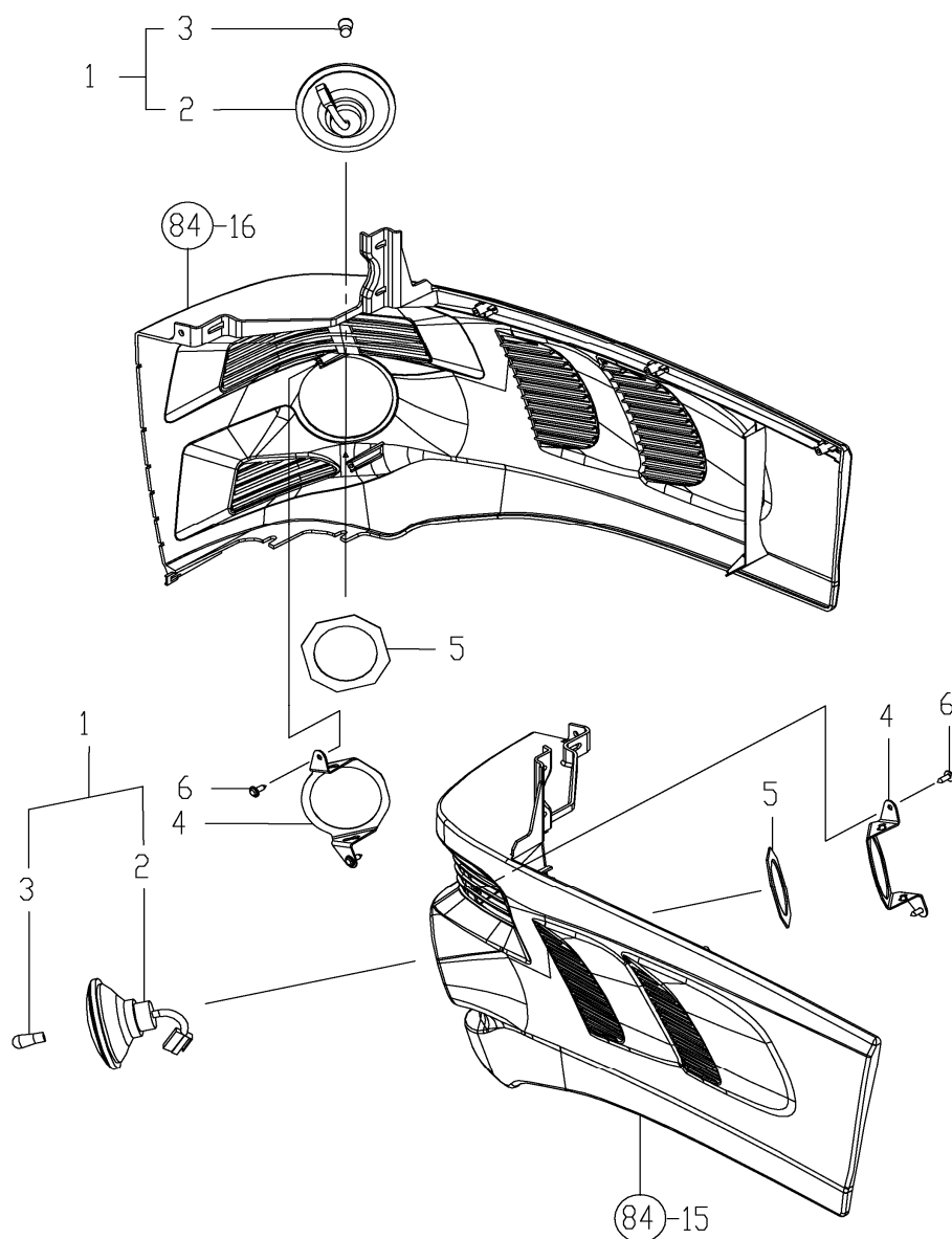
FIG. 82. FRONT LAMPS
