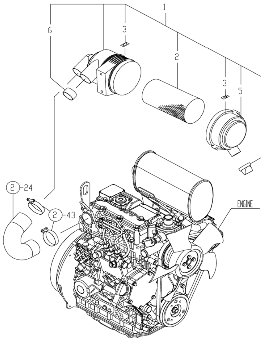
FIG. 1. ENGINE ACCESSORY
