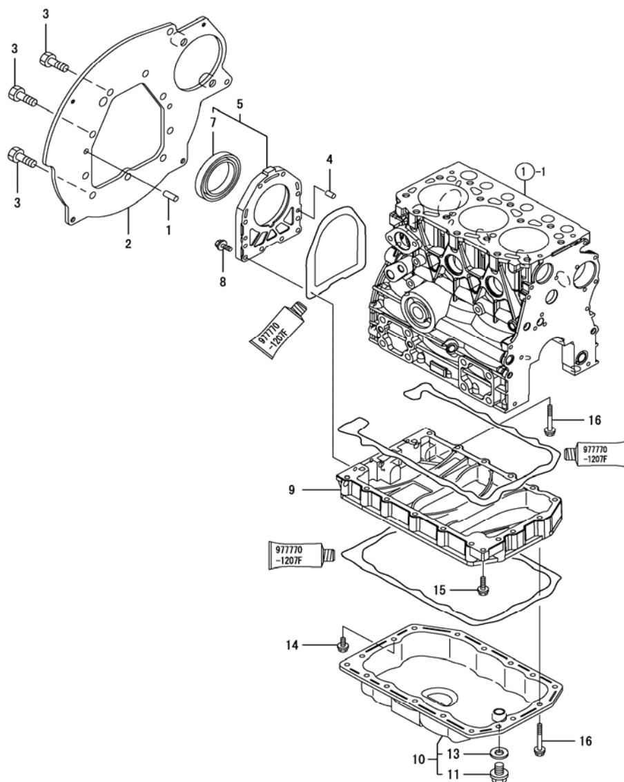
FIG. 3. OIL PAN &amp; REAR ENGINE PLATE
