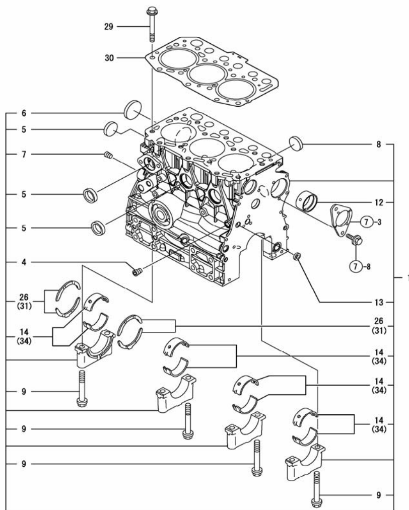
FIG. 1. CYLINDER BLOCK
