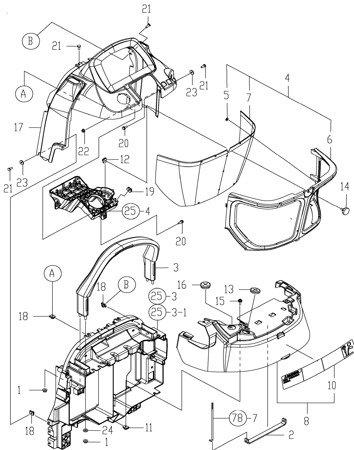
FIG. 86. DASHBOARD B
