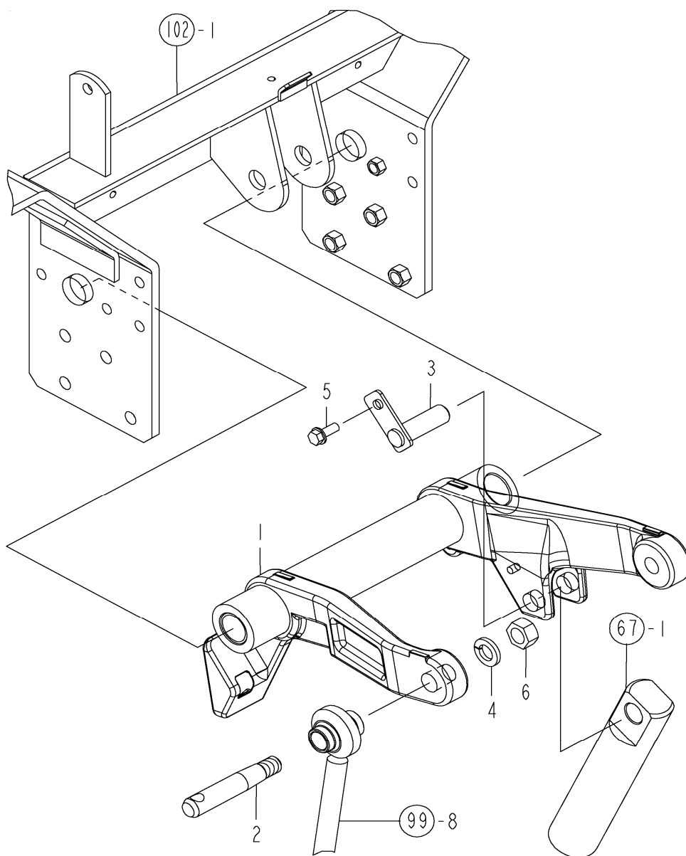
FIG. 68. LIFT ARM
