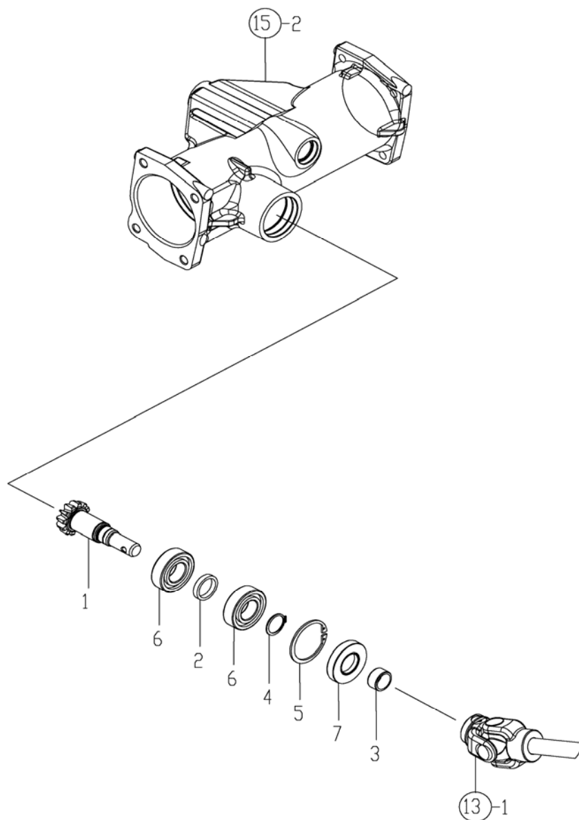
FIG. 11. DRIVE PINION
