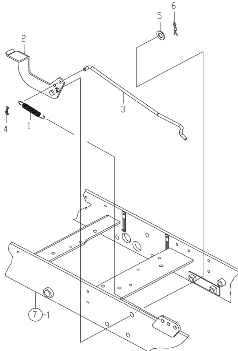
FIG. 58. DIFFERENTIAL PEDAL
