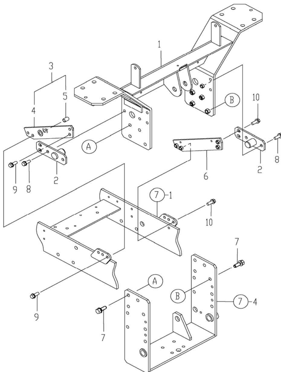
FIG.101. LOWER FRAME
