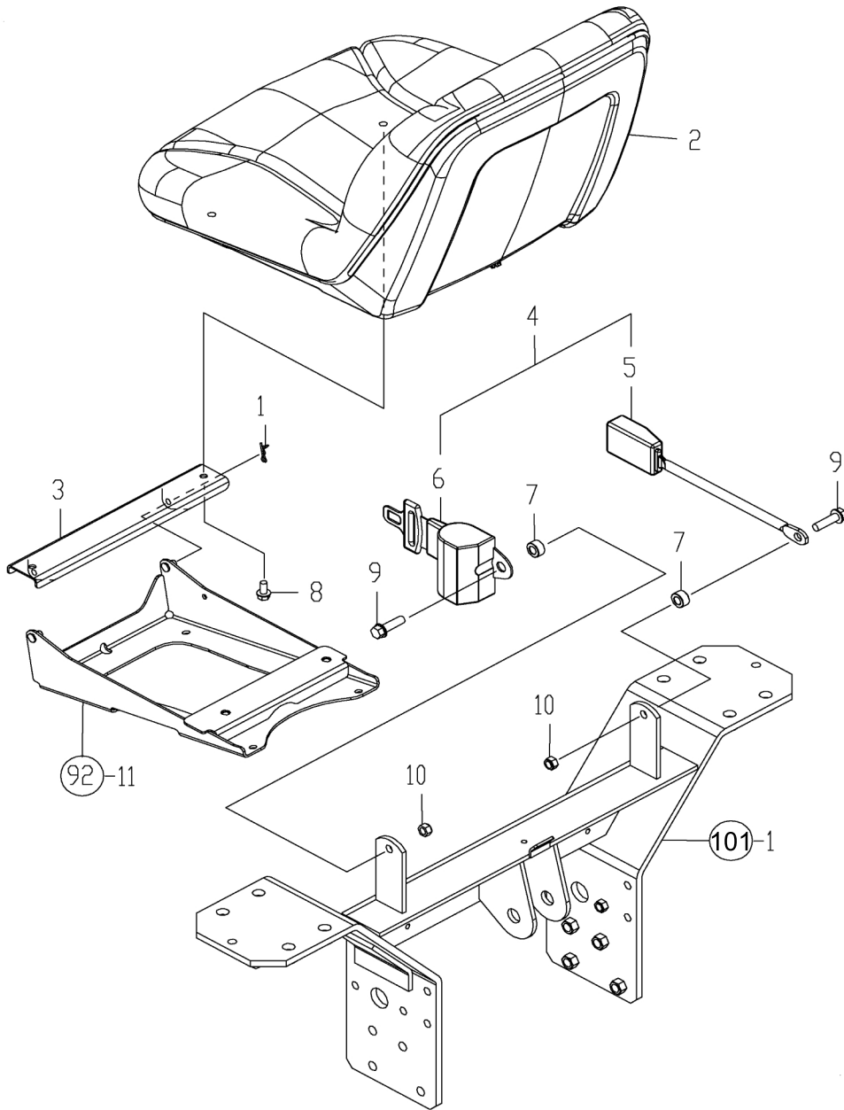
FIG. 91. SEAT
