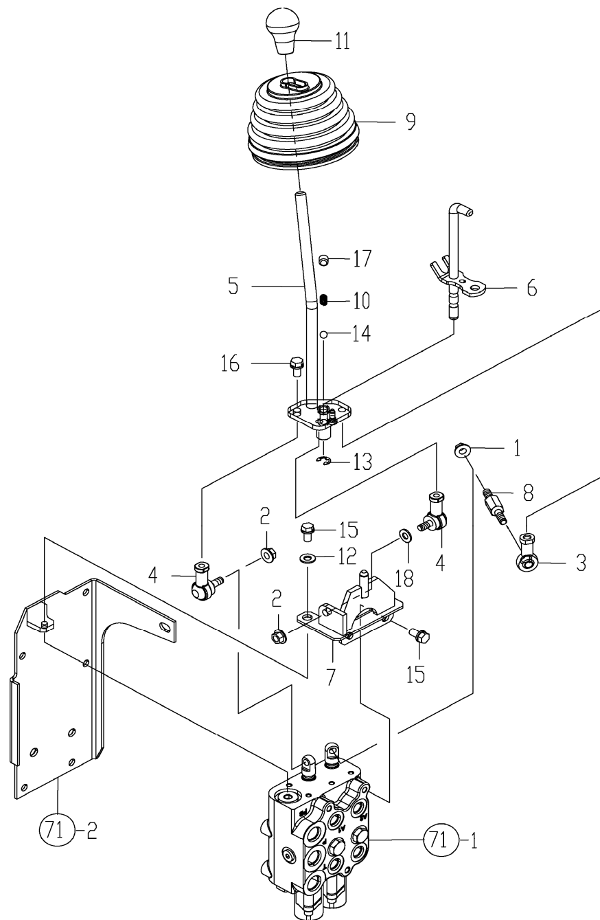
FIG. 72. LEVER, SCV
