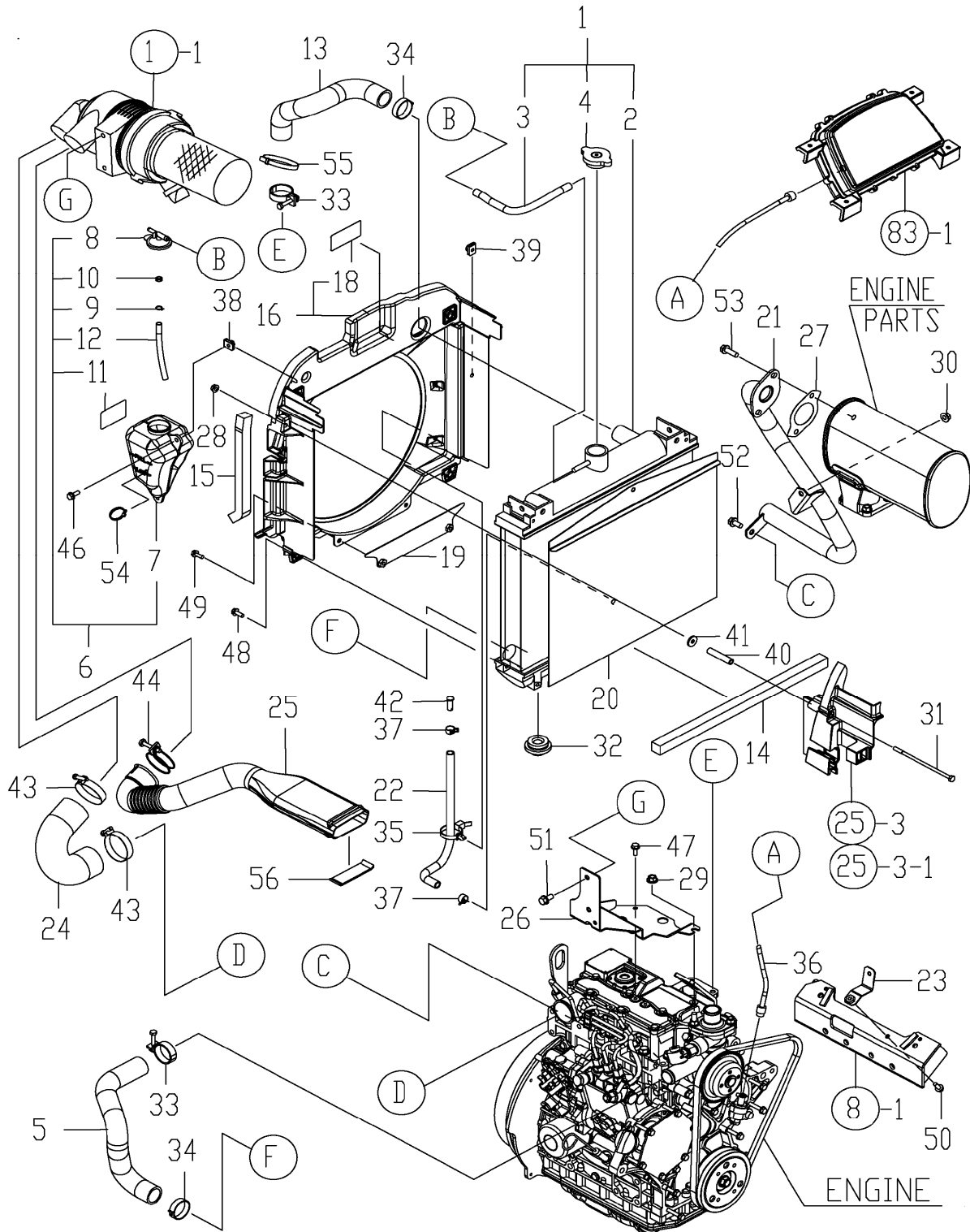
FIG. 2. ENGINE ACCESSORY MOUNTING
