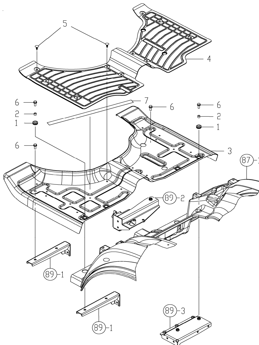
FIG. 90. FOOTREST
