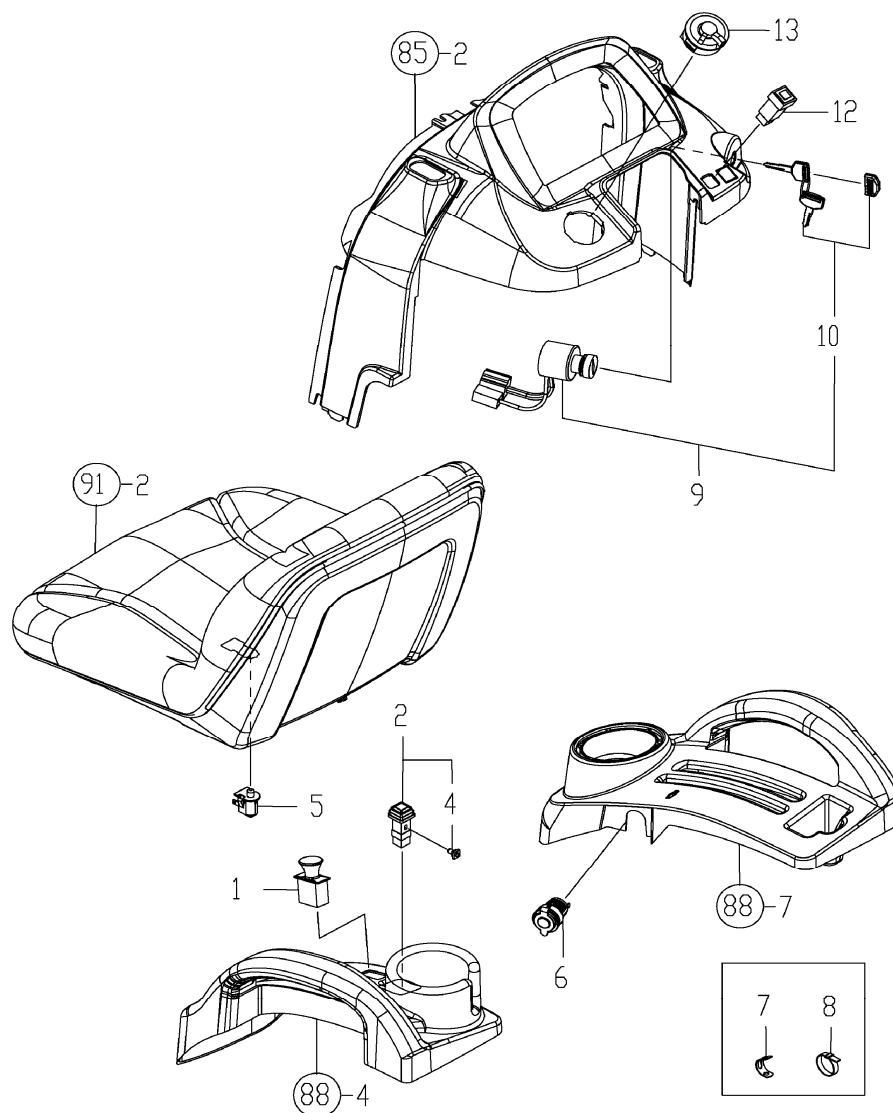
FIG. 80. SEAT SWITCH
