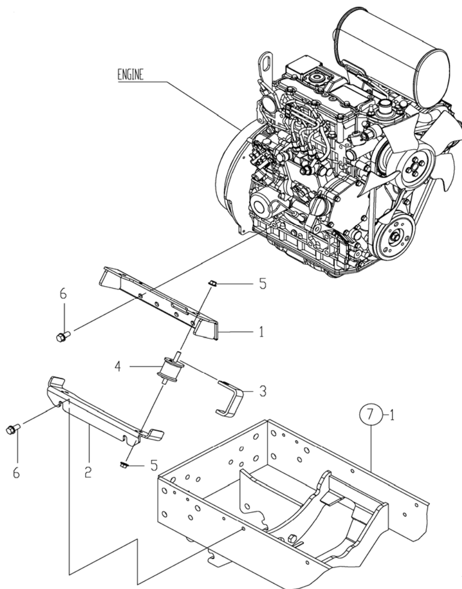
FIG. 8. ENGINE MOUNT
