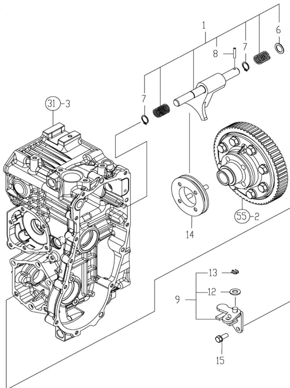
FIG. 57. DIFFERENTIAL LOCK
