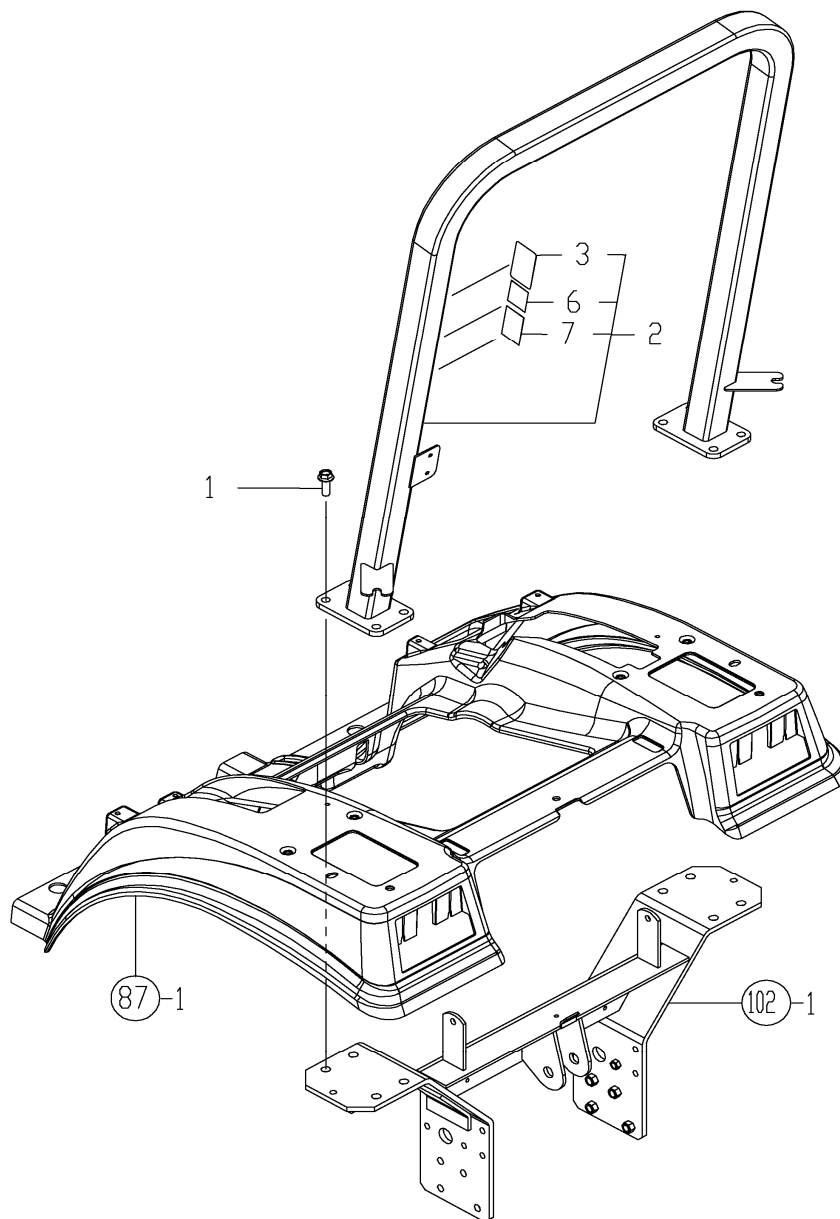
FIG.100. ROPS UPPER
