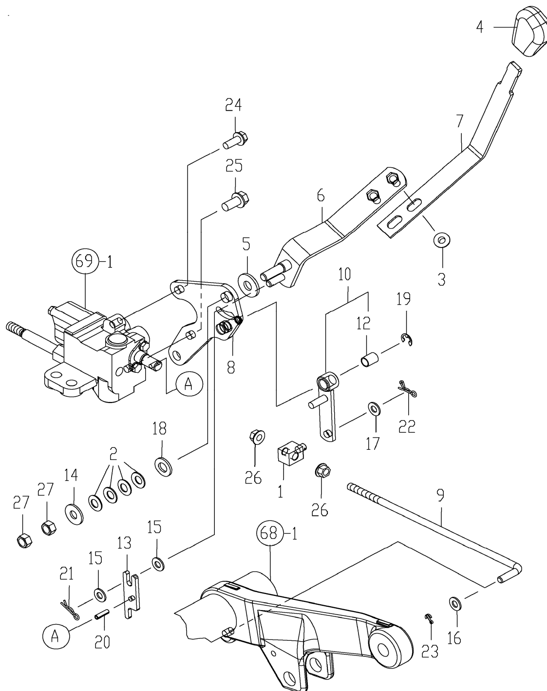
FIG. 73. HYDRAULIC CONTROL
