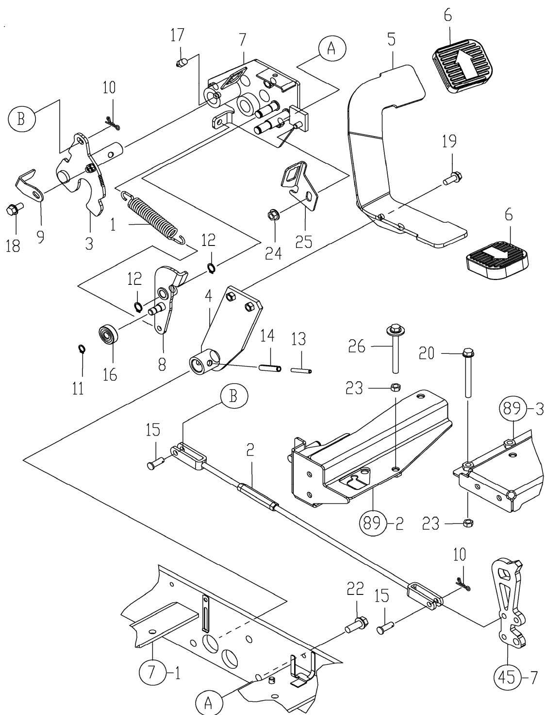
FIG. 50. HYDROSTATIC (HST) PEDAL
