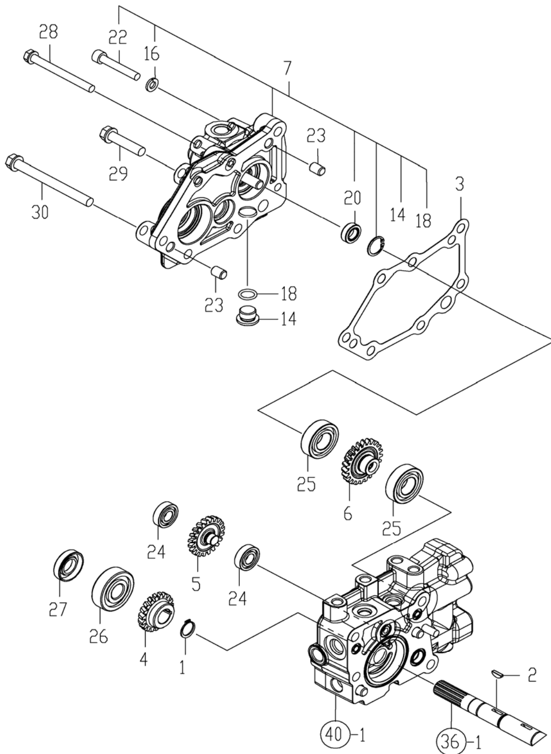
FIG. 53. GEAR PUMP
