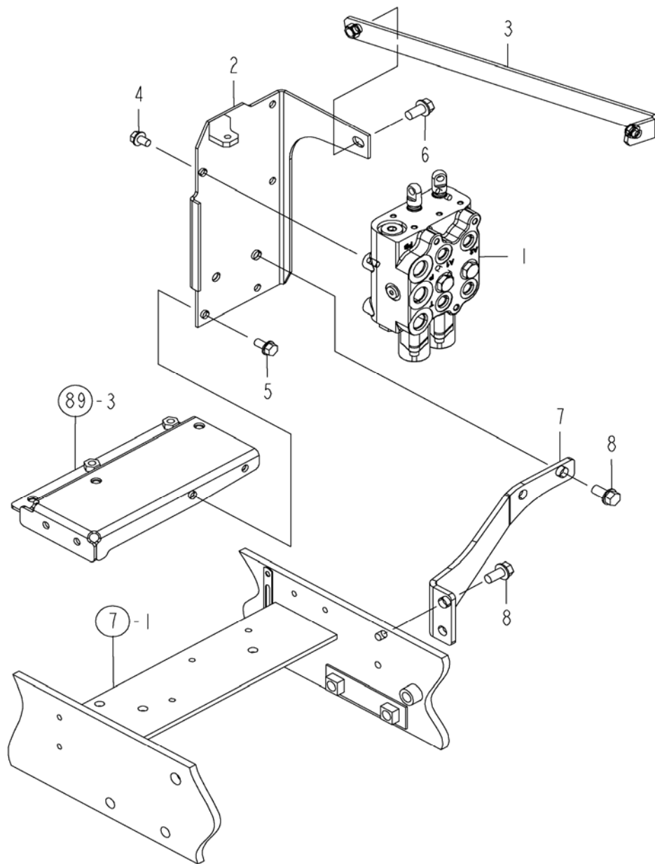
FIG. 71. VALVE, SCV
