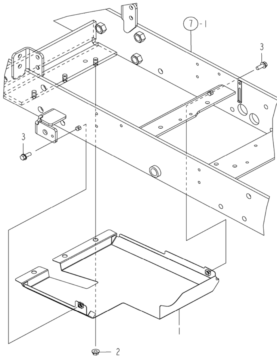
FIG. 5. FUEL TANK MOUNTING
