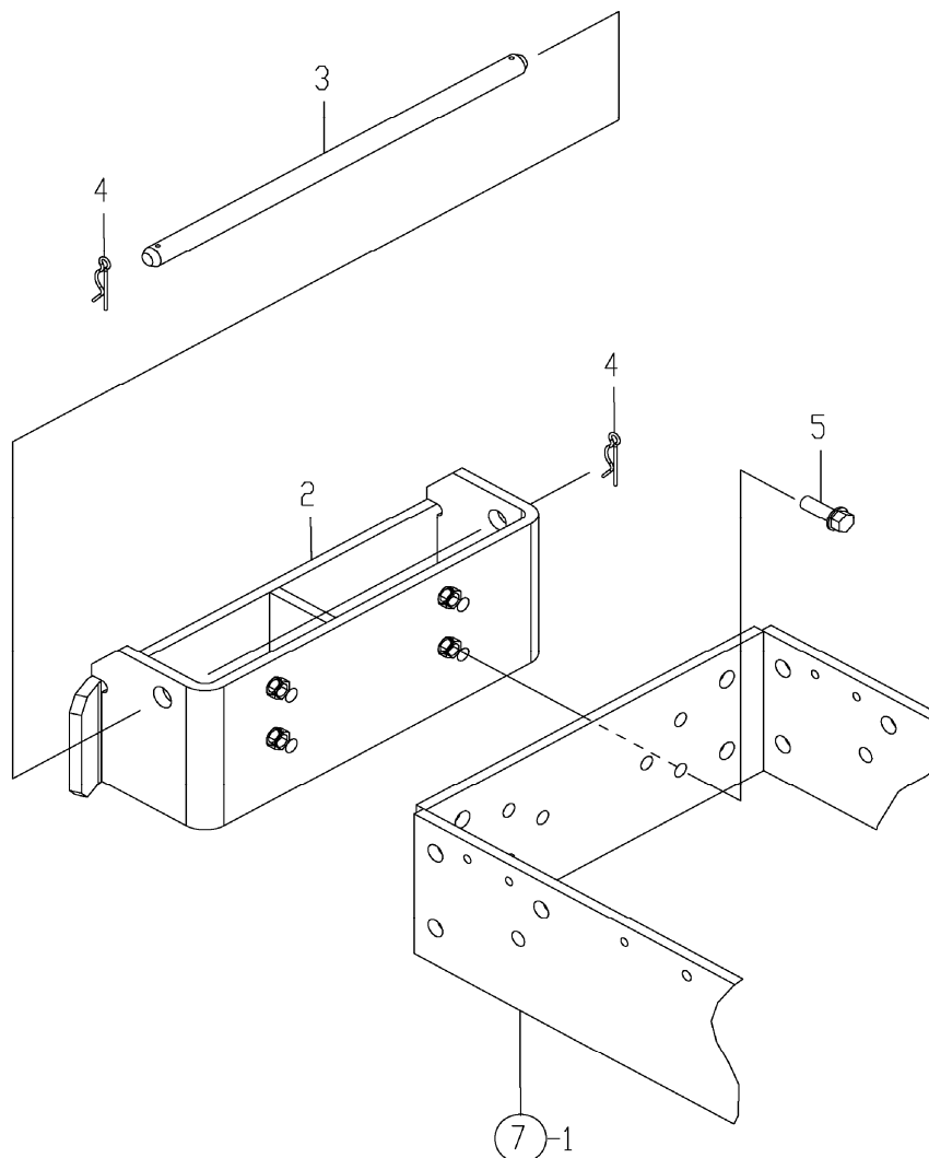
FIG. 103. FRONT HITCH
