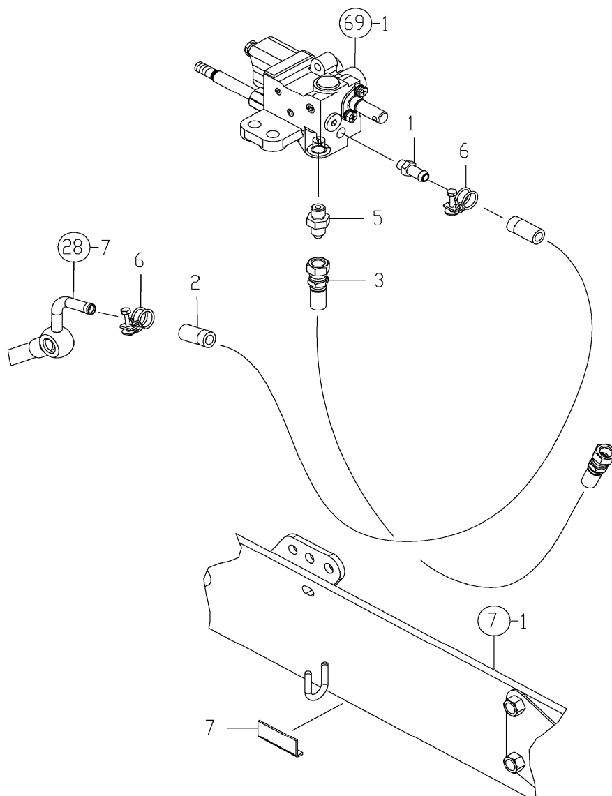
FIG. 74. HYDRAULIC PIPE
