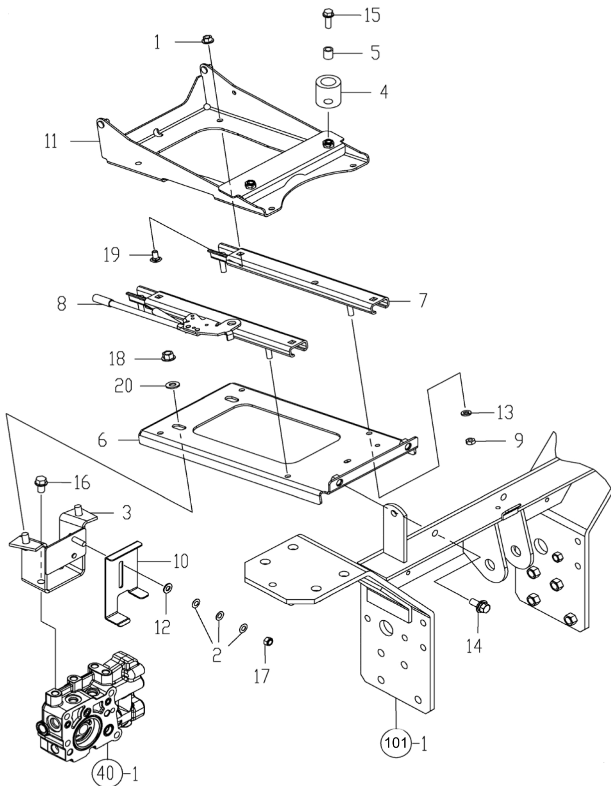
FIG. 92. SEAT STAY
