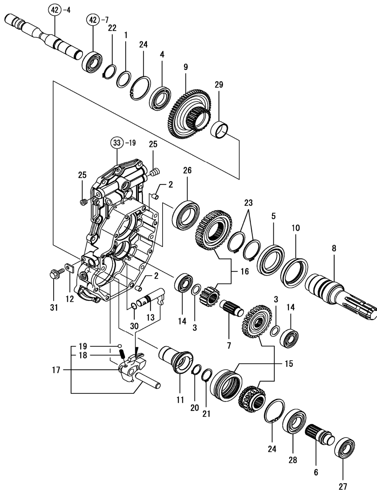
Fig. 45 - PTO Shaft, Rear
