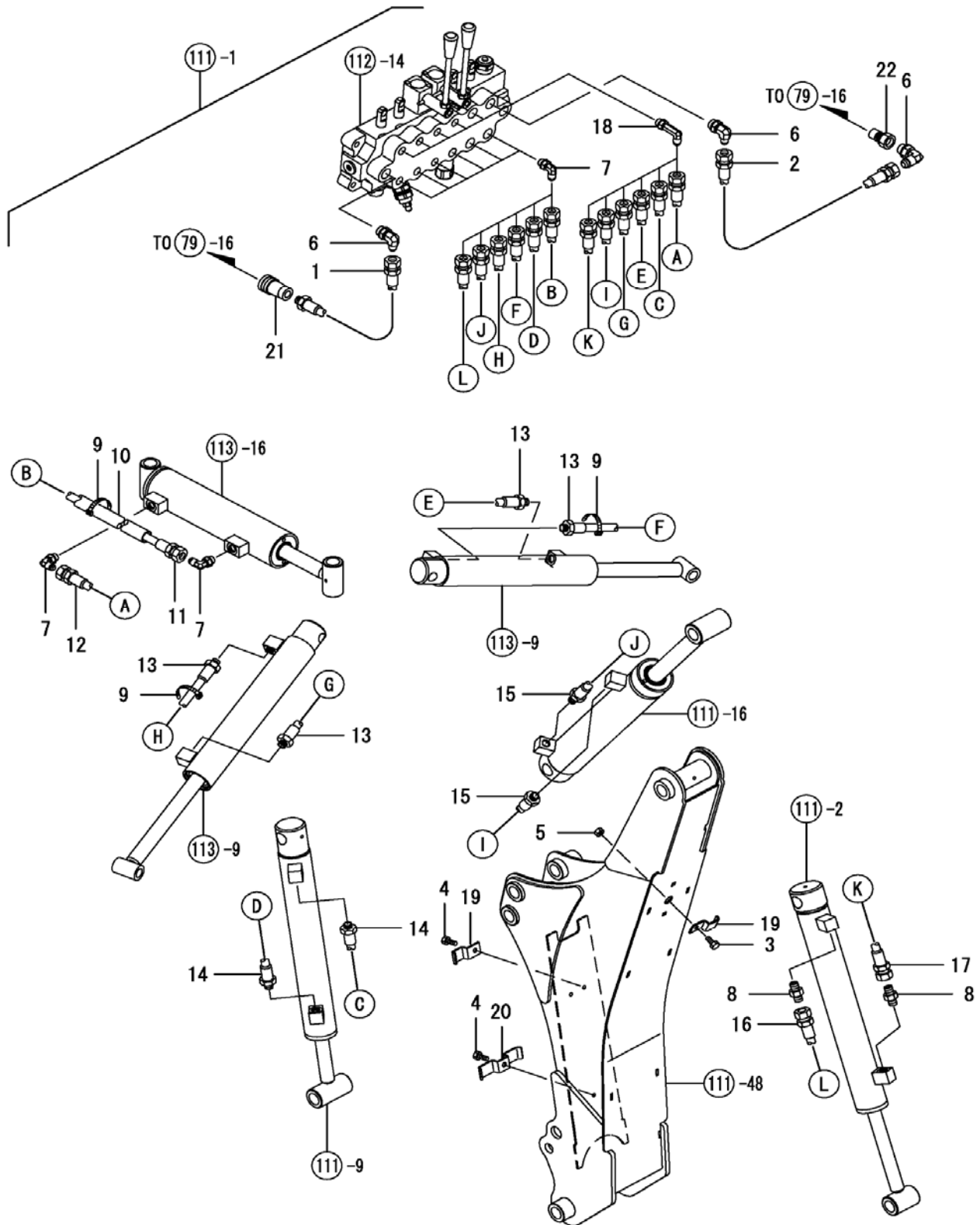
Fig. 114 - Backhoe, Piping
