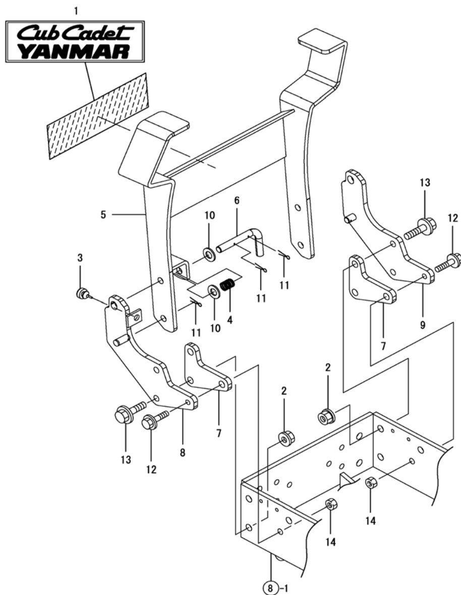
Fig. 104 - Front Grille Guard
