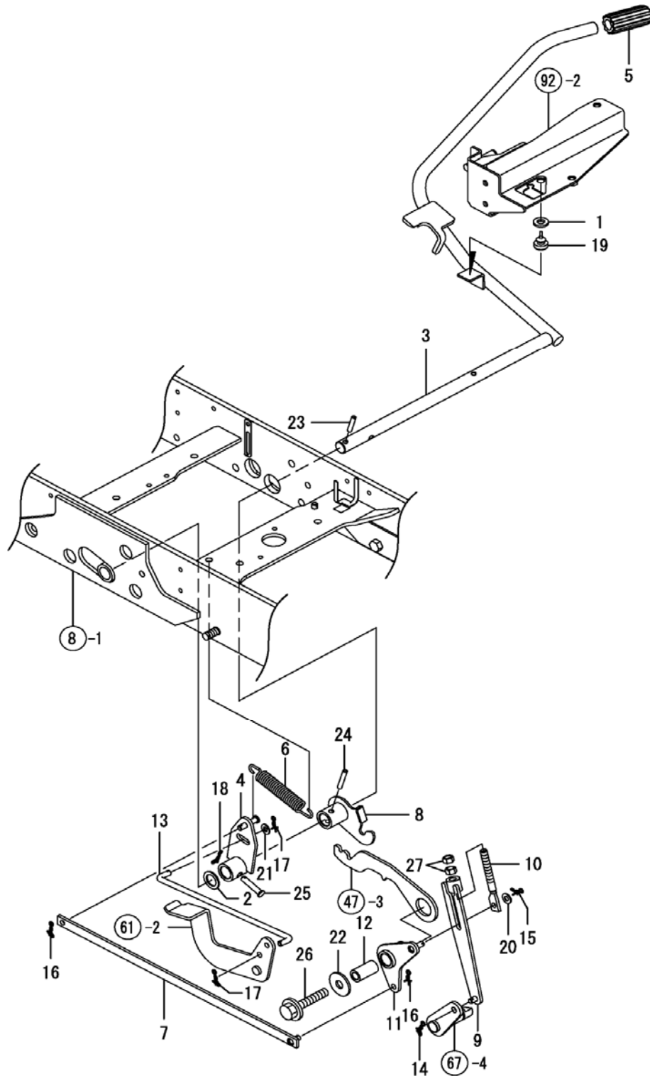
Fig. 68 - Brake Pedal
