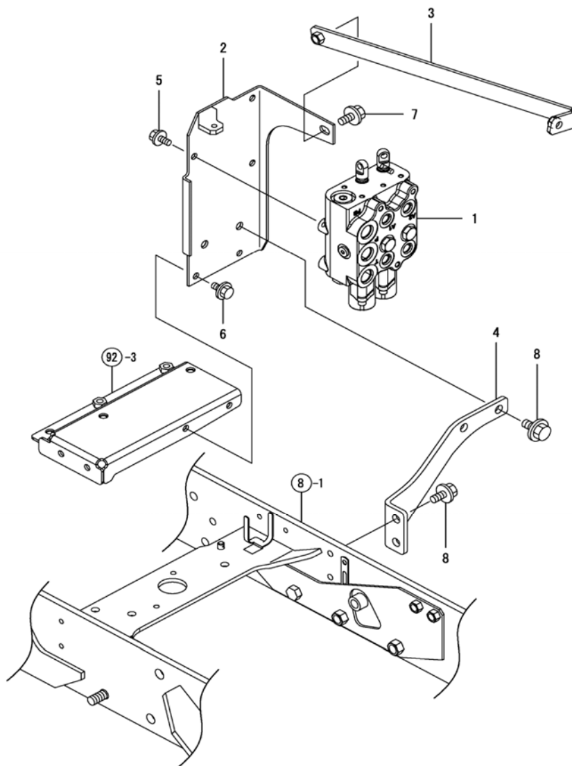
Fig. 74 - SCV Valve
