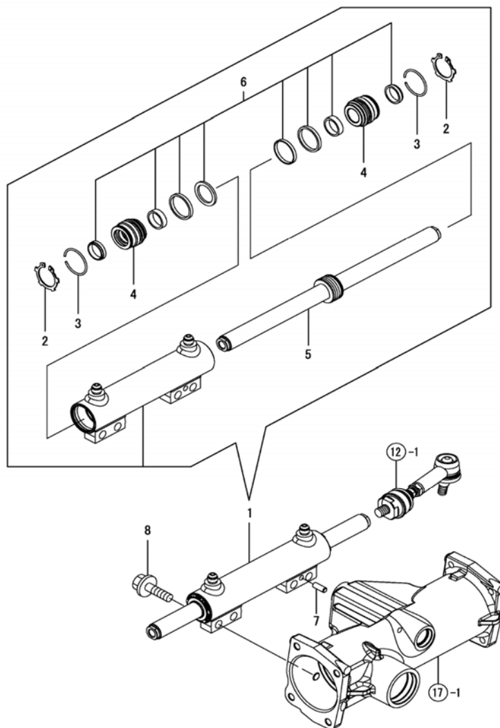
Fig. 29 - Power Steering Cylinder
