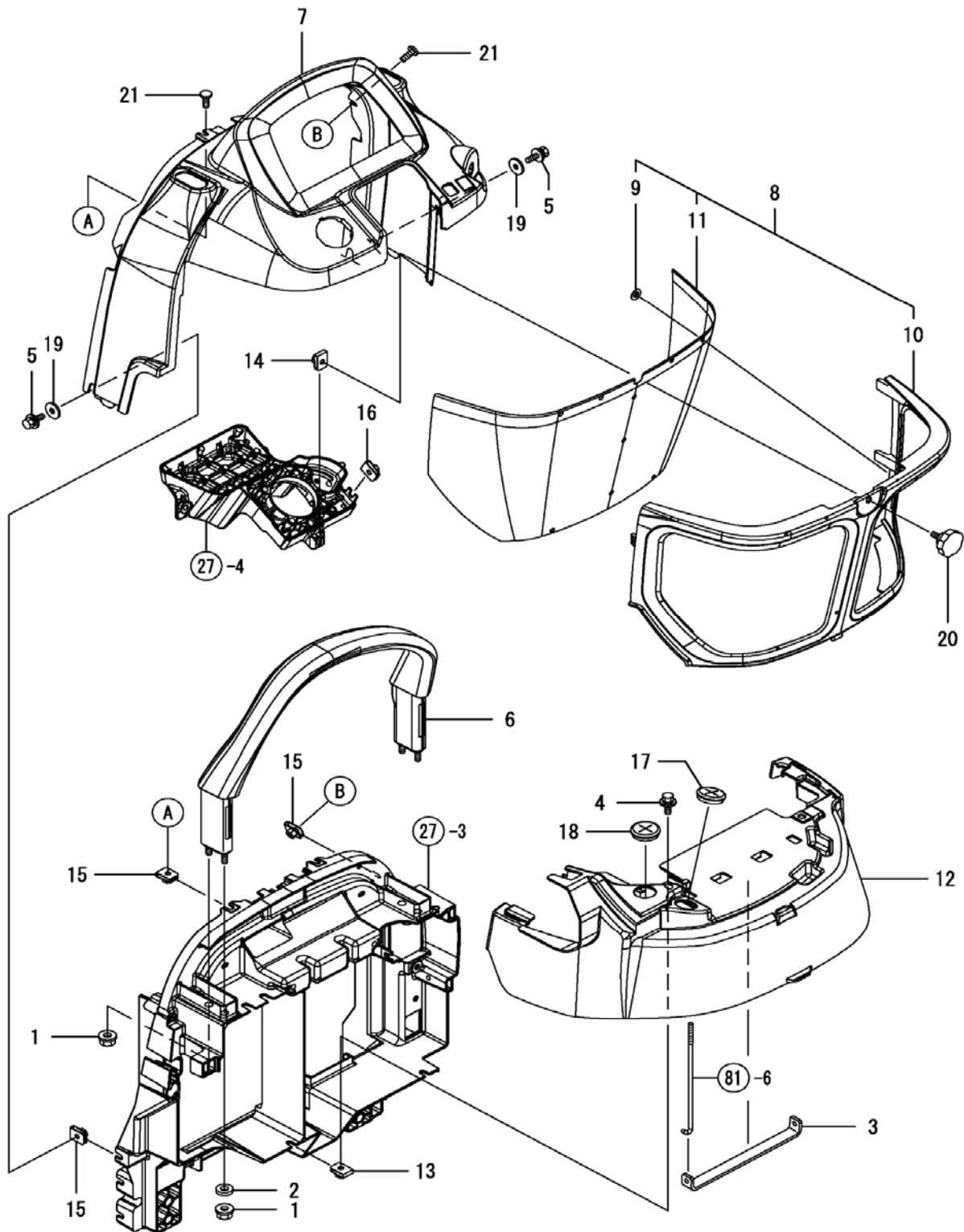
Fig. 89 - Dashboard
