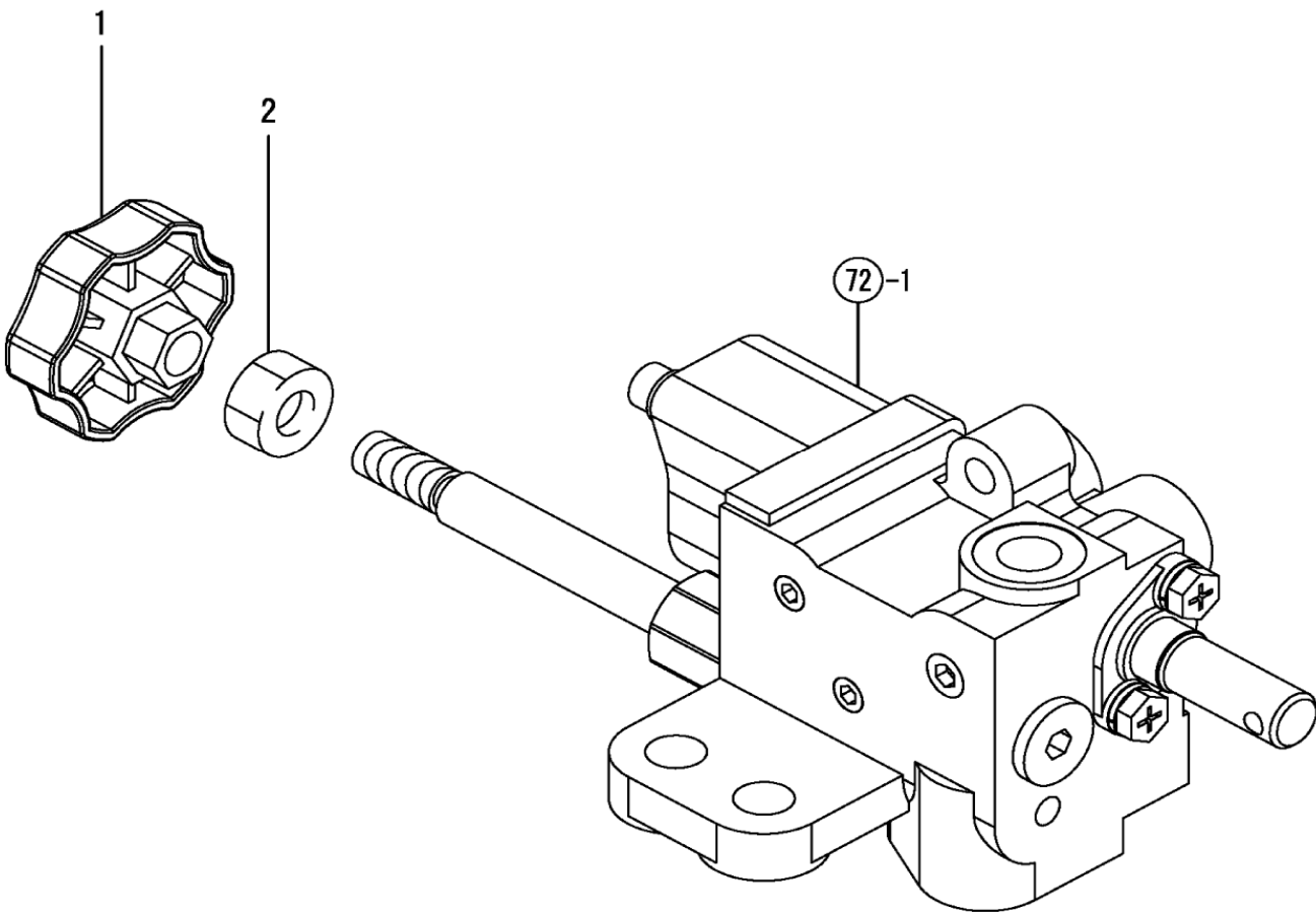
Fig. 73 - Stop Valve
