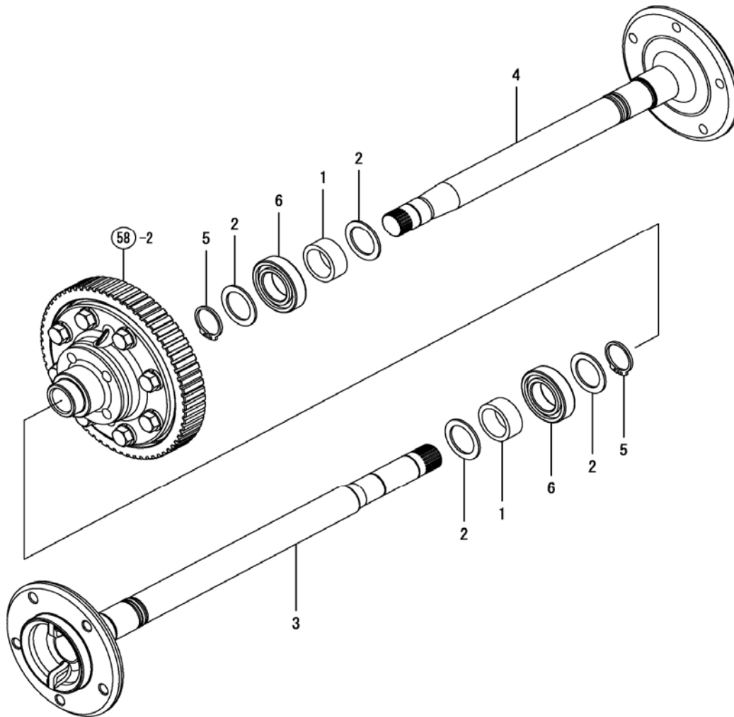
Fig. 62 - Rear Axle Shaft
