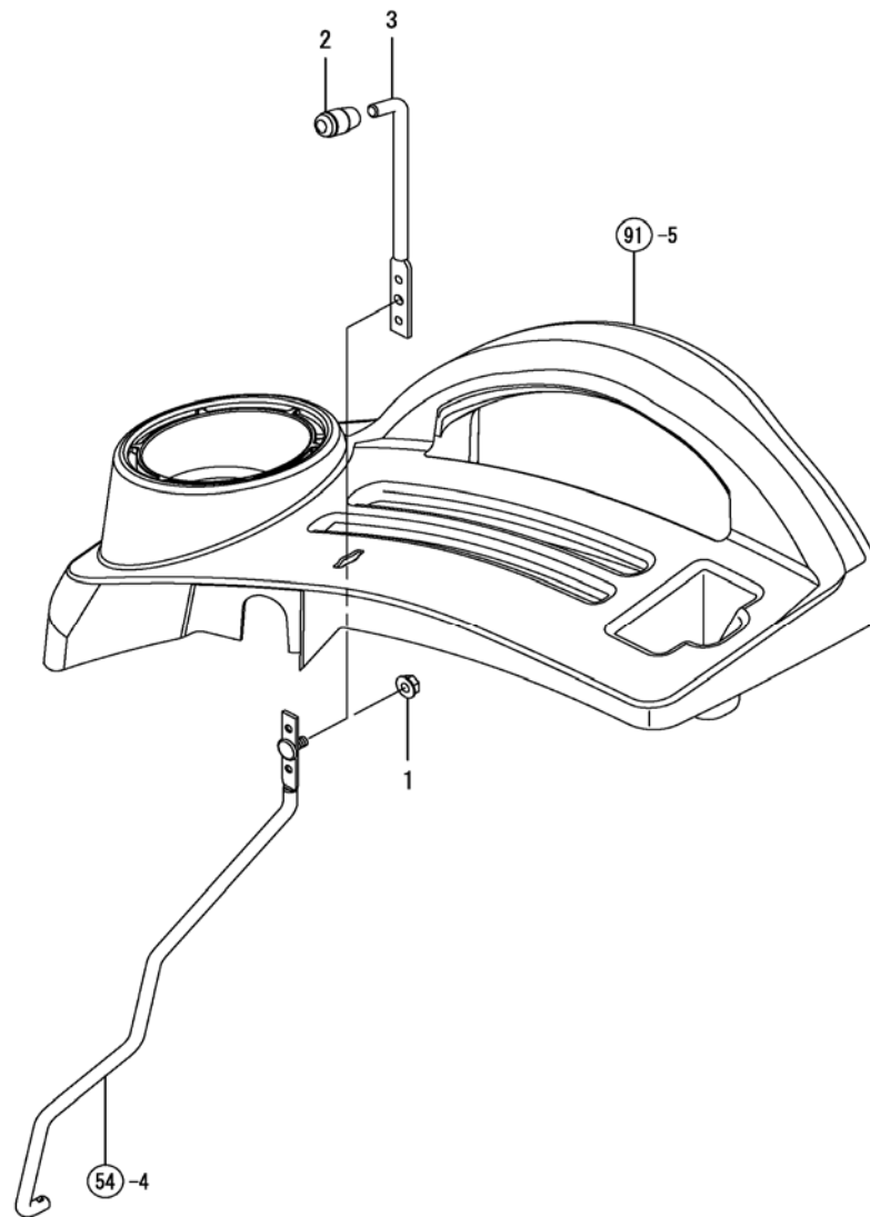
Fig. 55 - Cruise Lever
