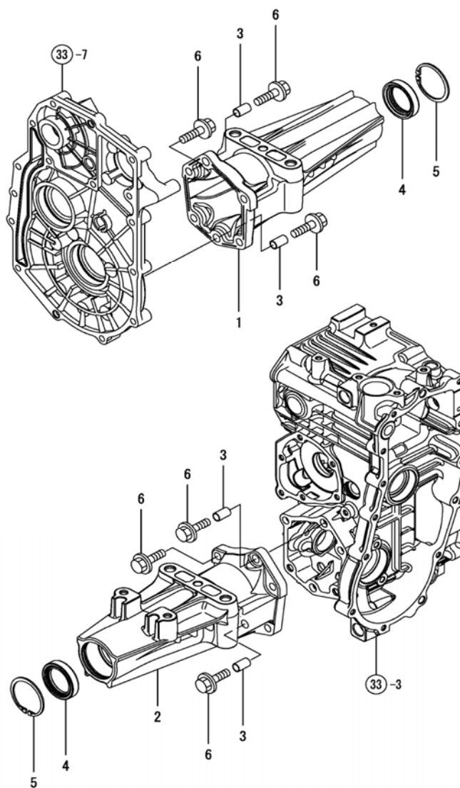
Fig. 59 - Rear Axle Housing
