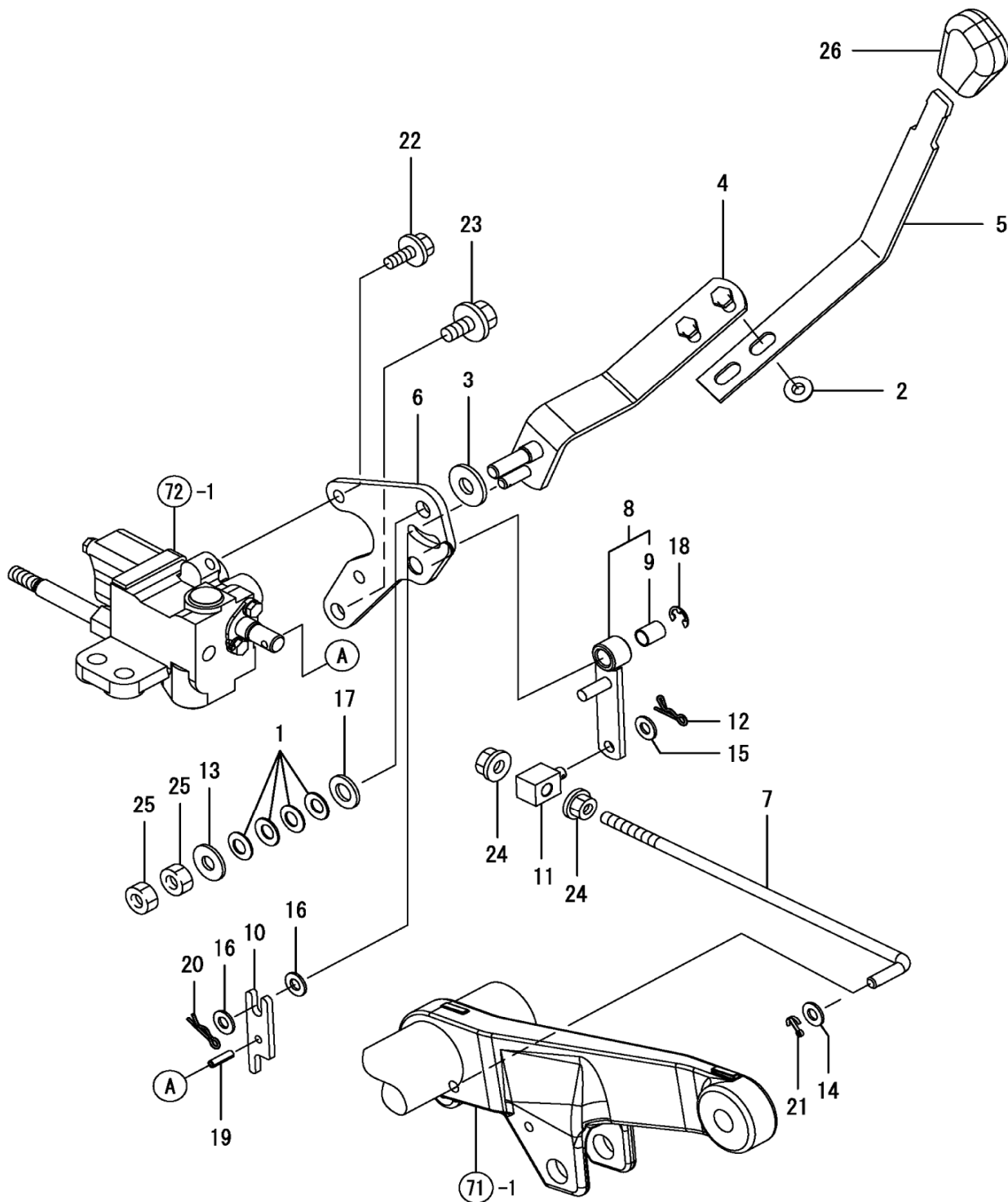
Fig. 76 - Hydraulic Control
