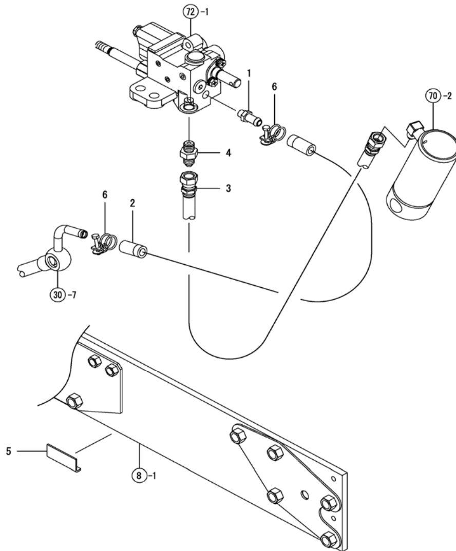
Fig. 77 - Hydraulic Line
