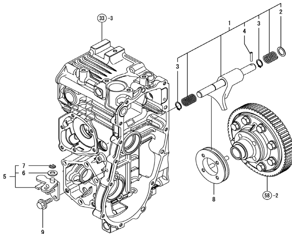
Fig. 60 - Differential Lock
