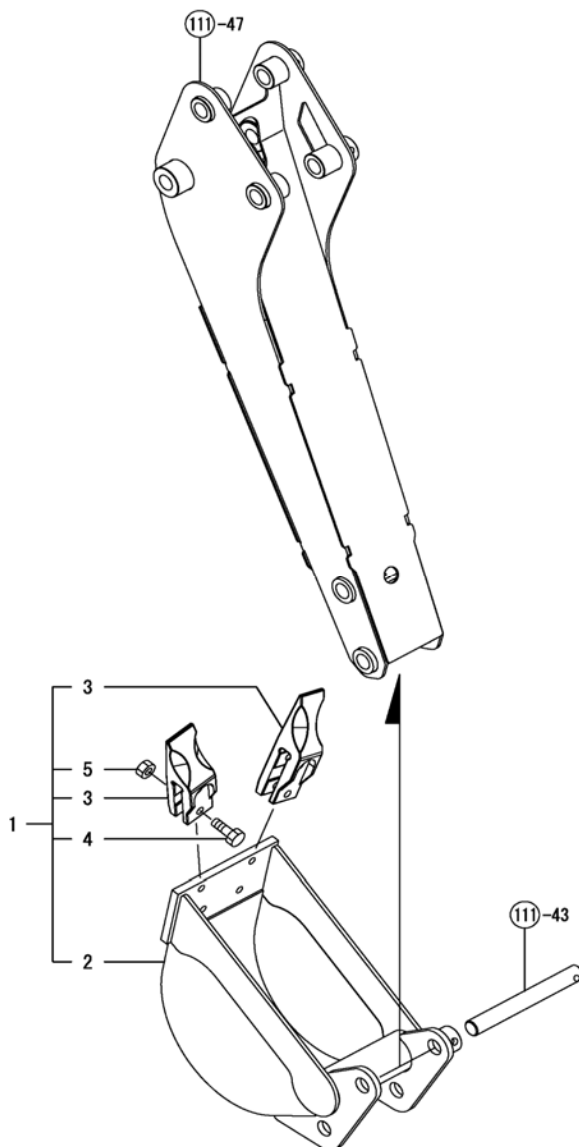
Fig. 115 - Buckets, 8 Inch Kit
