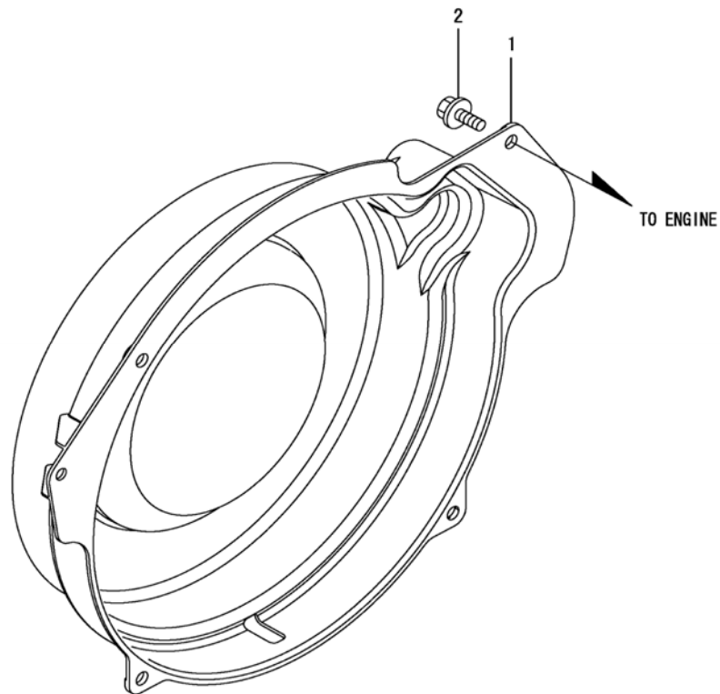
Fig. 1 - Engine Accessories 1
