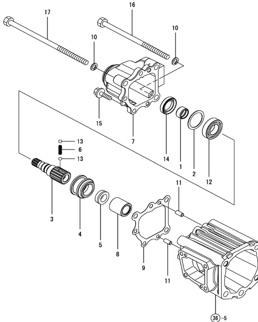
Fig. 50 - Gearbox
