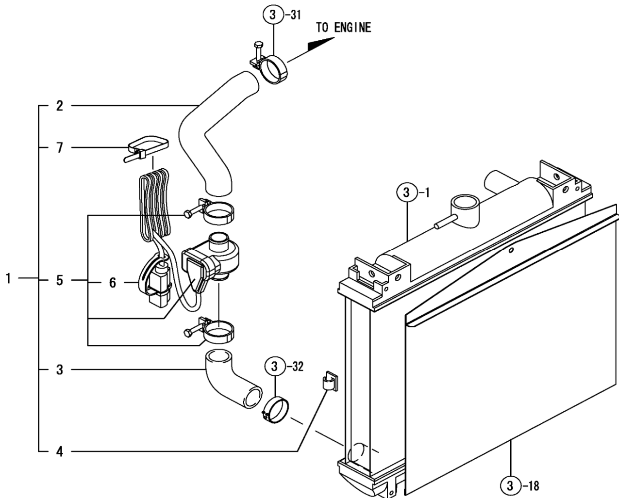
Fig. 110 - Heater, Radiator Hose
