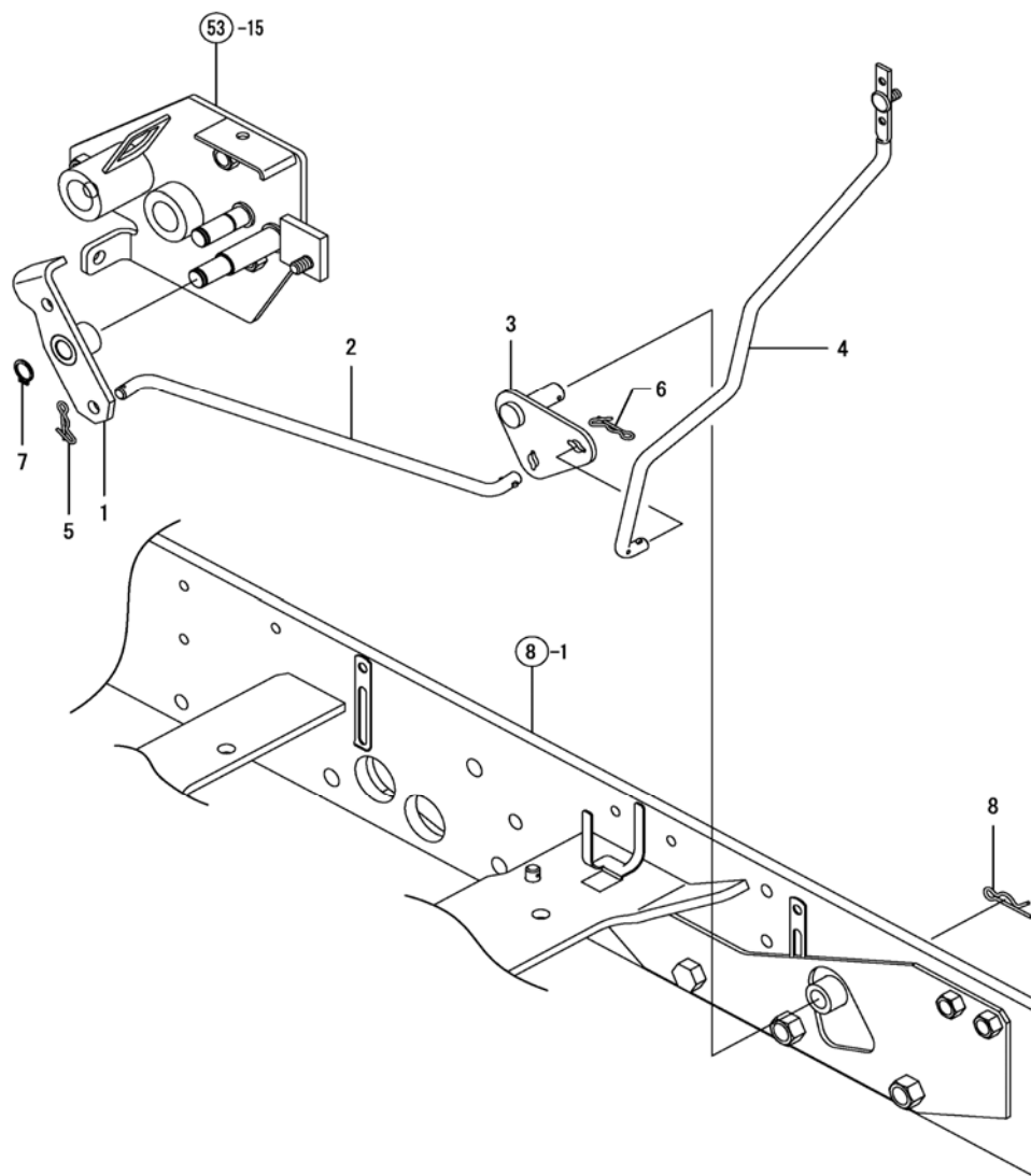
Fig. 54 - Hydrostatic Cruise Link
