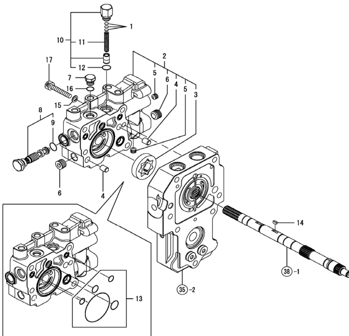
Fig. 43 - Power Pump
