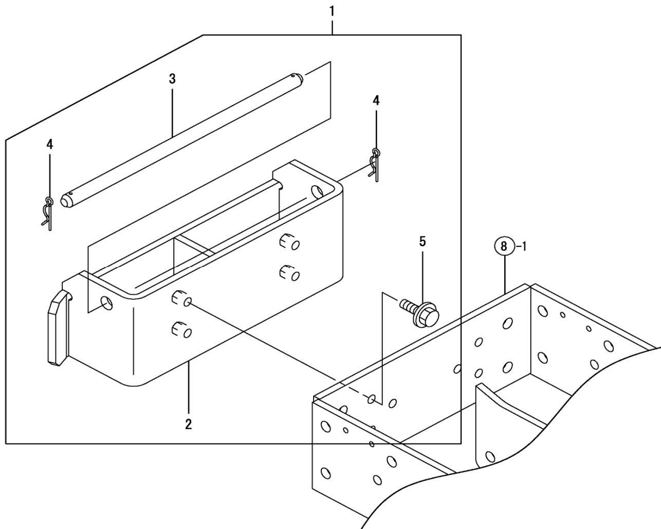
Fig. 108 - Front Hitch
