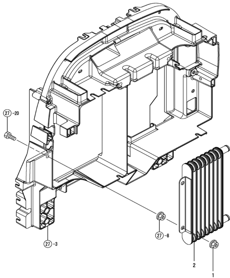
Fig. 78 - Oil Cooler
