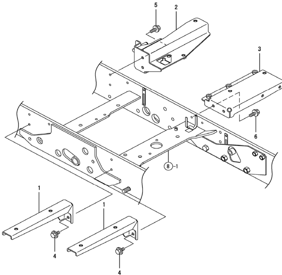
Fig. 92 - Footrest Stay
