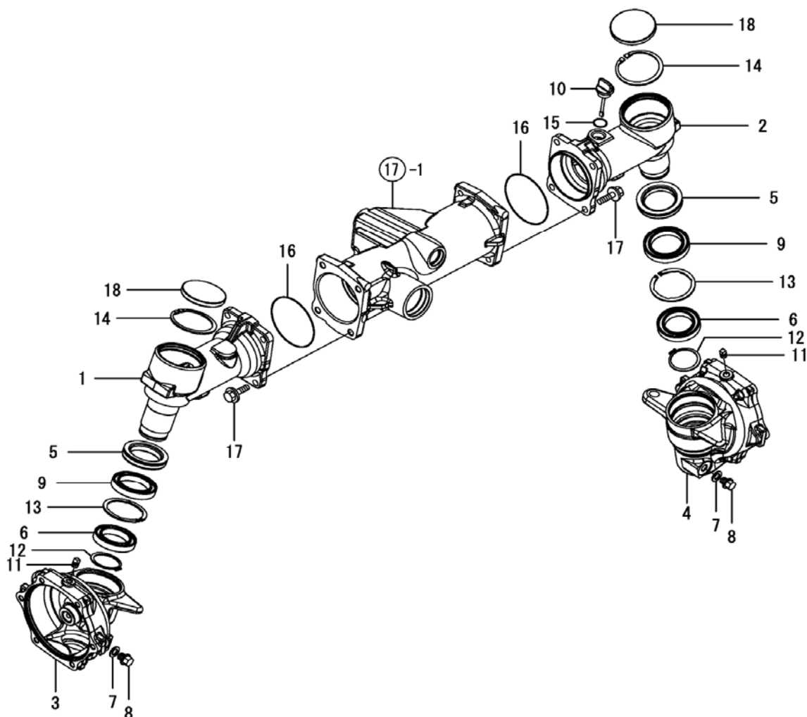
Fig. 18 - Case, Front Gear
