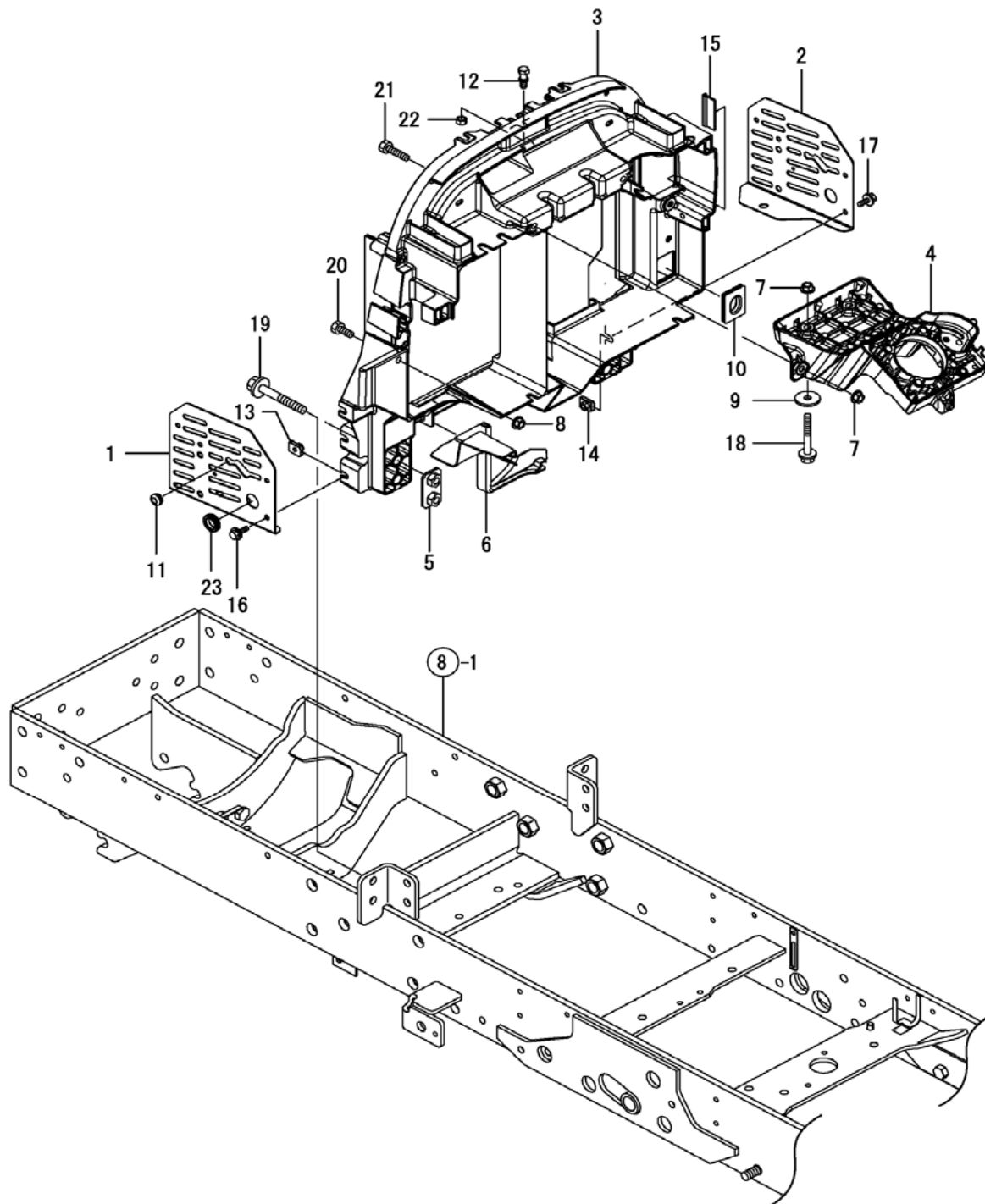
Fig. 27 - Column Bracket
