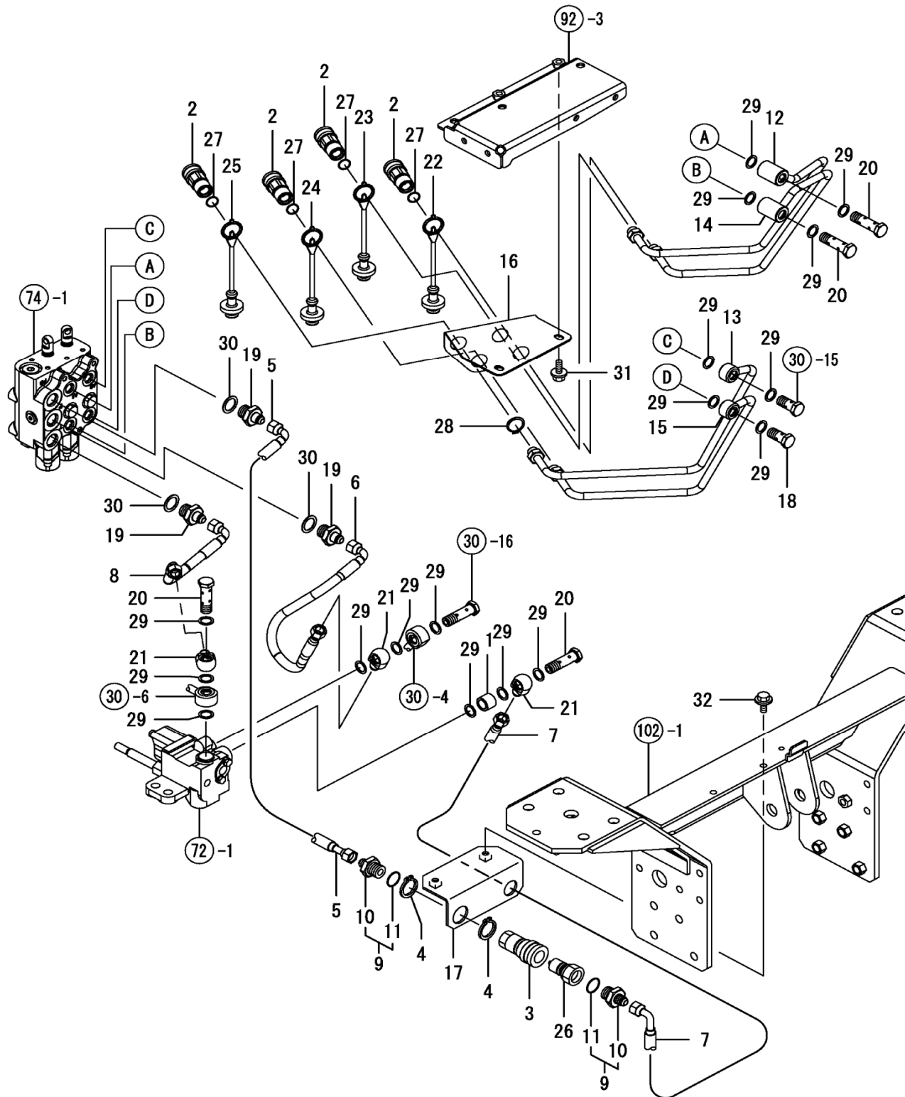
Fig. 79 - Piping
