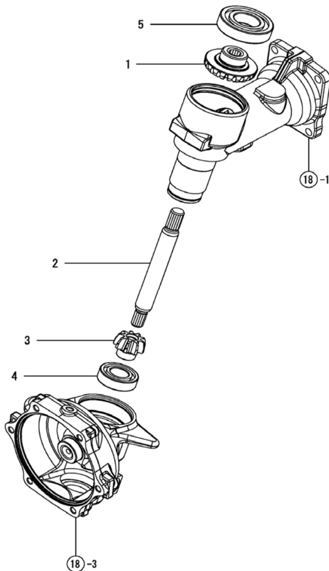
Fig. 19 - Front Shaft
