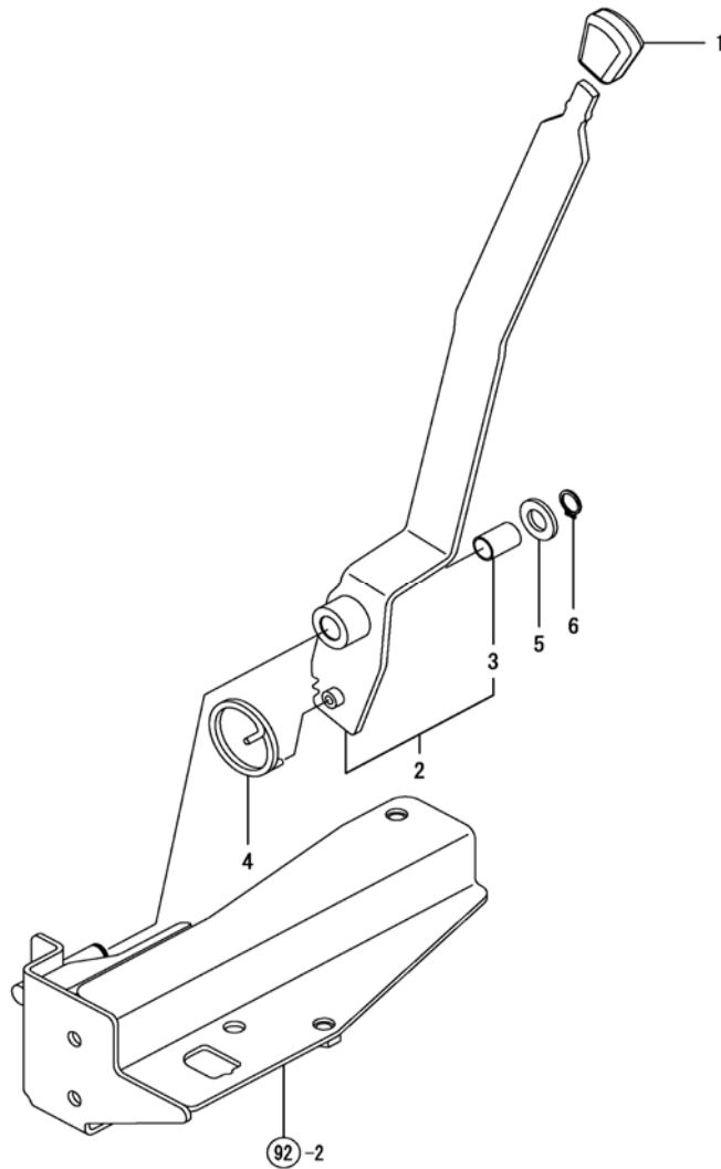
Fig. 69 - Parking Brake
