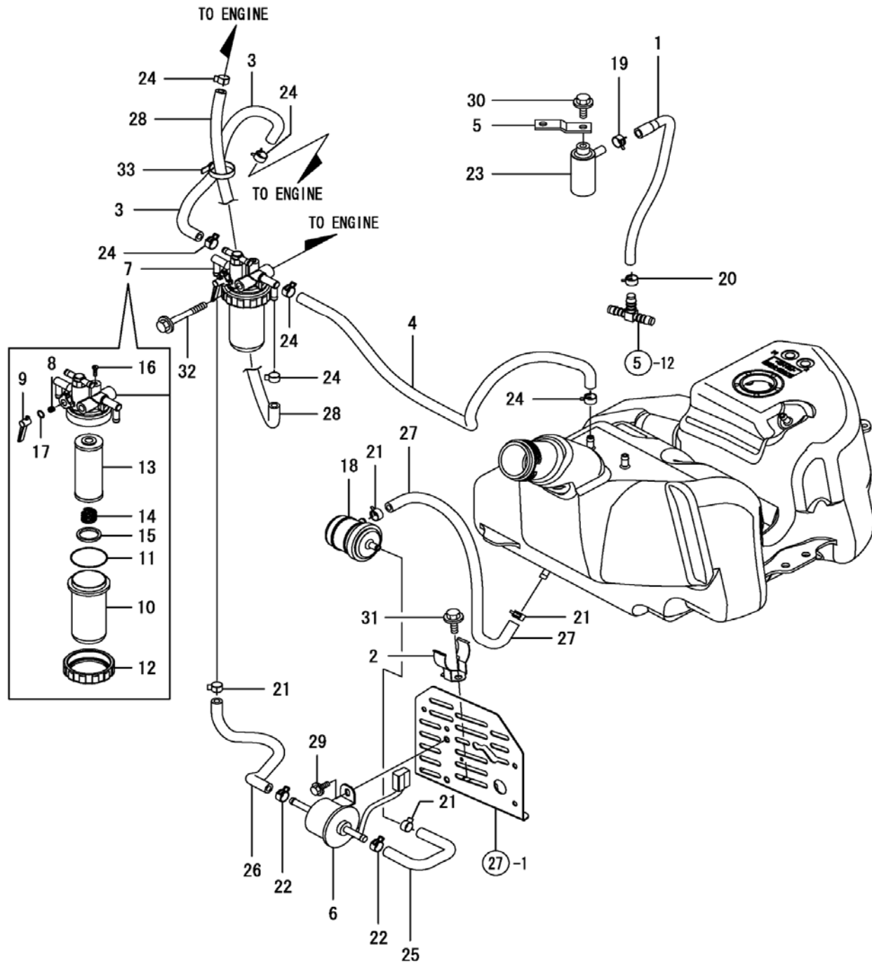
Fig. 7 - Fuel Pipe
