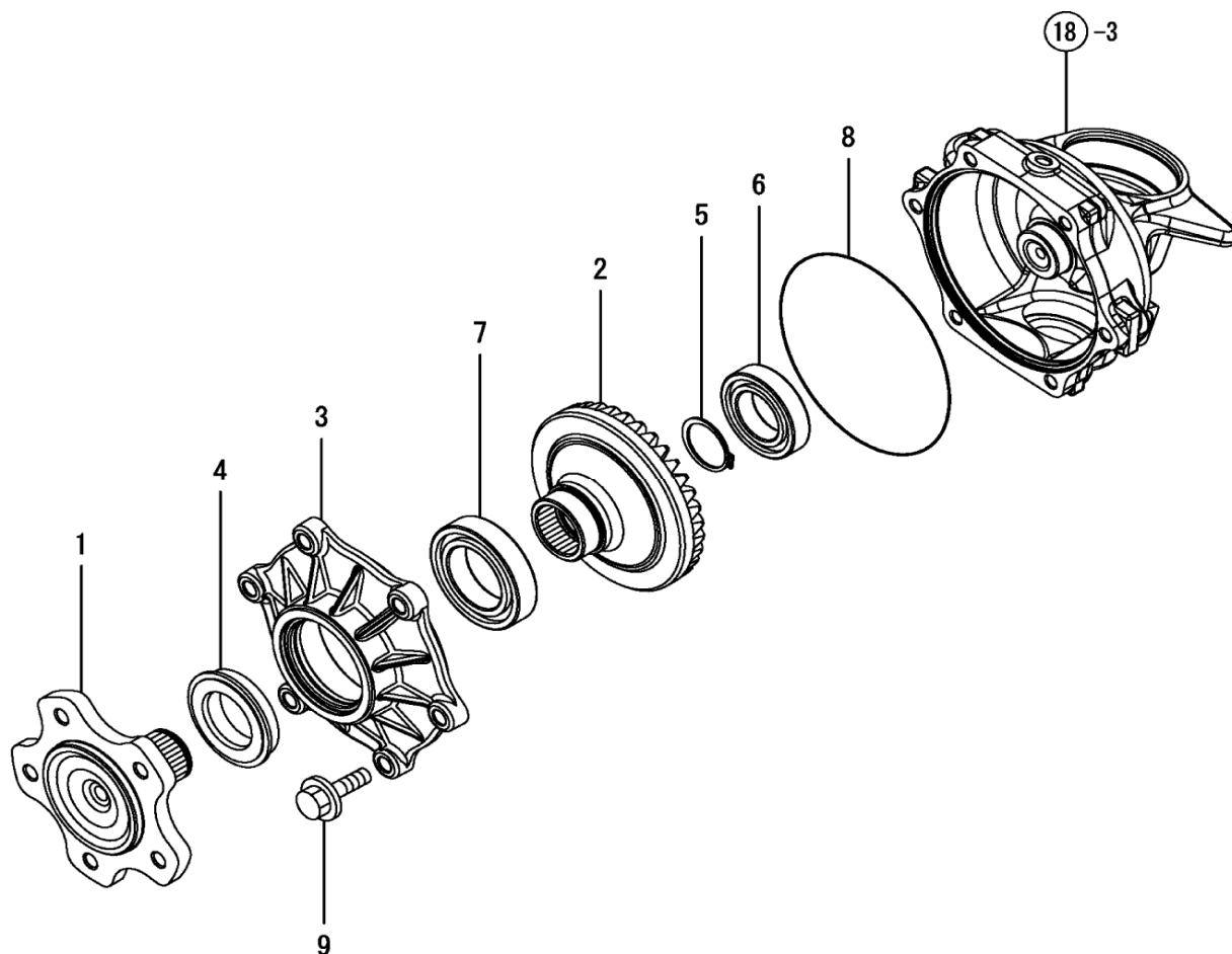
Fig. 20 - Front Spindle
