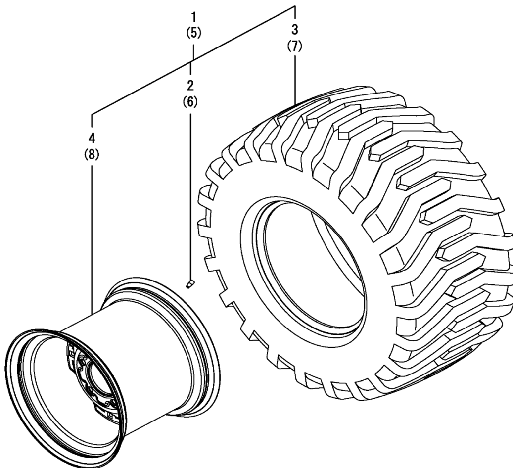
Fig. 65 - Tire, Rear (Industrial)
