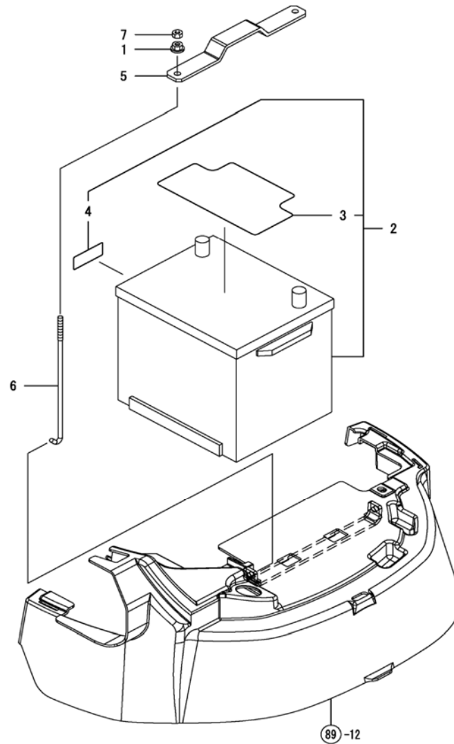
Fig. 81 - Battery
