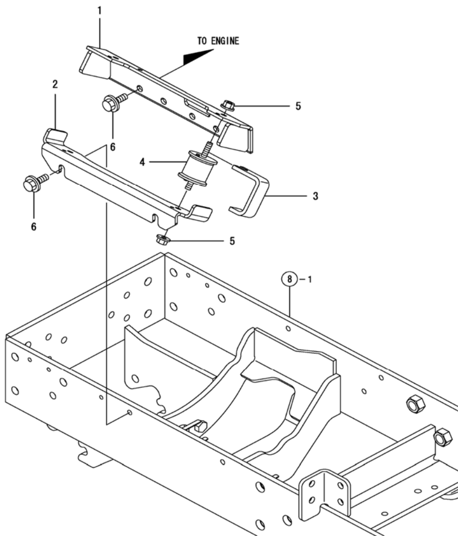
Fig. 10 - Engine Mount
