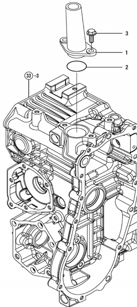
Fig. 32 - Oil Gauge Tube
