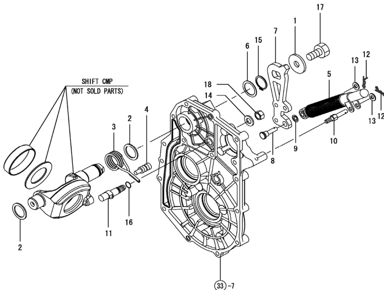
Fig. 48 - Control
