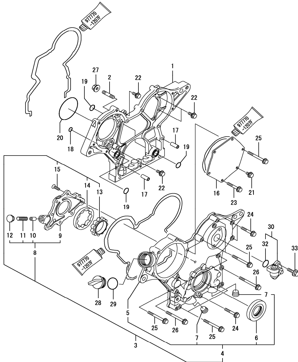
FIG. 2. GEAR HOUSING
