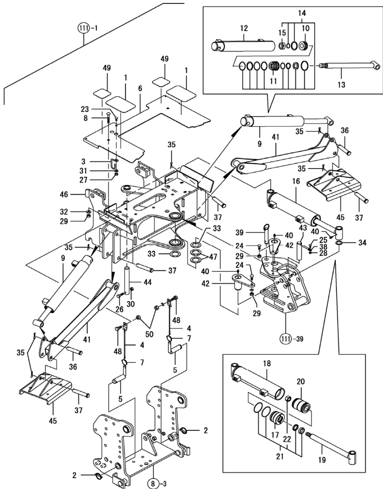
Fig. 113 - Backhoe, Main Frame
