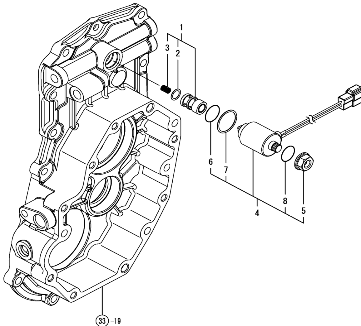
Fig. 44 - Solenoid Valve
