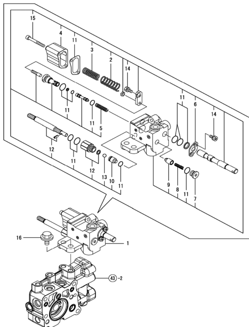
Fig. 72 - Control Valve
