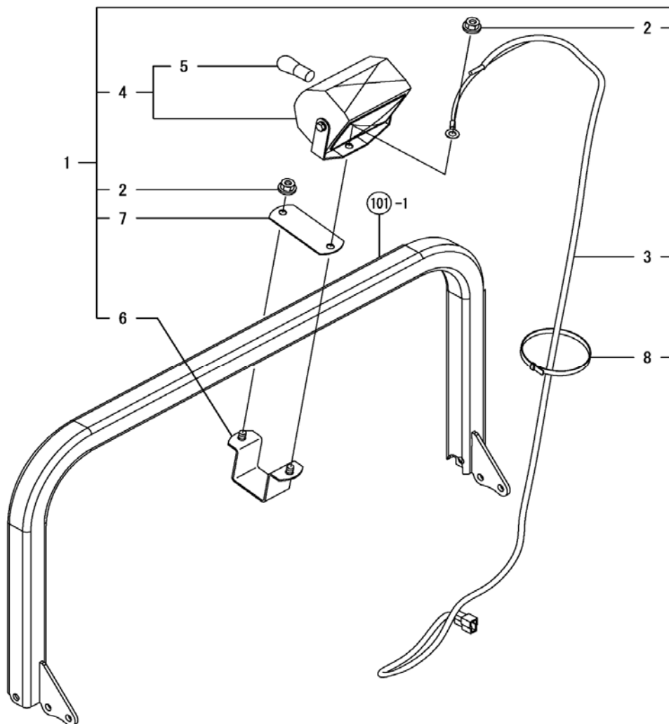
Fig. 109 - Work Lamp
