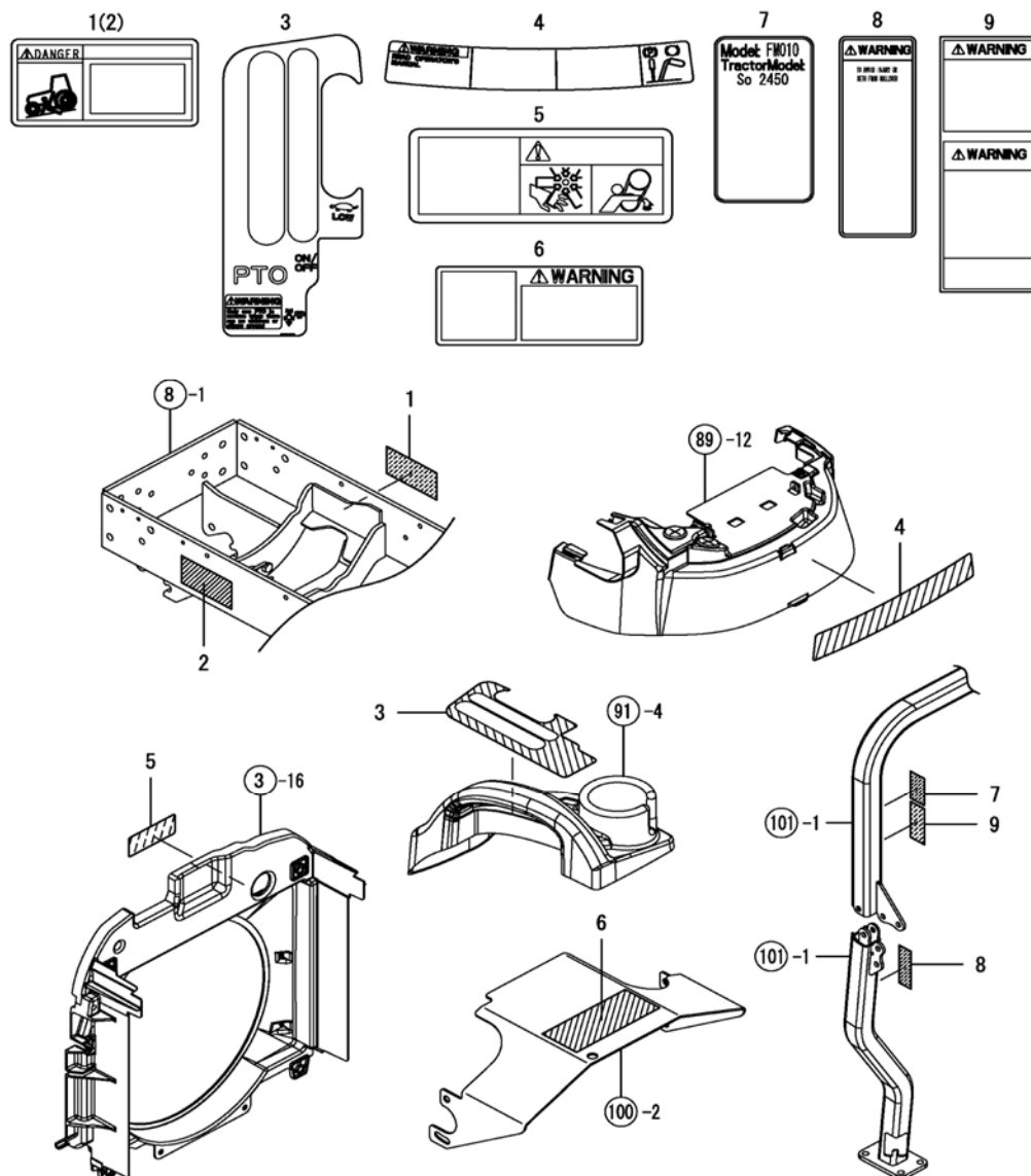
Fig. 99 - Label, Safety
