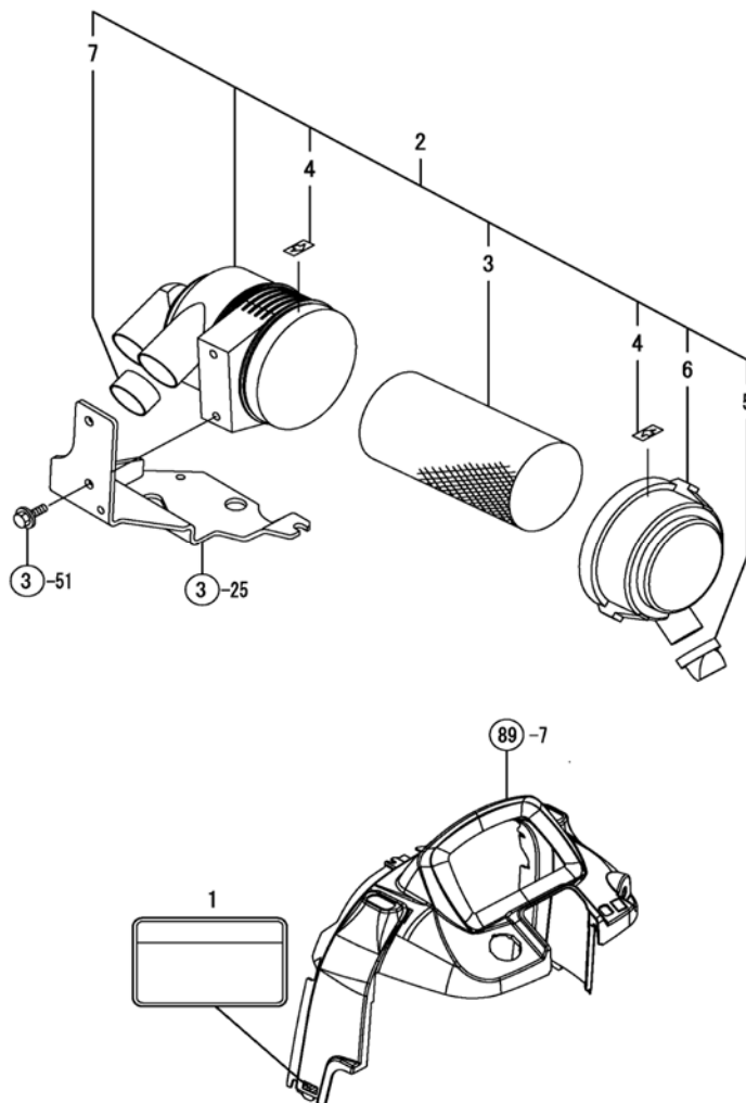
Fig. 2 - Engine Accessories 2
