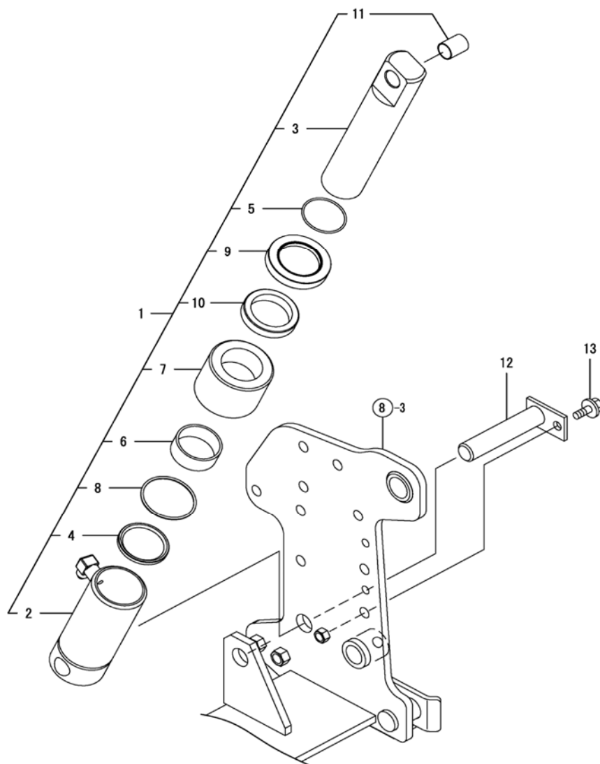
Fig. 70 - Lift Cylinder
