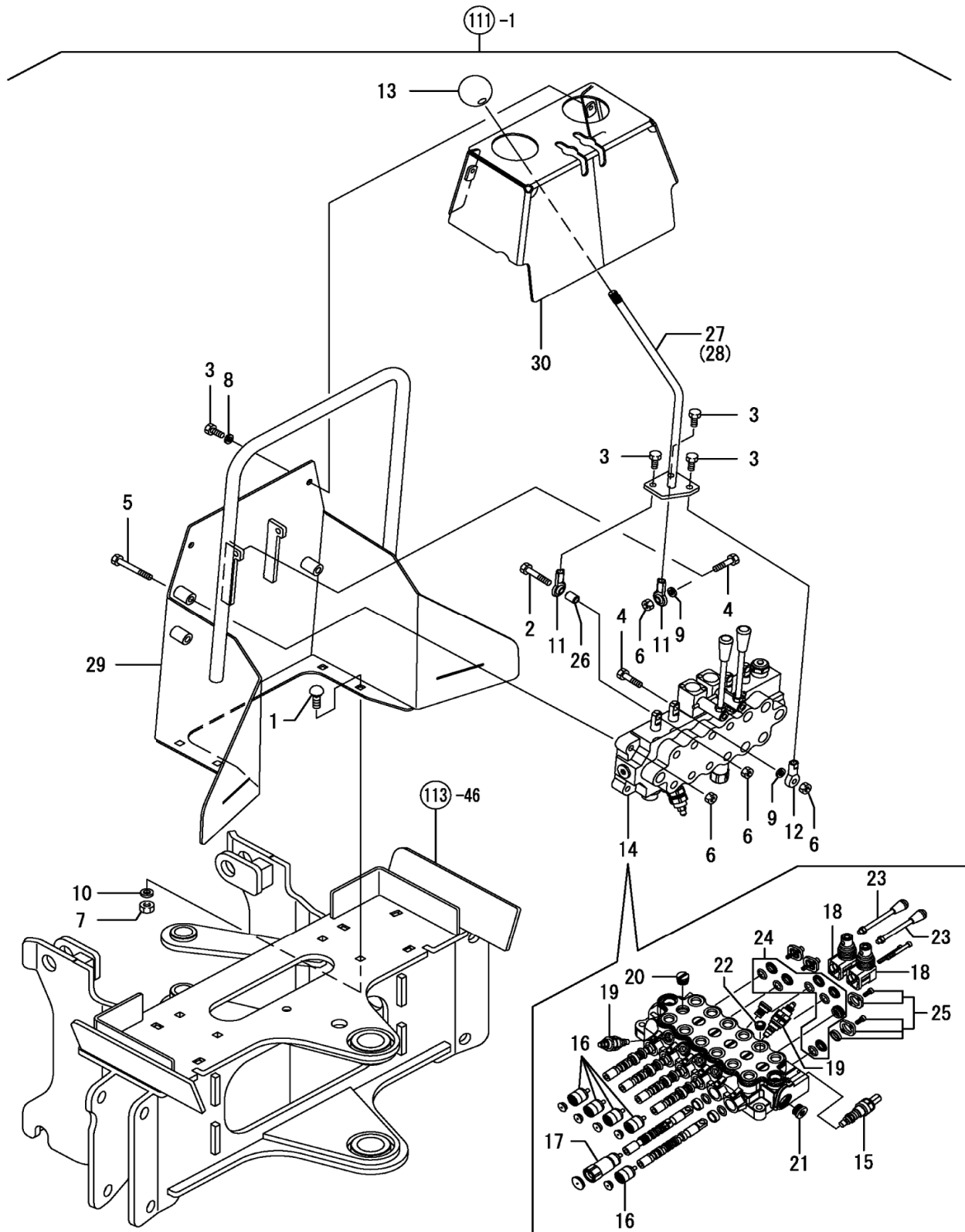
Fig. 112 - Backhoe, Control
