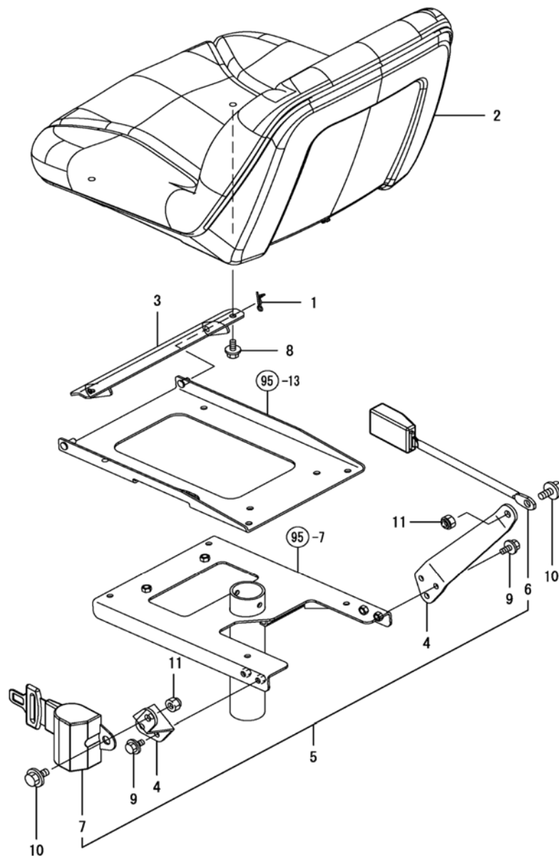
Fig. 94 - Driver Seat
