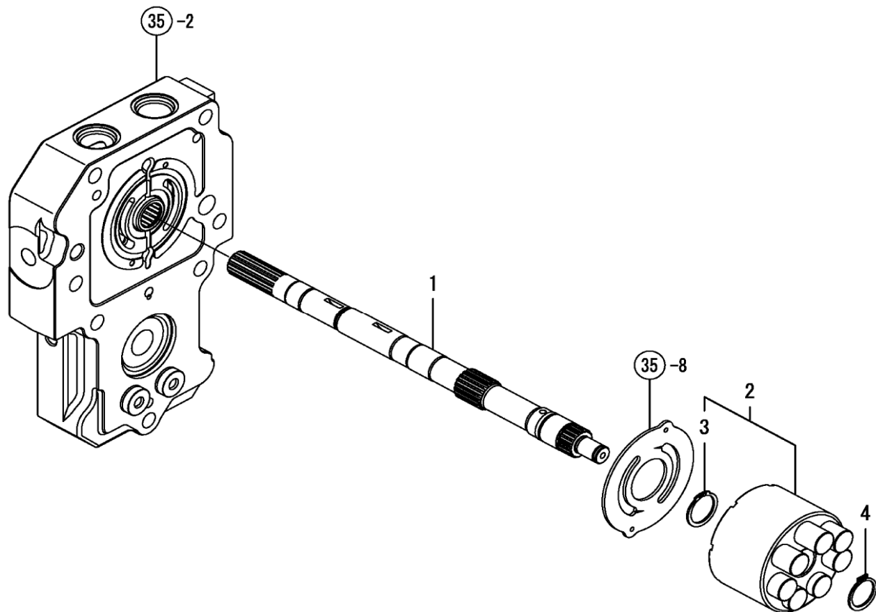
Fig. 38 - Pump
