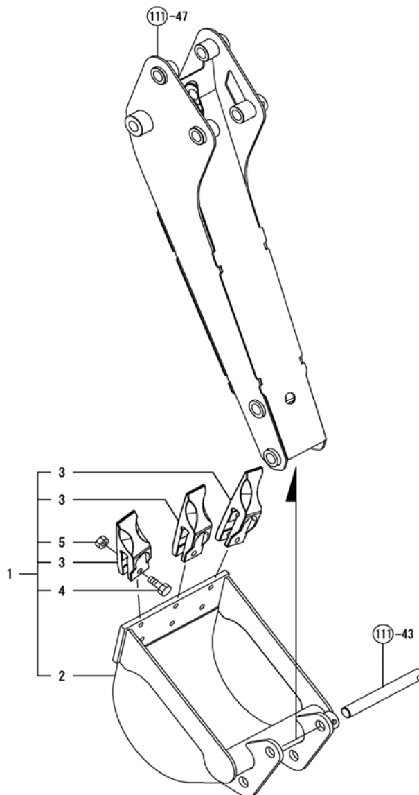
Fig. 116 - Buckets, 12 Inch Kit
