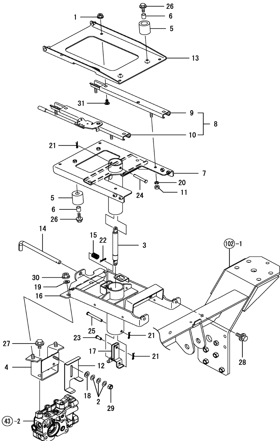
Fig. 95 - Seat Stay
