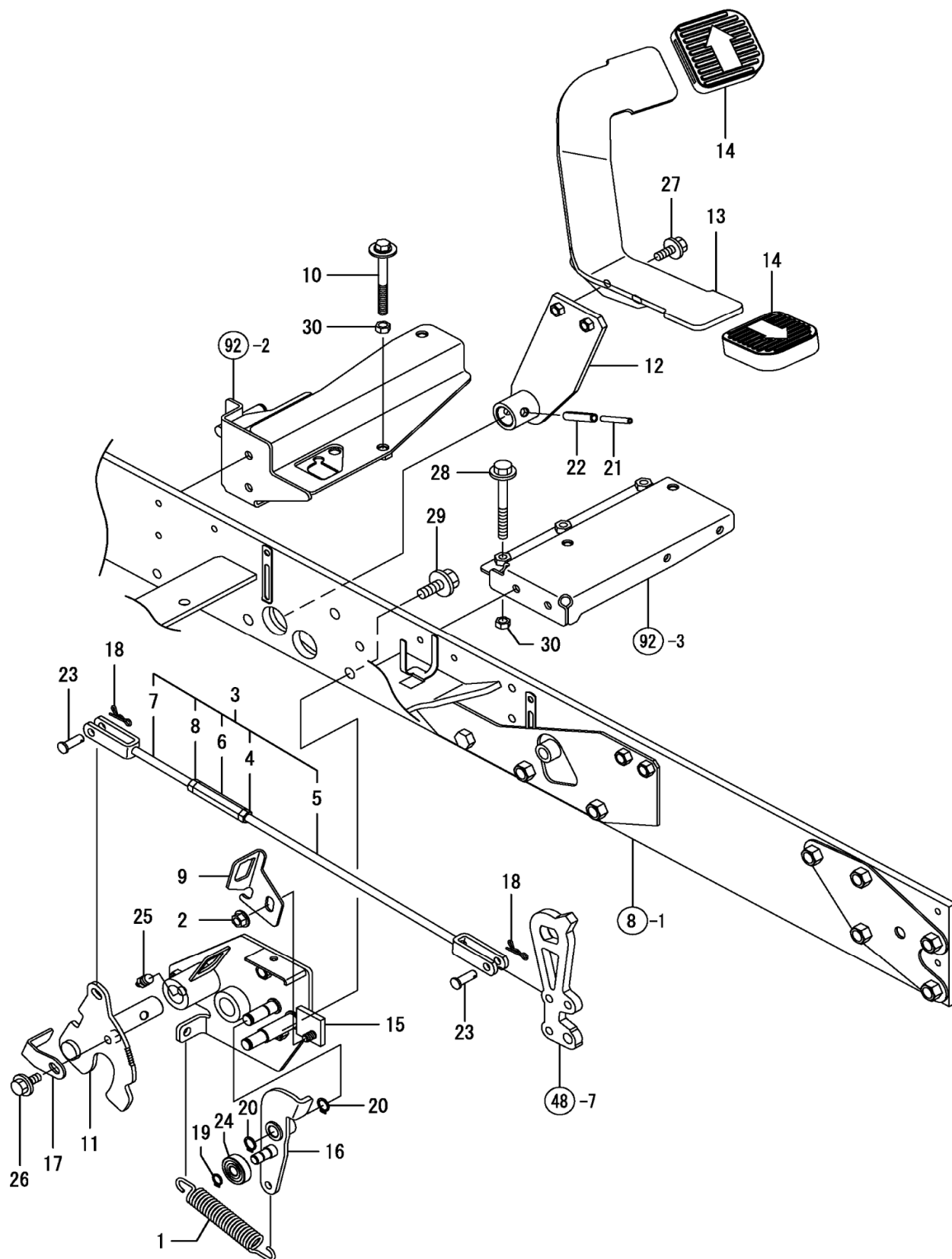
Fig. 53 - Hydrostatic Pedal
