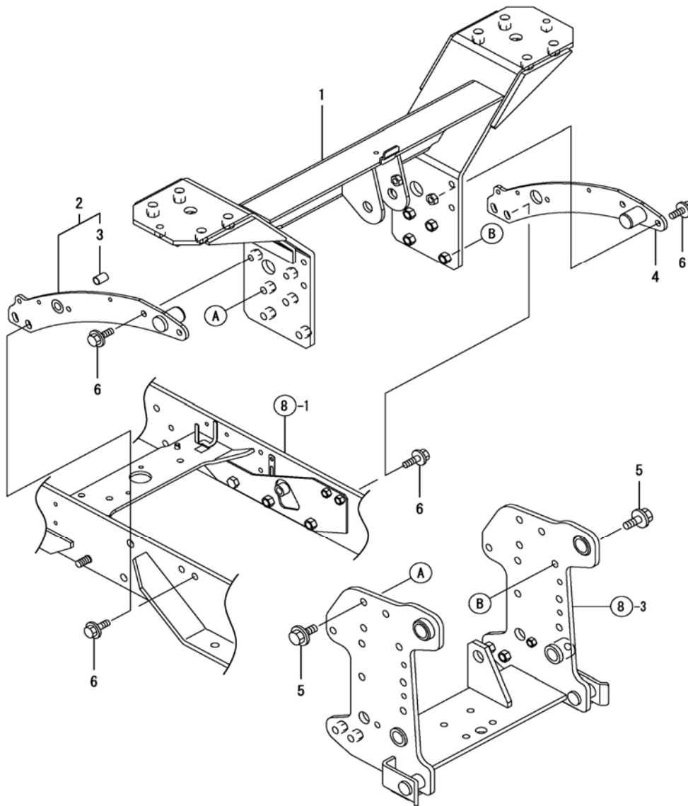
Fig. 102 - Lower Frame
