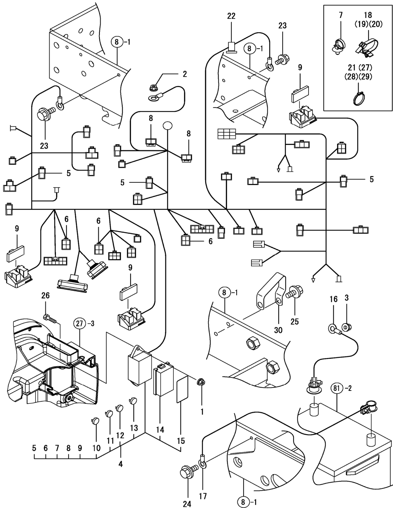
Fig. 80 - Wire Harness
