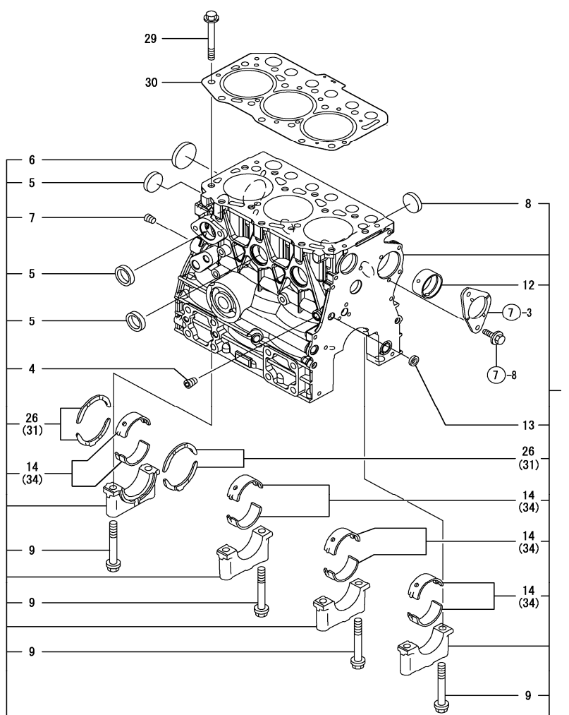
FIG. 1. CYLINDER BLOCK
