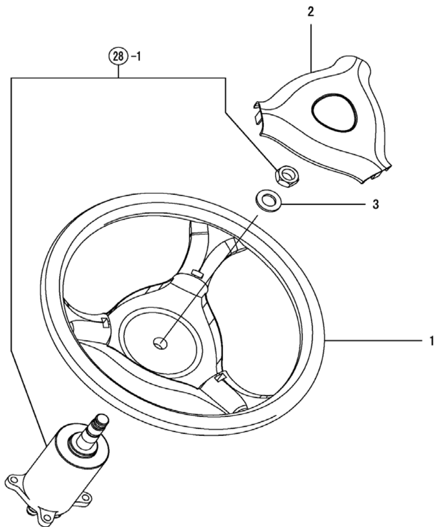
Fig. 26 - Steering Wheel
