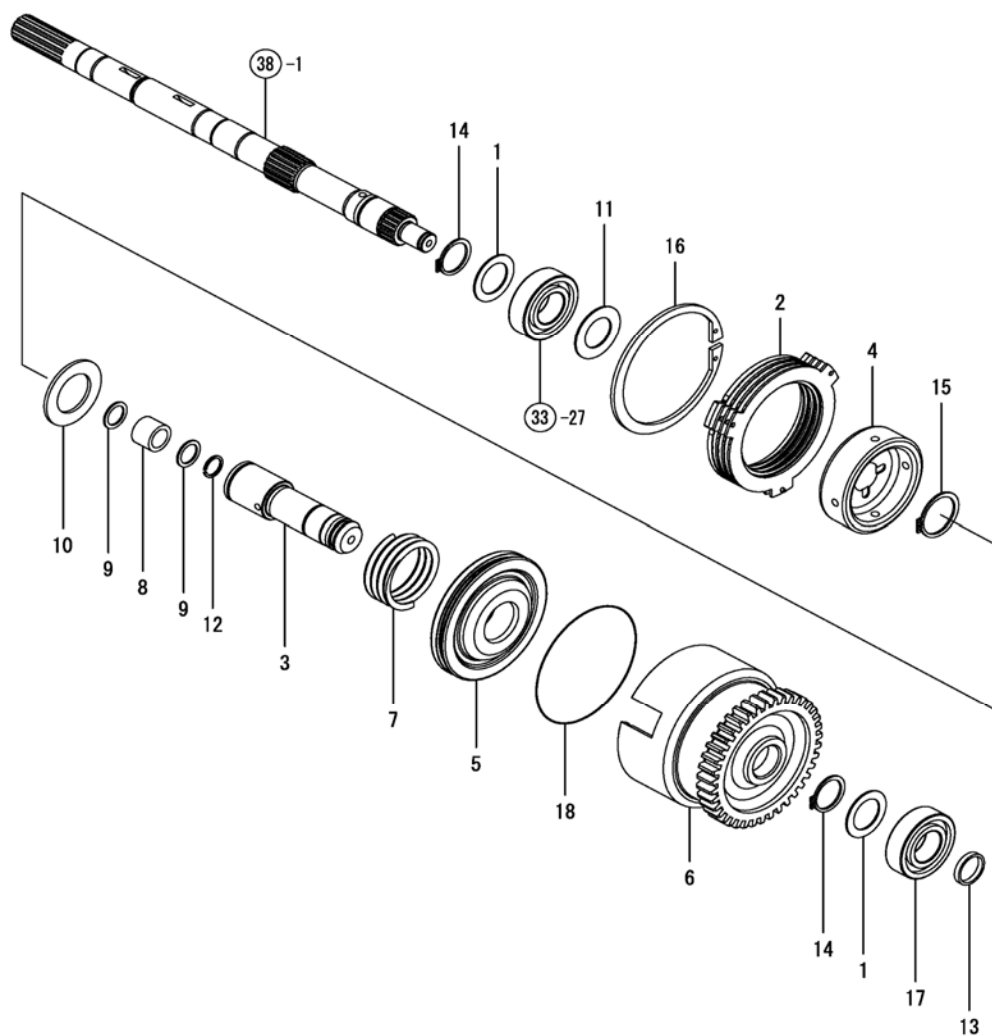
Fig. 40 - Clutch Shaft
