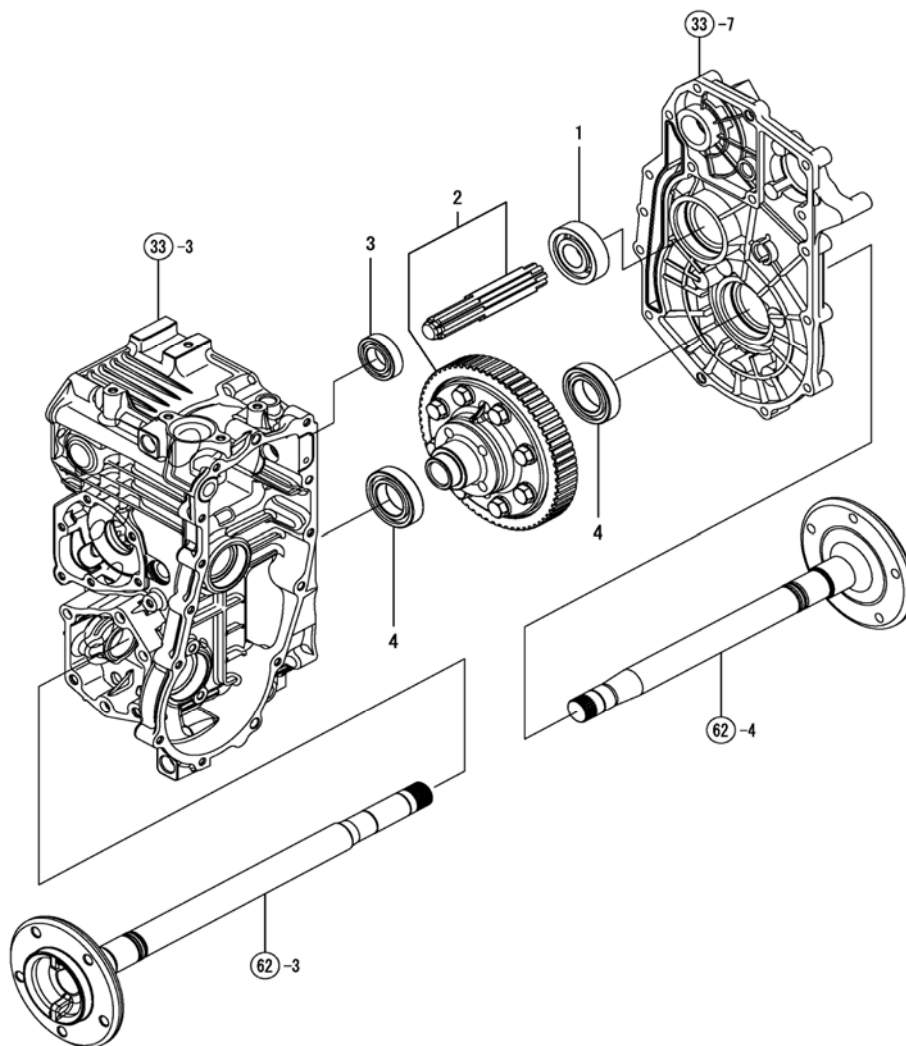
Fig. 58 - Differential Gear, Rear
