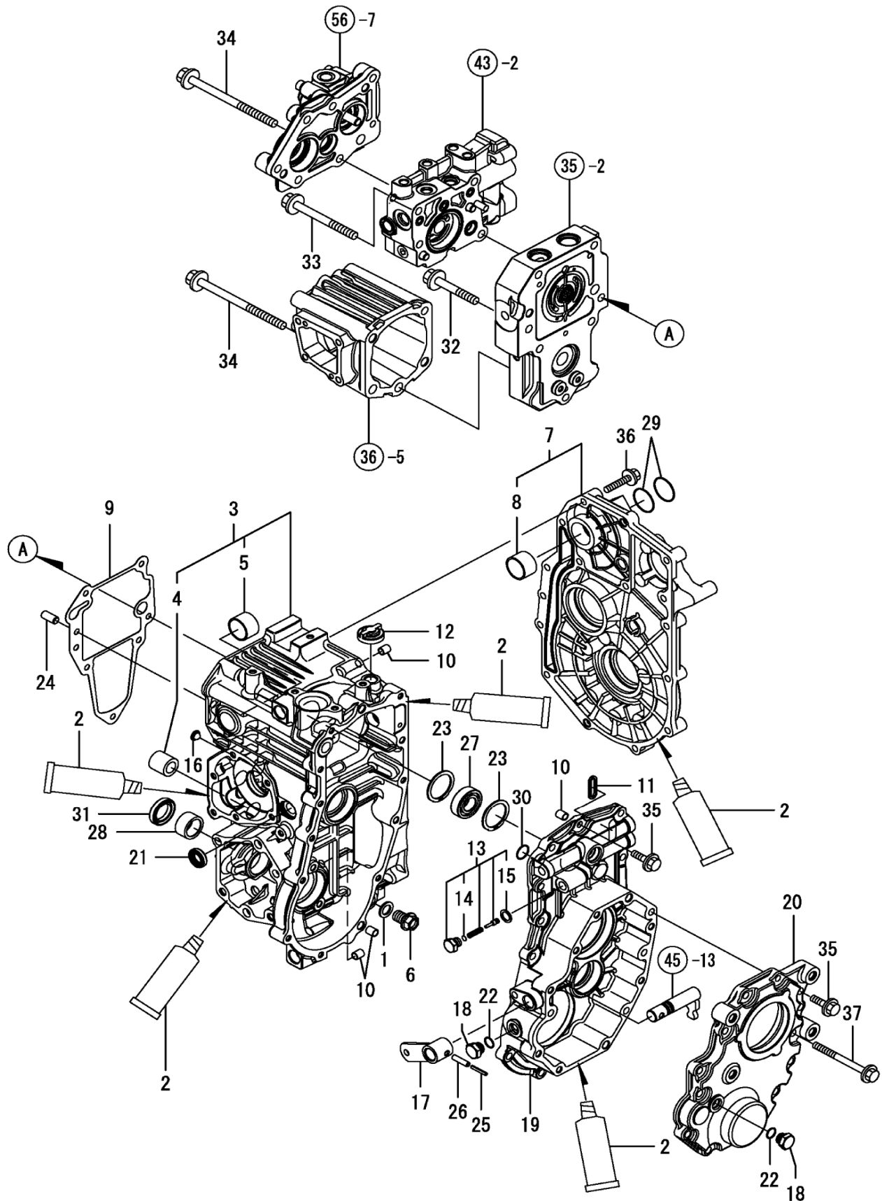
Fig. 33 - Transaxle Case
