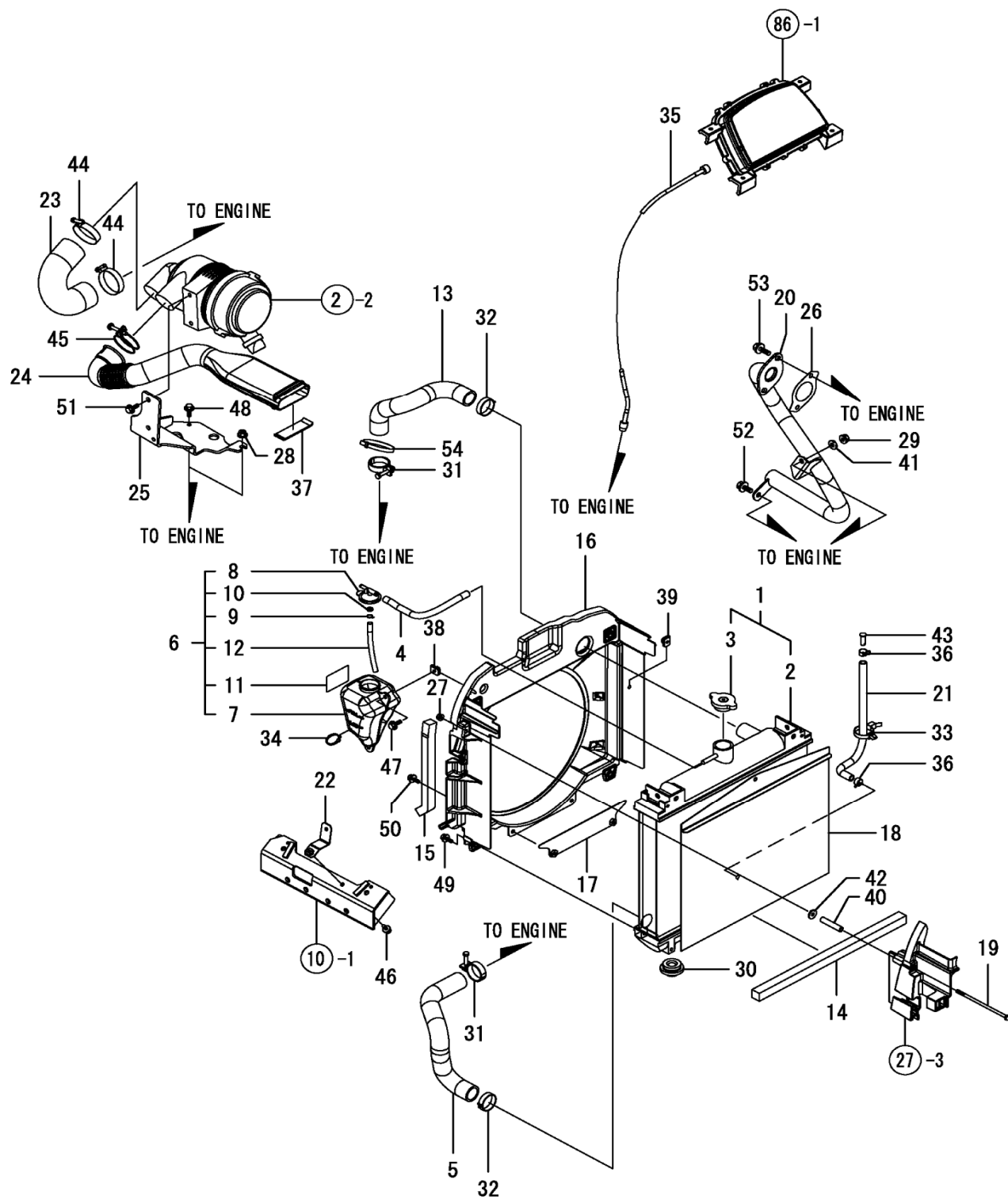
Fig. 3 - Engine Accessories 3
