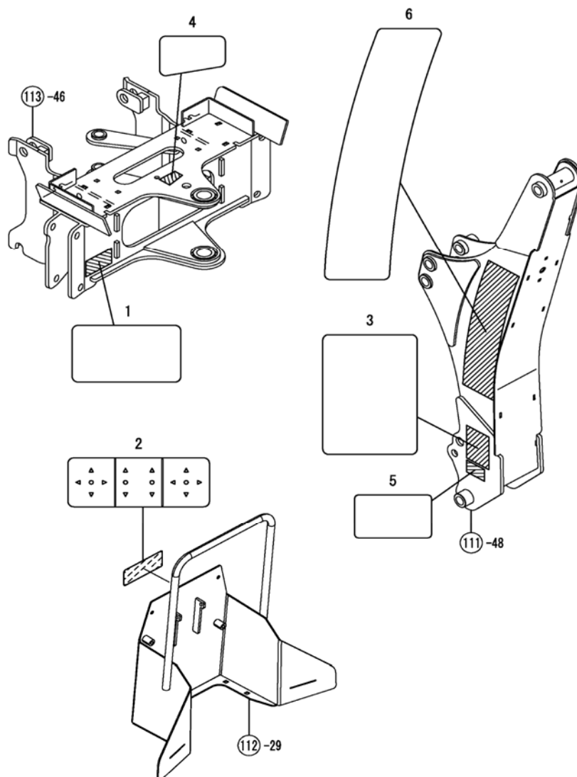
Fig. 118 - Backhoe, Label
