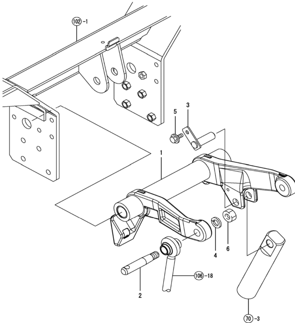
Fig. 71 - Lift Arm
