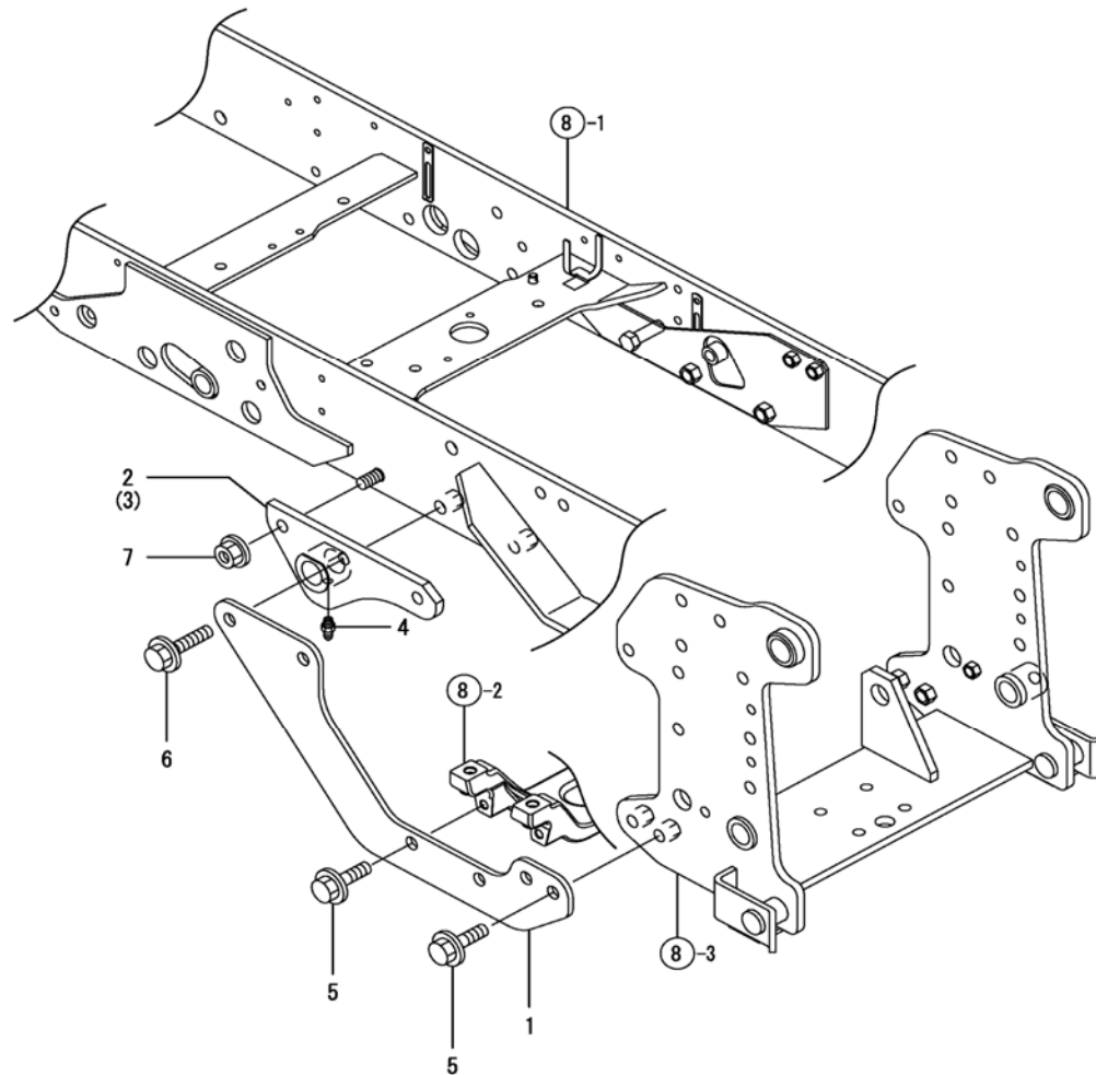
Fig. 9 - Frame, Joint
