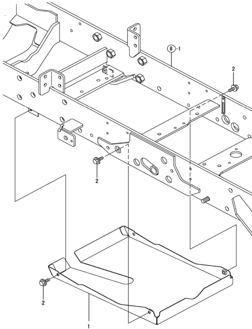
Fig. 6 - Fuel Tank Cover
