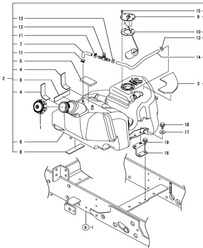
Fig. 5 - Fuel Tank
