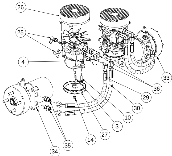
Pump & Motor Systems
