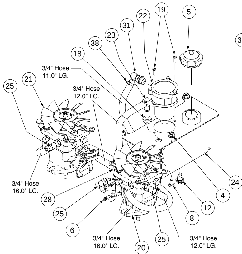
Pilot & Drain Systems
