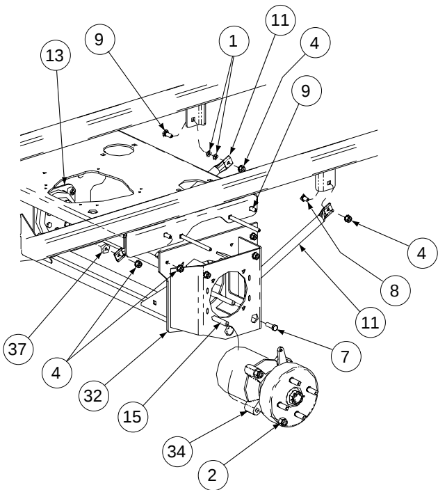
Motor Mount Systems
