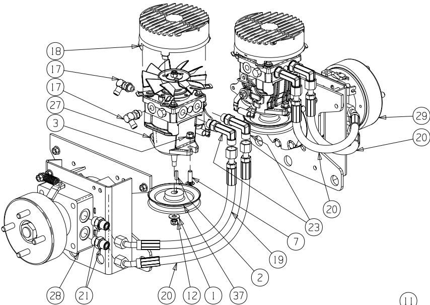
Pump & Motor Systems
