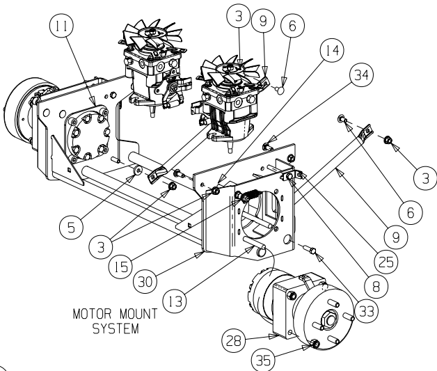
Motor Mount Systems
