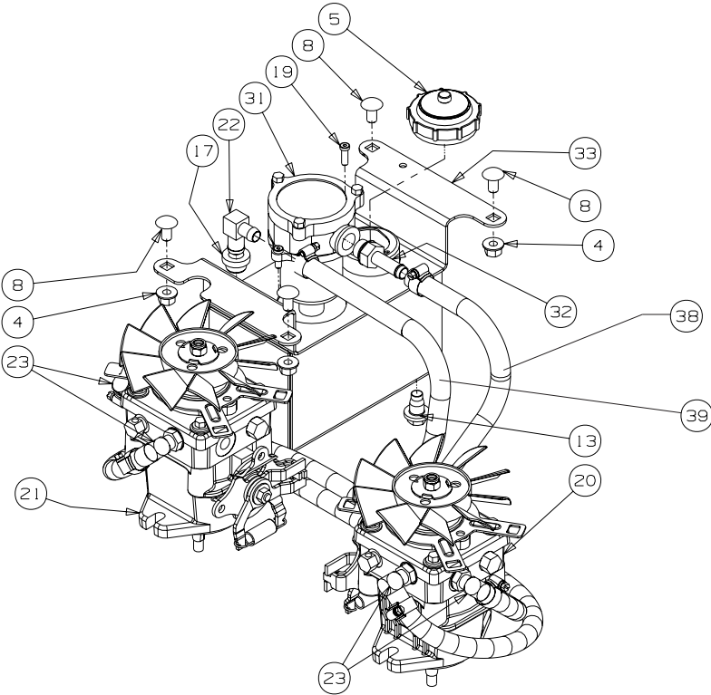
Pilot & Drain Systems
