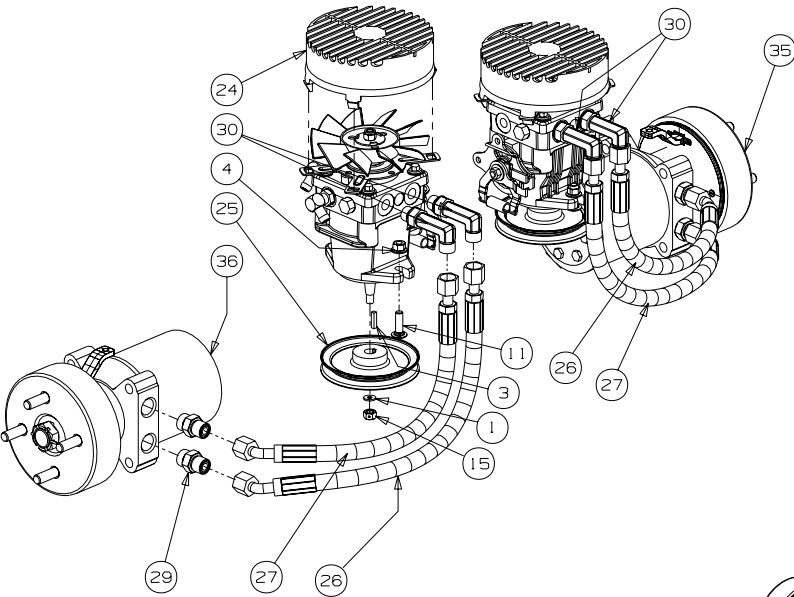
Pump & Motor Systems
