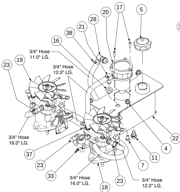
Pilot & Drain Systems
