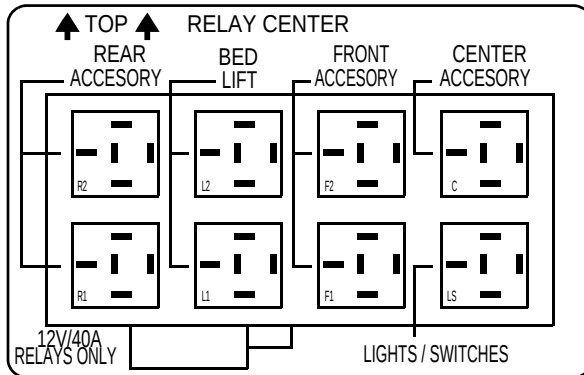
Relay Center
