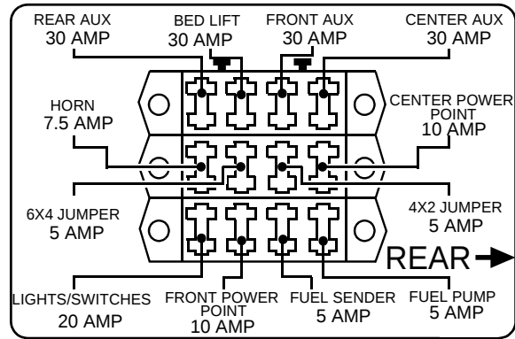
Fuse Box
