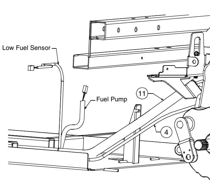
GAS/FUEL PUMP VIEW
