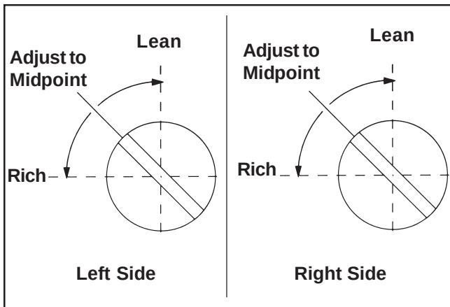
Figure 19. Optimum Low Idle Fuel Settings.
