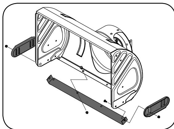
Figure 18B - Reversible Skid Shoe
