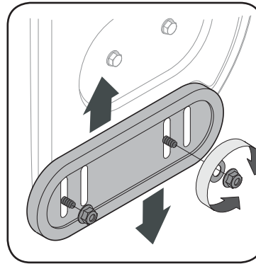
Figure 5-6 - Plastic Reversible
