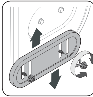
Figure 5-6 - Plastic Reversible
