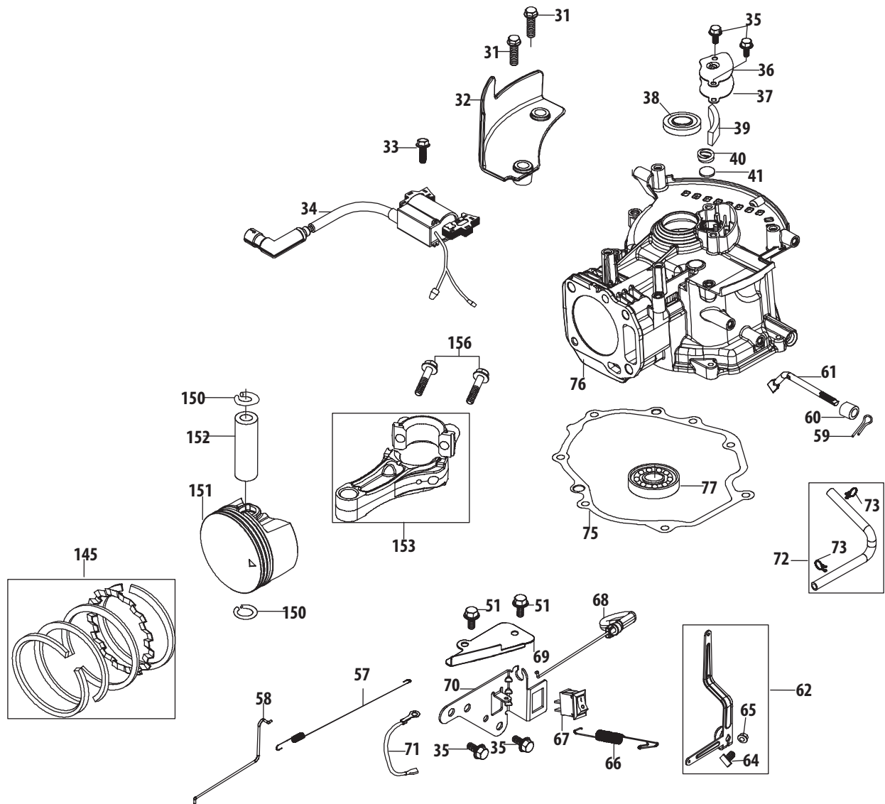
160 - Complete Engine
