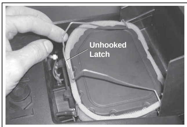
Figure 12. Unhooking Latch.
