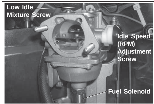
Figure 15. Carburetor.
