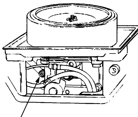
IDLE SPEED ADJUSTING SCREW AND SPRING
