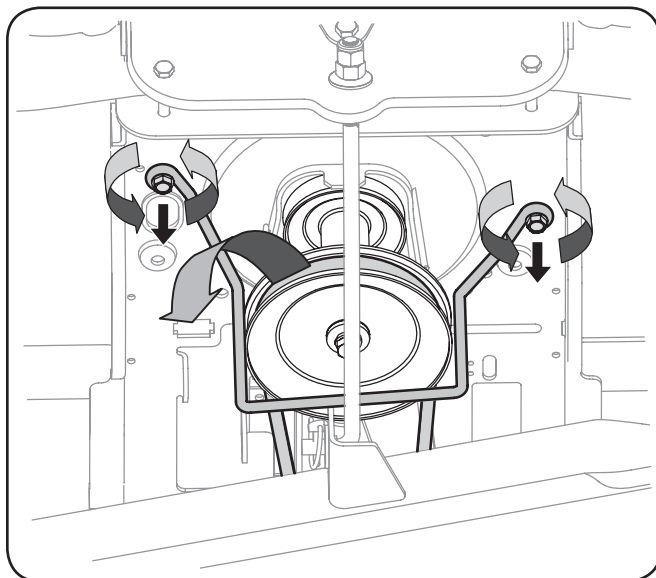
Figure 7-1 (Manual PTO shown)
