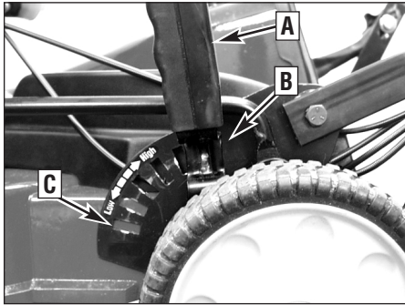
Figure 4-6: Cutting height adjustment.
