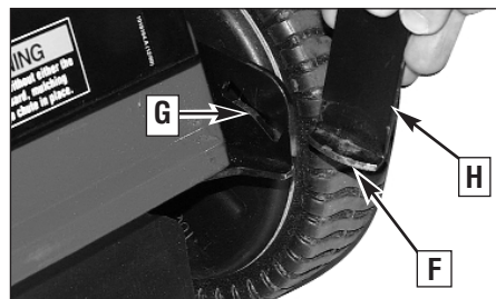
Figure 2-3: Assembling handlebar. (Right-side handlebar strut shown.)
