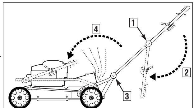
Figure 5-16: Folding the mower for storage.
