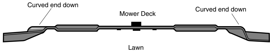
Figure 5-4: Correct blade installation.
