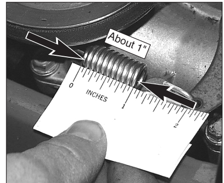
Figure 5-9: First measurement with drive clutch spring disengaged.
