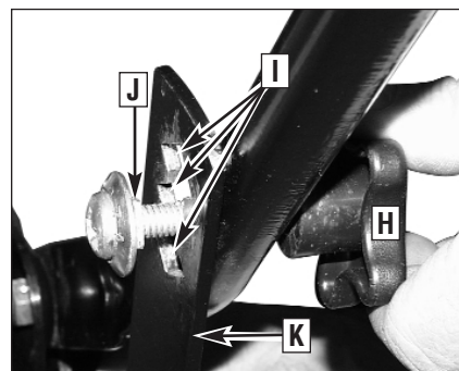
Figure 4-5: Adjusting handlebar height.
