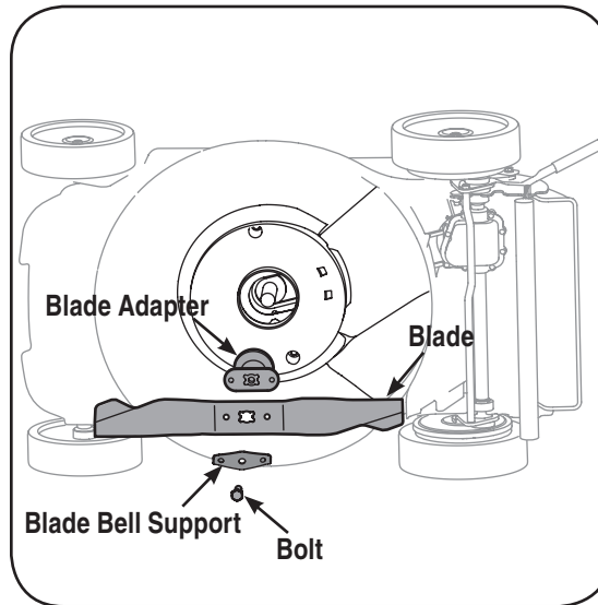
Figure 5-3: Remove the bolt and blade bell support to access the blade.
