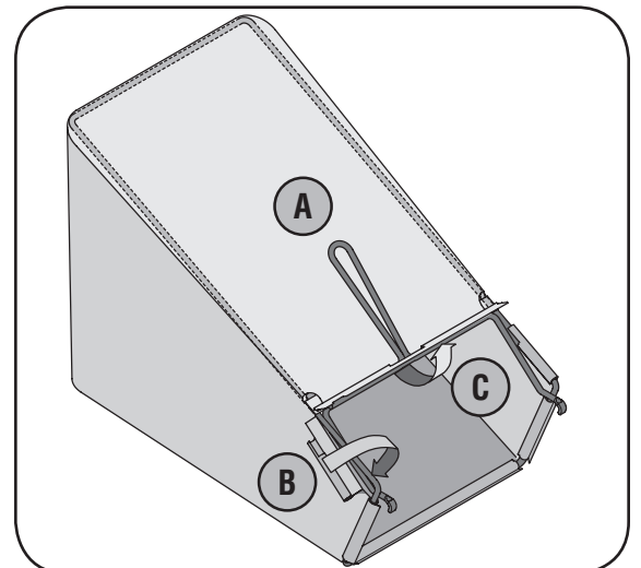
Figure 3-4: Assemble the grass catcher (if needed).
