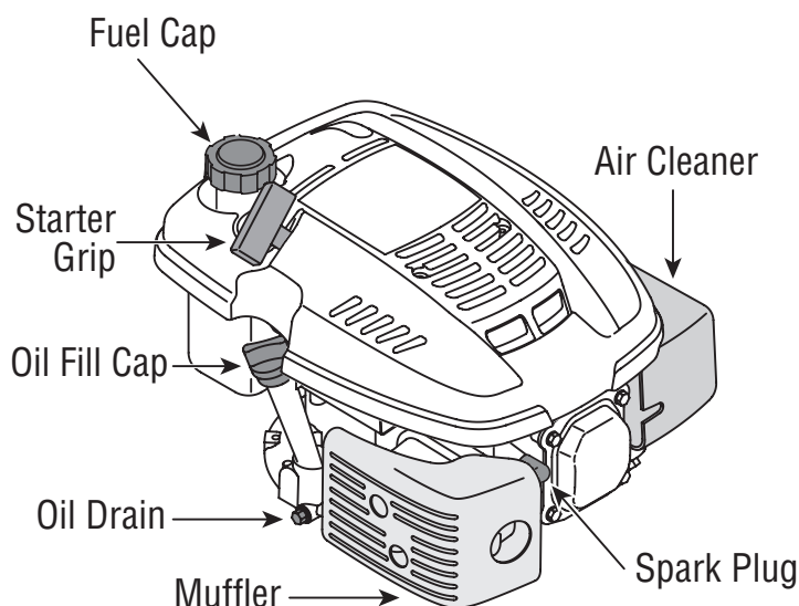
Figure 9-1: The major components of the engine.
