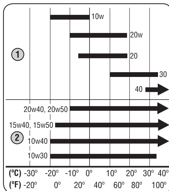
Figure 9-2 Ambient Temperature
