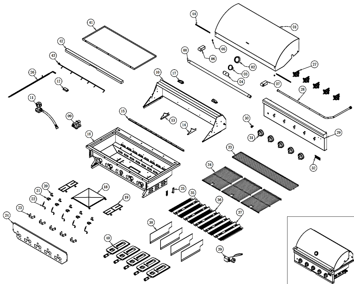
C3CL42 Parts List
