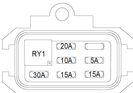
IDENTIFICATION DECAL – MXZ WITH ELECTRIC STARTER
