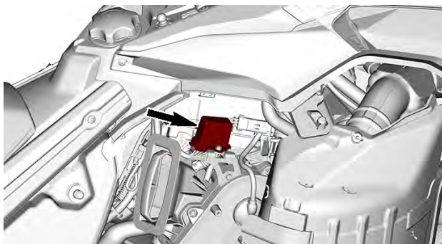
FUSE BOX 1 (FB1) – E-TEC ENGINES 400 MM (16 IN)
