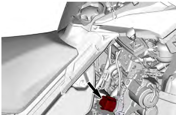
FUSE BOX 1 (FB1) – E-TEC ENGINES 500 MM (20 IN)
